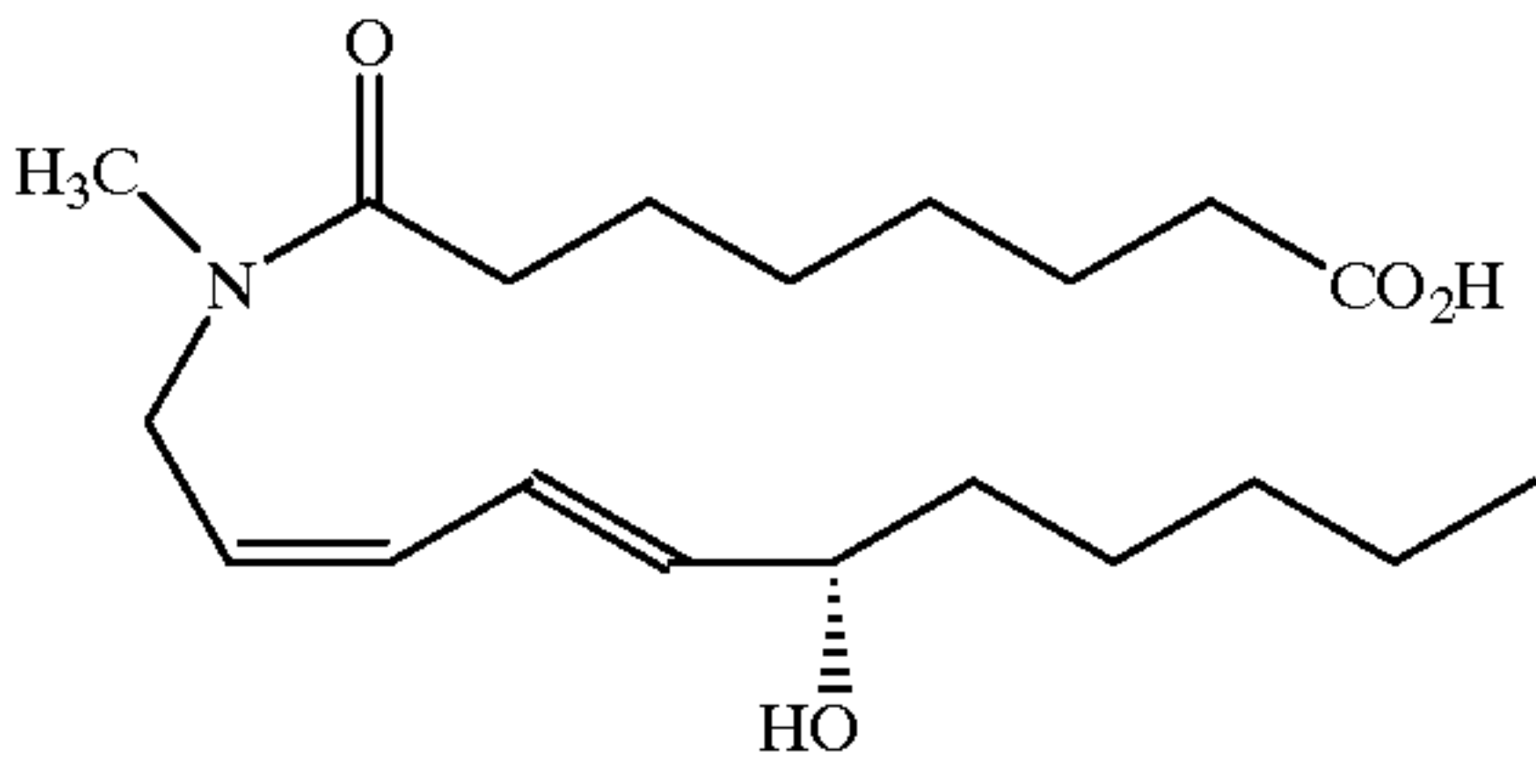
(15S)-(11Z,13E)-9-aza-15-hydroxy-9-methyl-8-oxo-11,13-eicosadienoic acid
