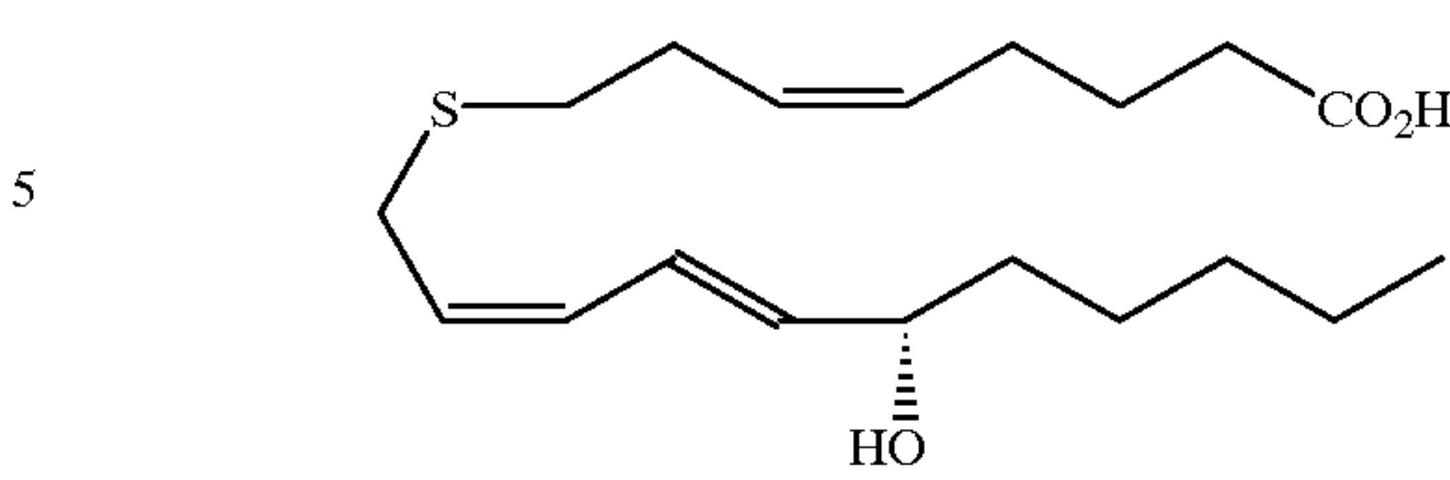
(15S)-(5Z,11Z,13E)-15-hydroxy-9-thia-5,11,13-eicosatrienoic acid
