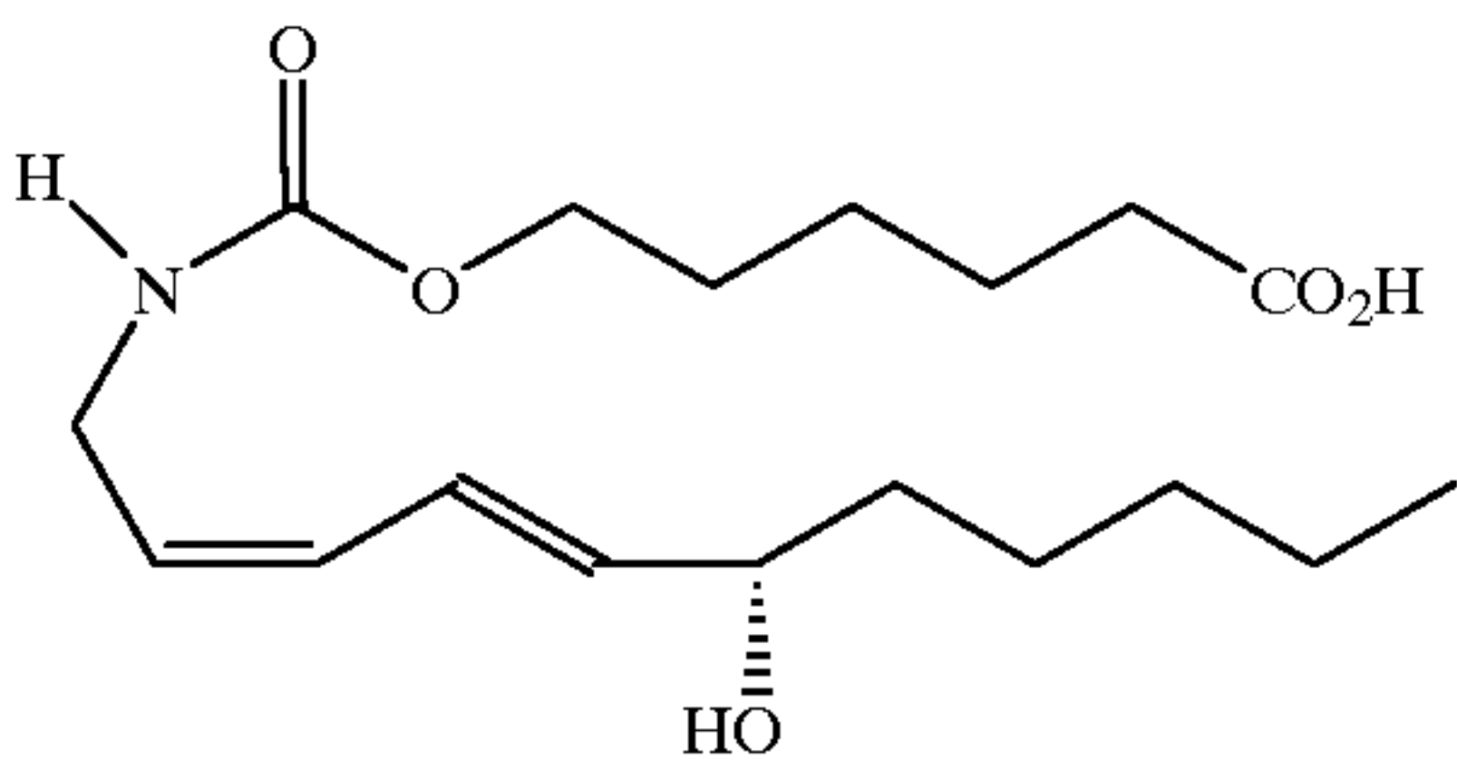
(15S)-(11Z,13E)-9-aza-15-hydroxy-7-oxa-8-oxo-11,13-eicosadienoic acid
