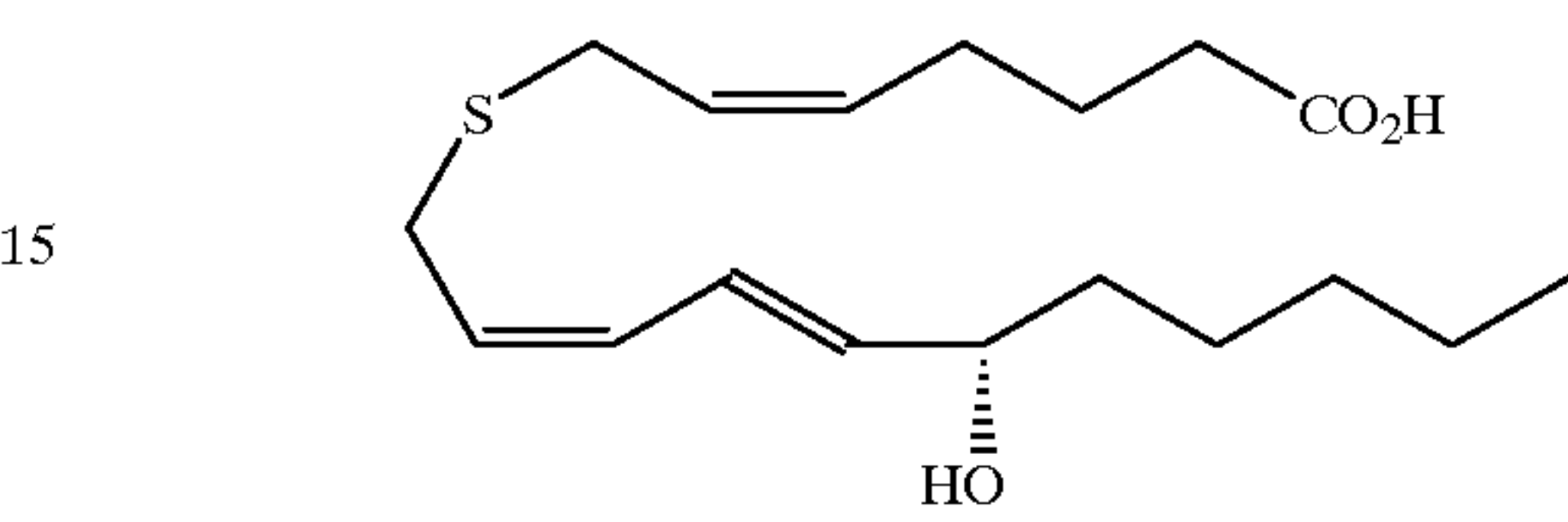
(14S)-(5Z,10Z,12E)-14-hydroxy-8-thia-5,10,12-nonadecatrienoic acid
