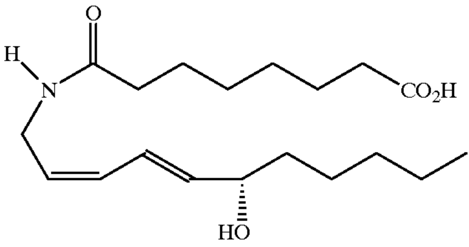
(15S)-(11Z,13E)-9-aza-15-hydroxy-8-oxo-11,13-eicosadienoic acid
