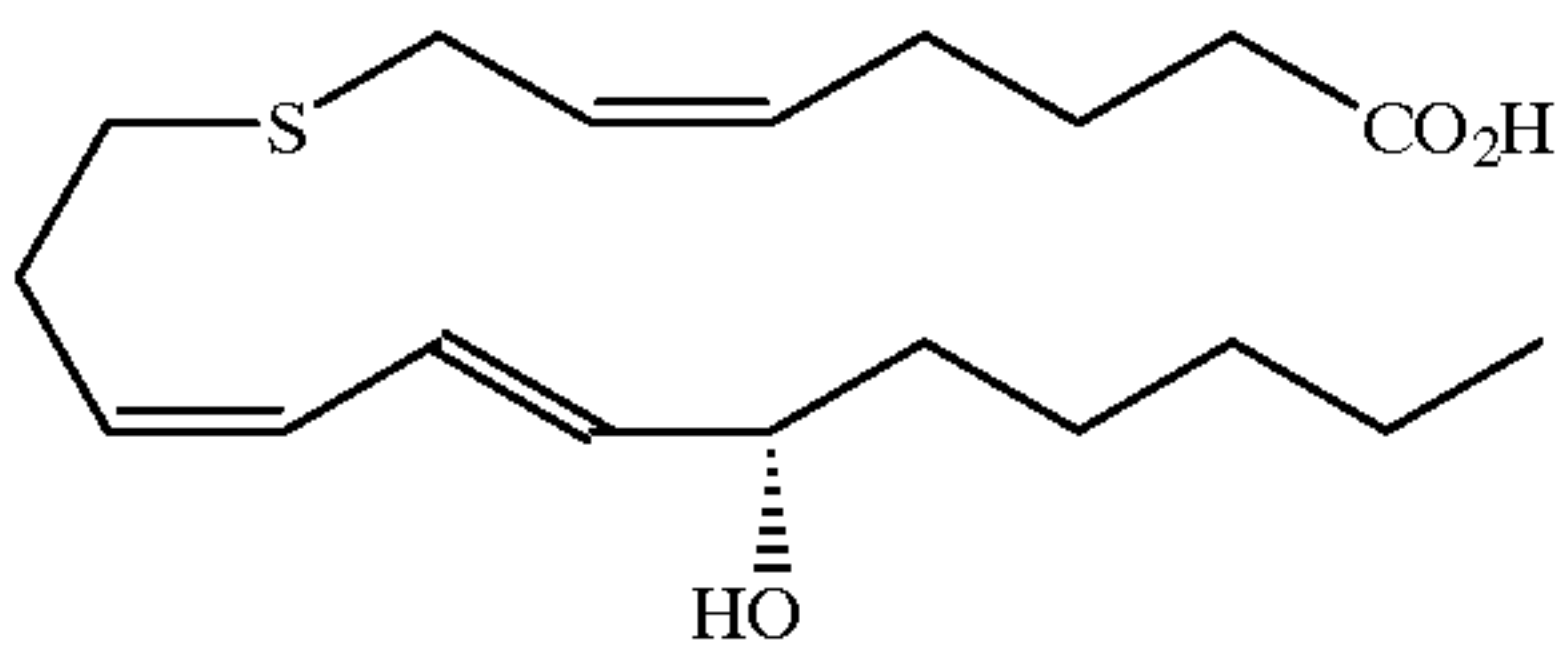
(15S)-(5Z,11Z,13E)-15-hydroxy-8-thia-5,11,13-eicosatrienoic acid
