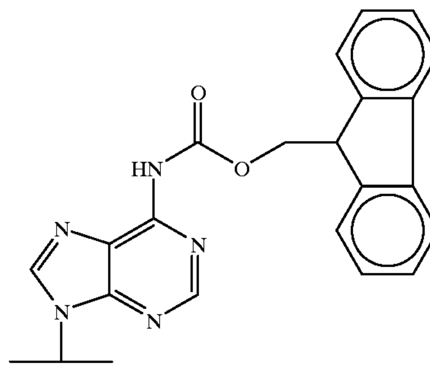
Adenine (A)
