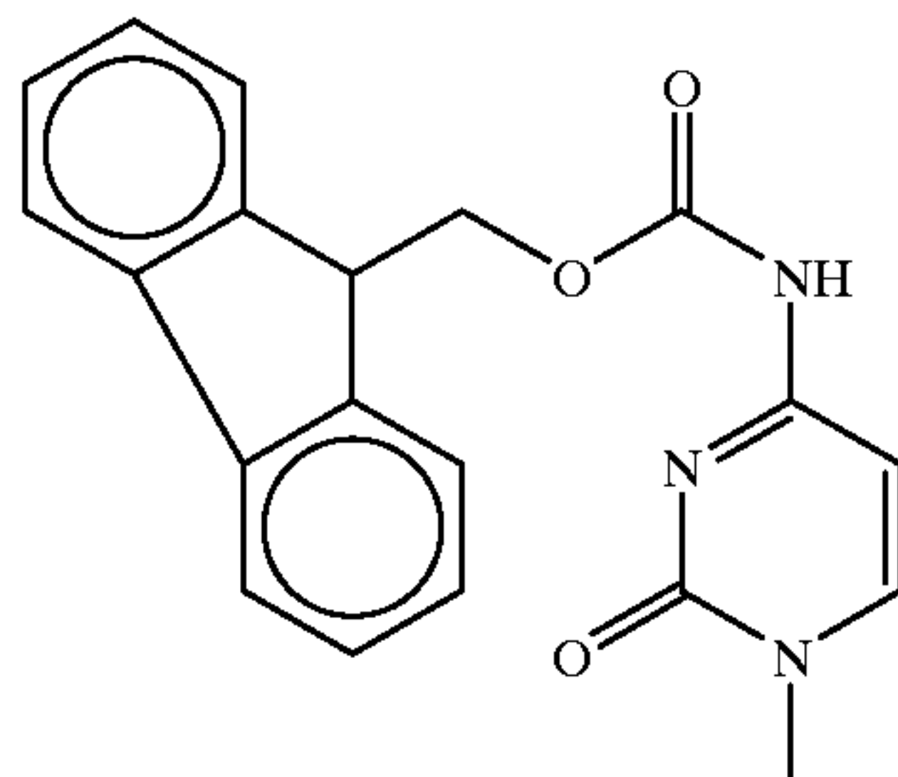
Cytosine (C)
