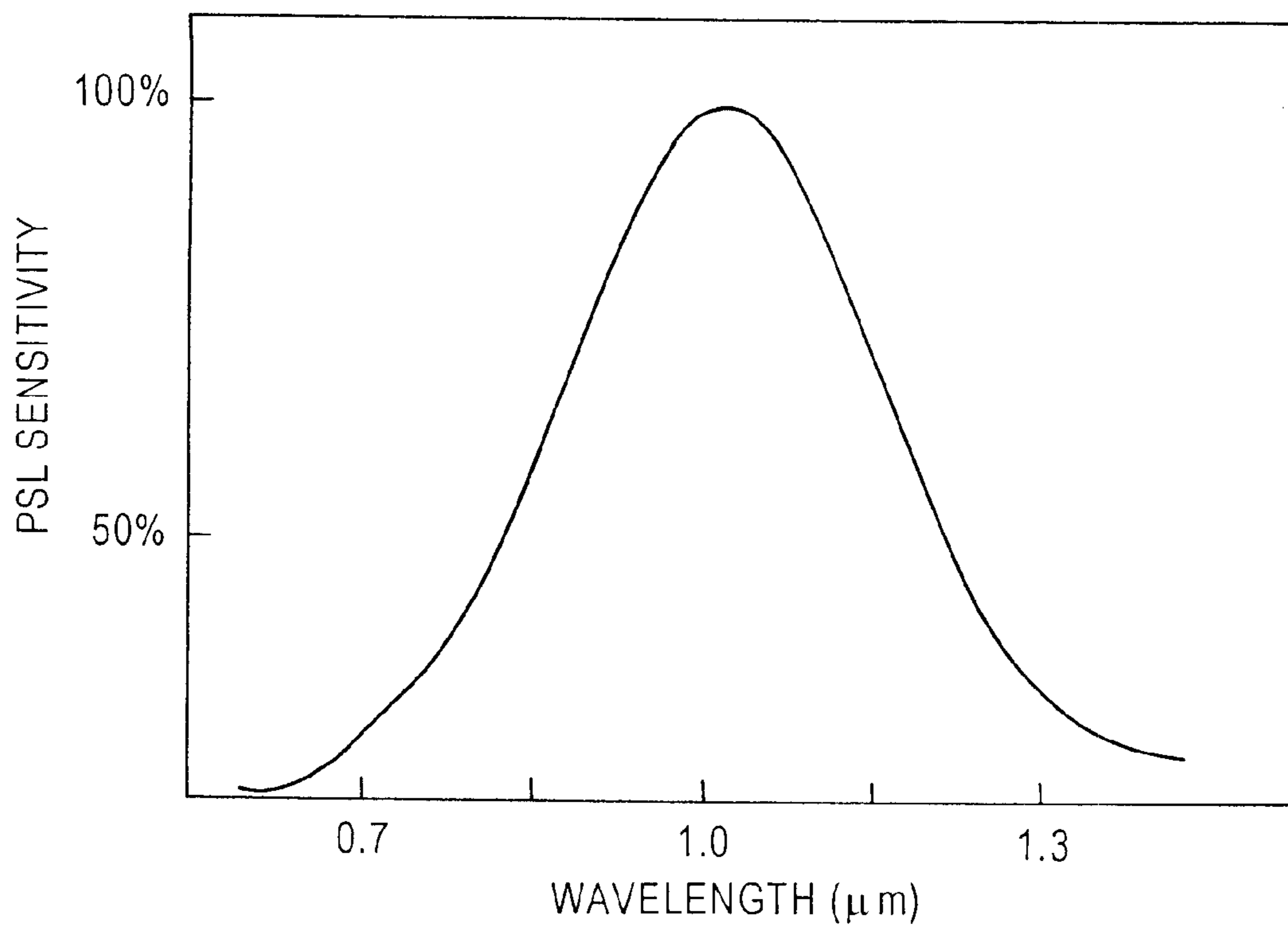
FIG. 5 Prior Art
