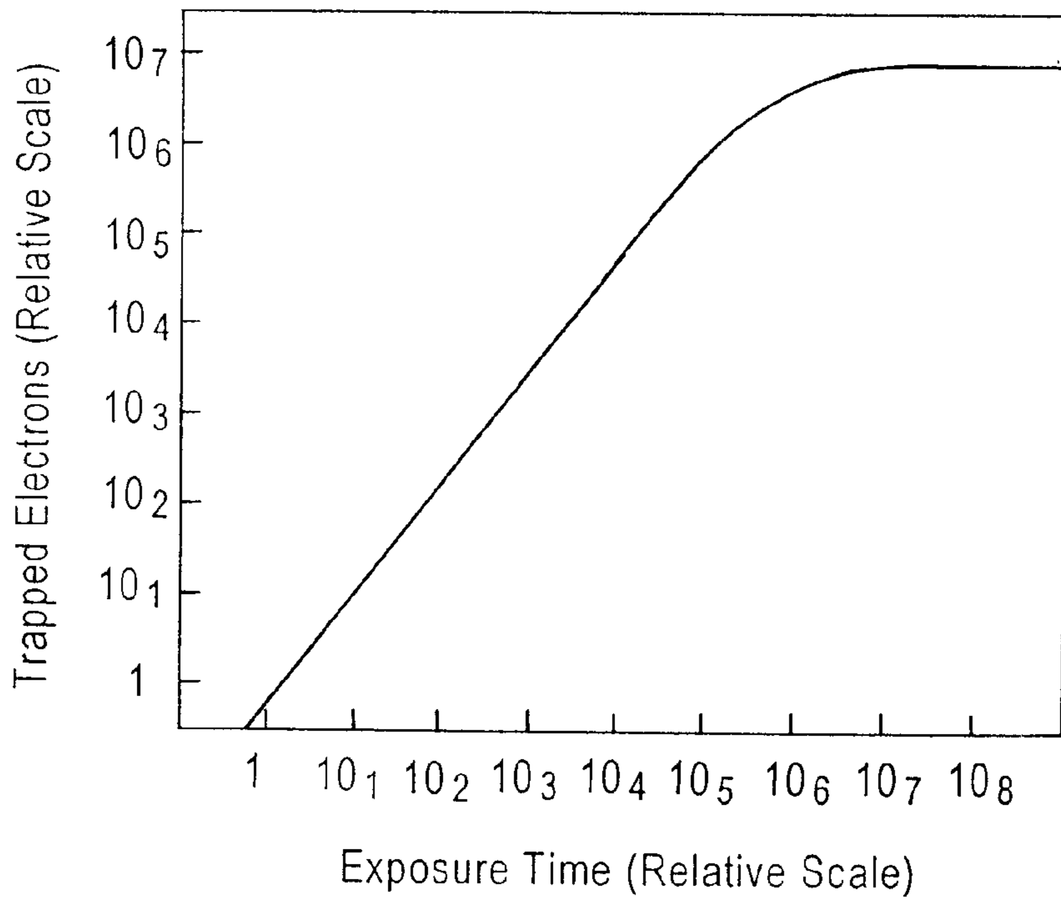
FIG. 6 Prior Art
