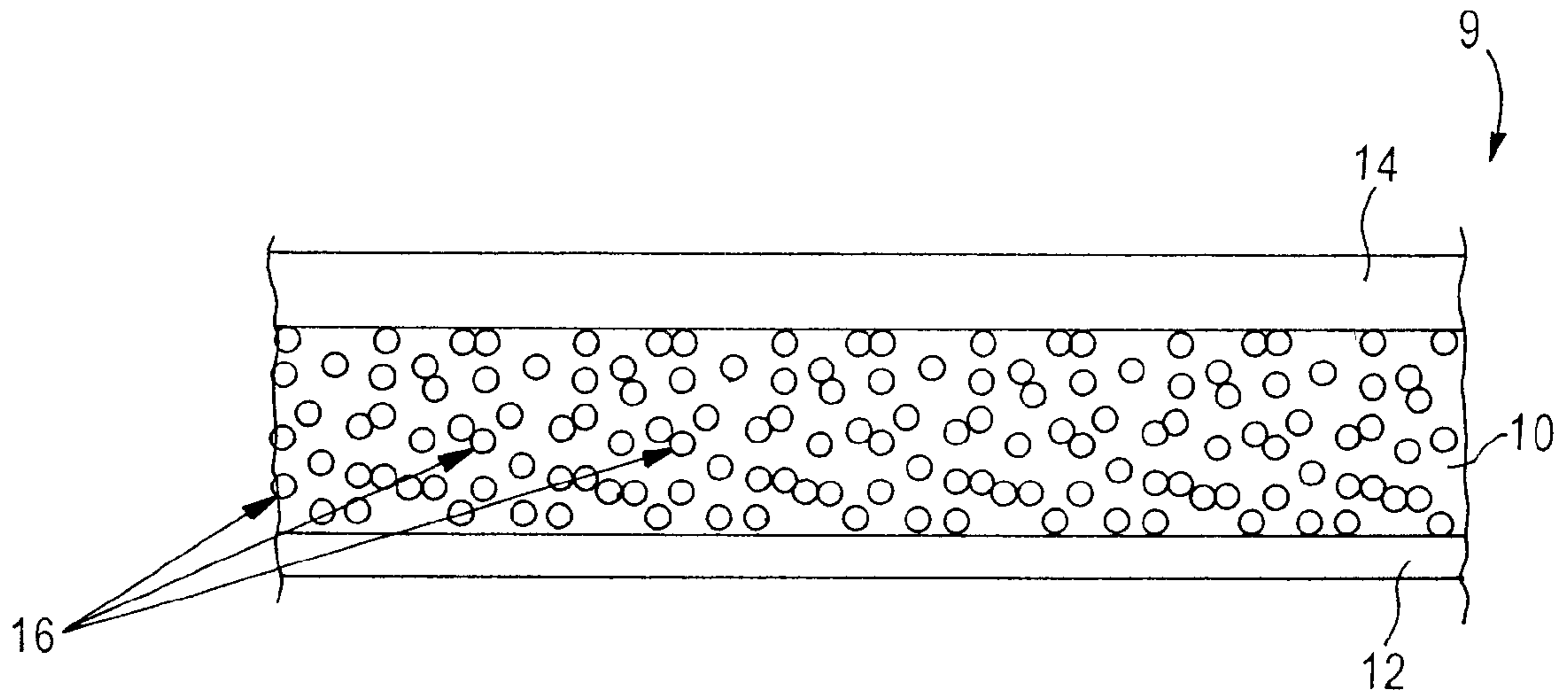
FIG. 1 Prior Art
