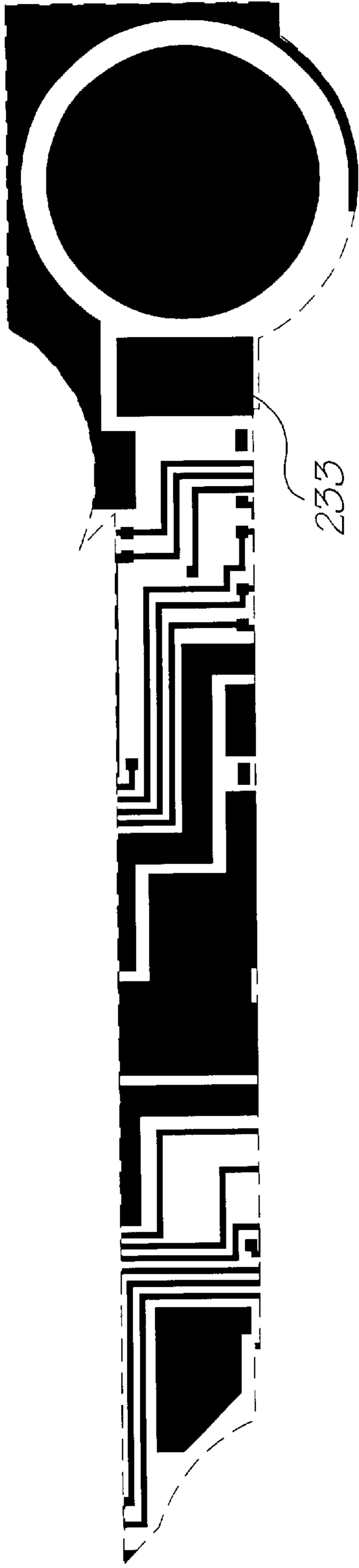
Metal 2 mask
