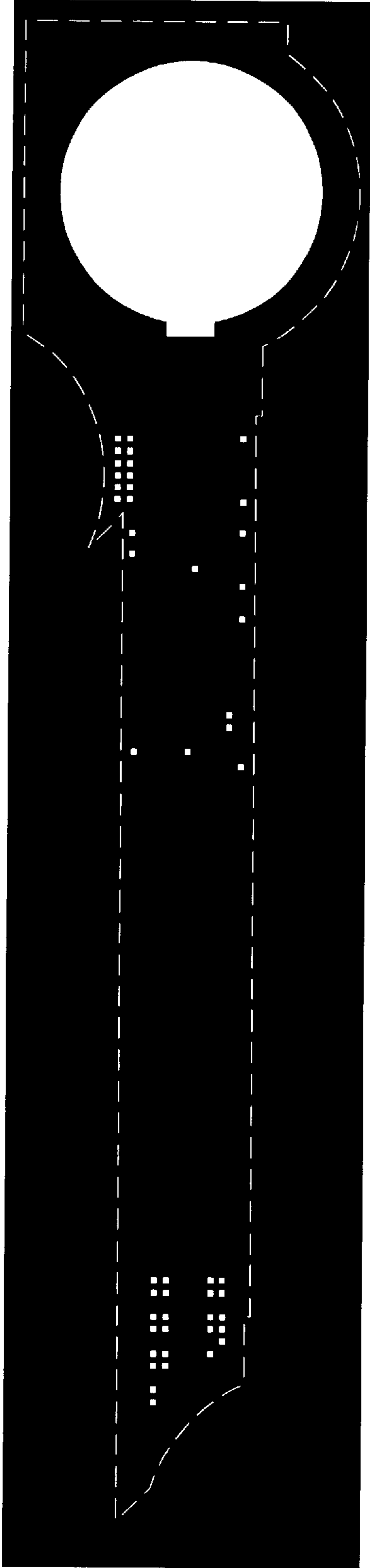
Via 1 mask
