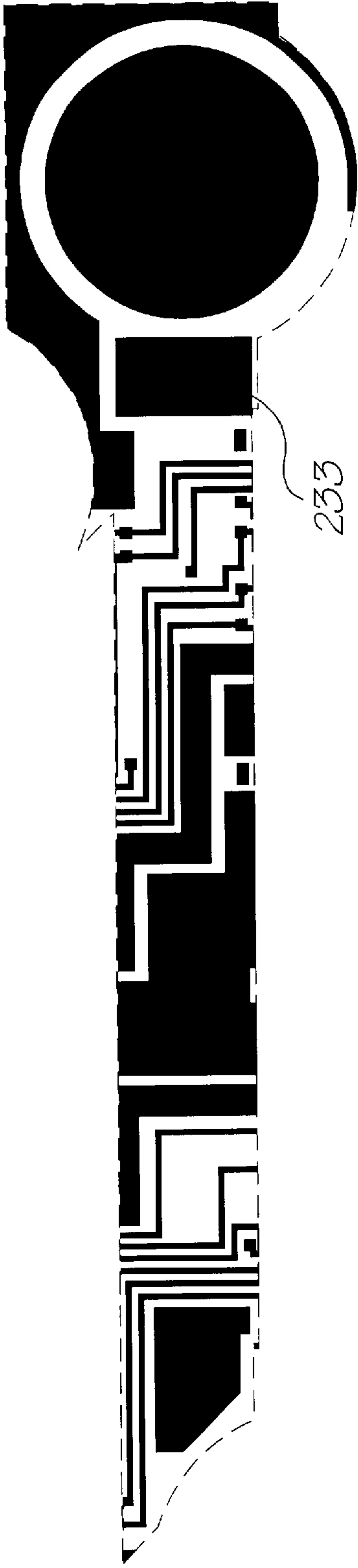
Metal 2 mask
