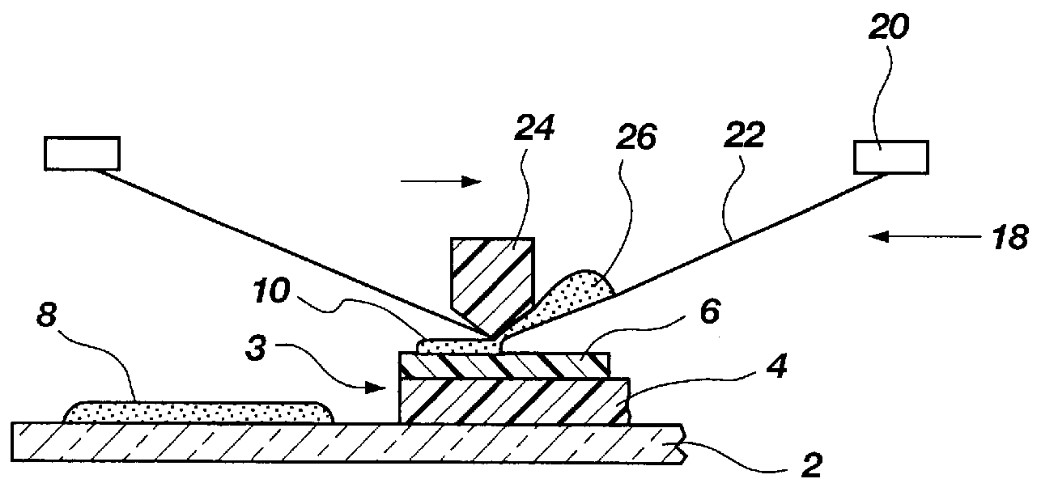
Fig. 1C (PRIOR ART)
