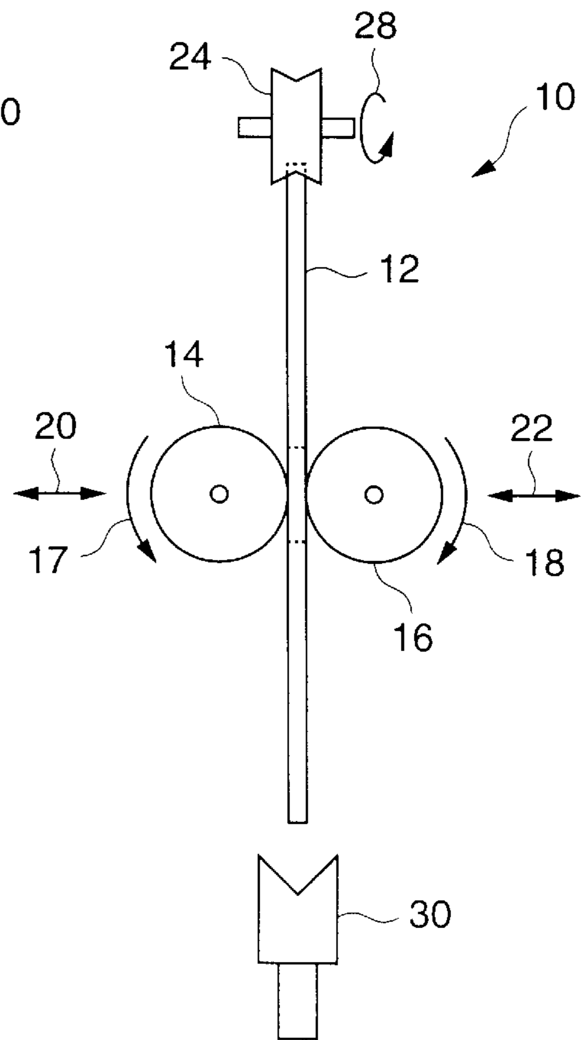
FIG. 2 (PRIOR ART)
