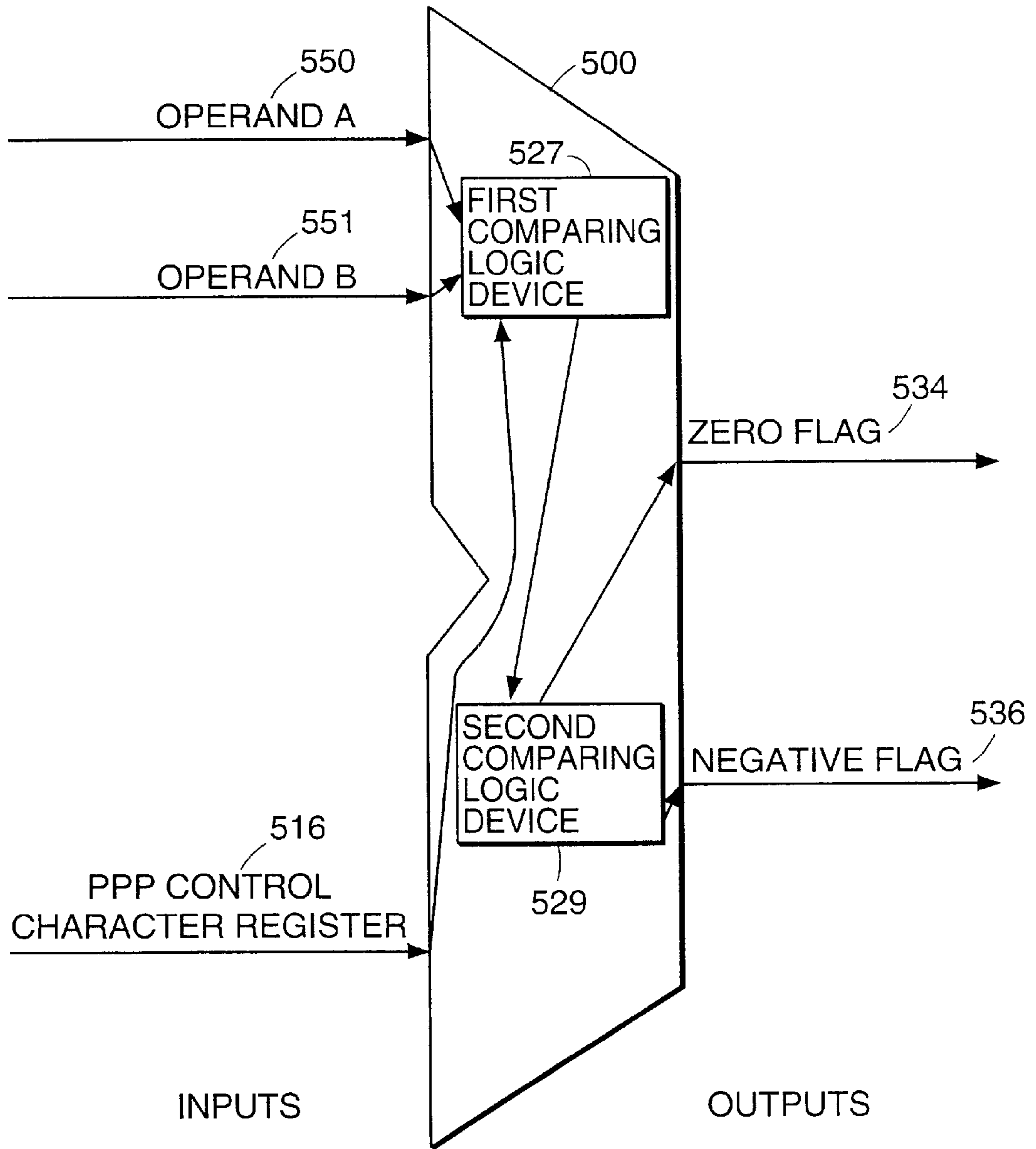
MULTIPLE COMPARE
