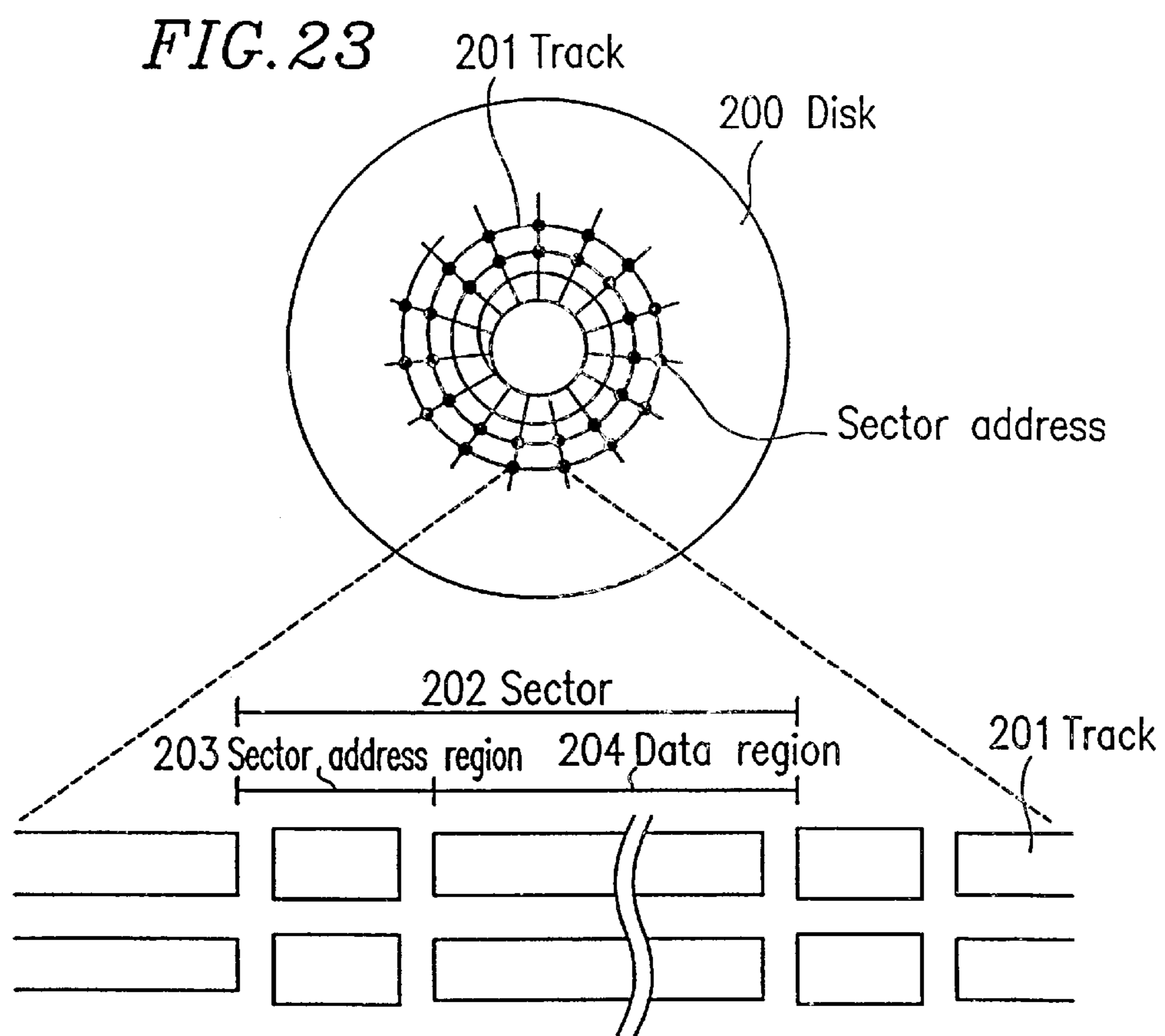
Track structure of a recording/reproduction option disk
