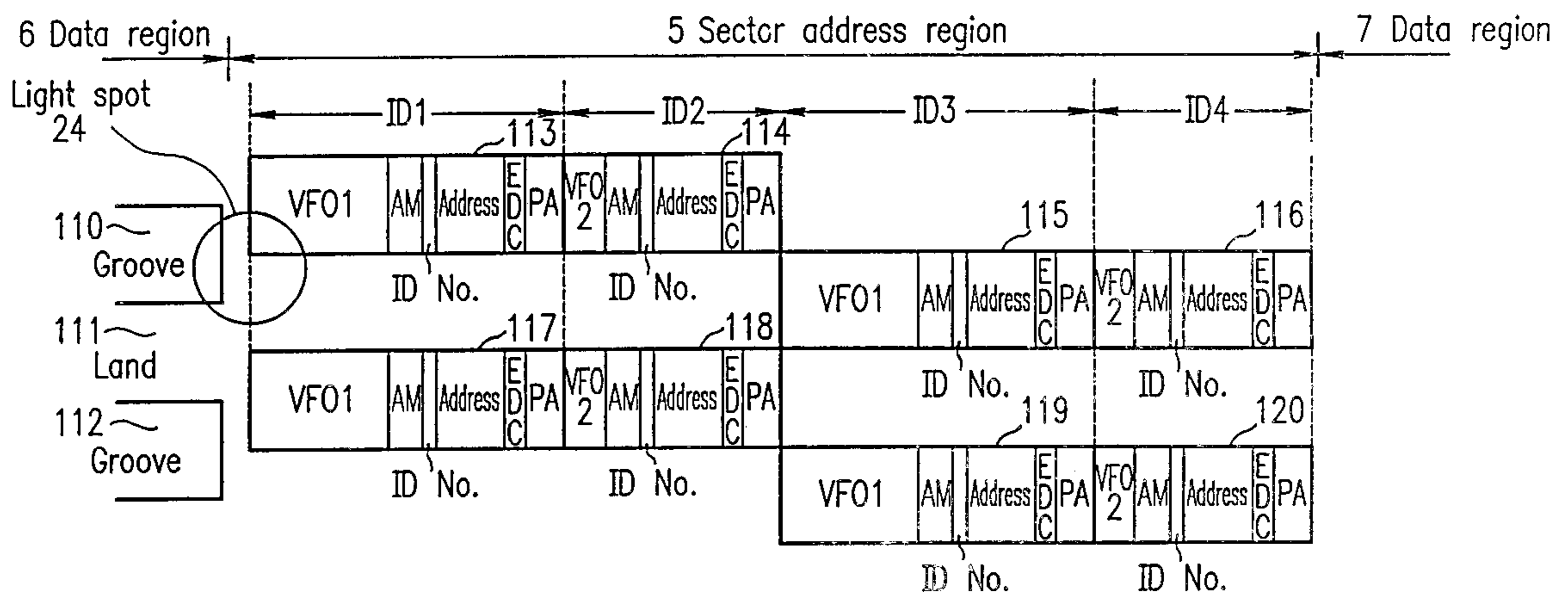
Data arrangement in address blocks
