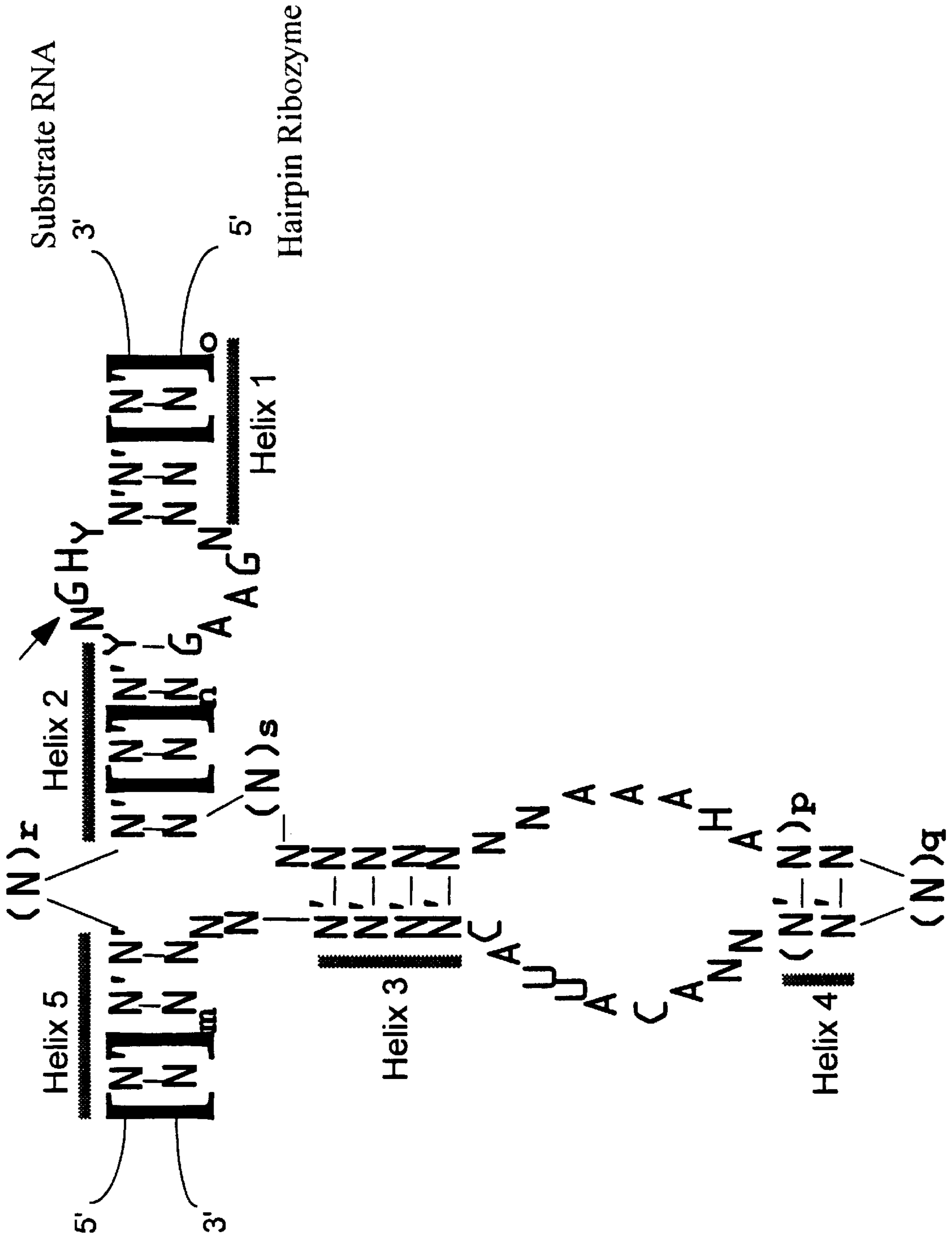
Figure 3: Hairpin Ribozyme
