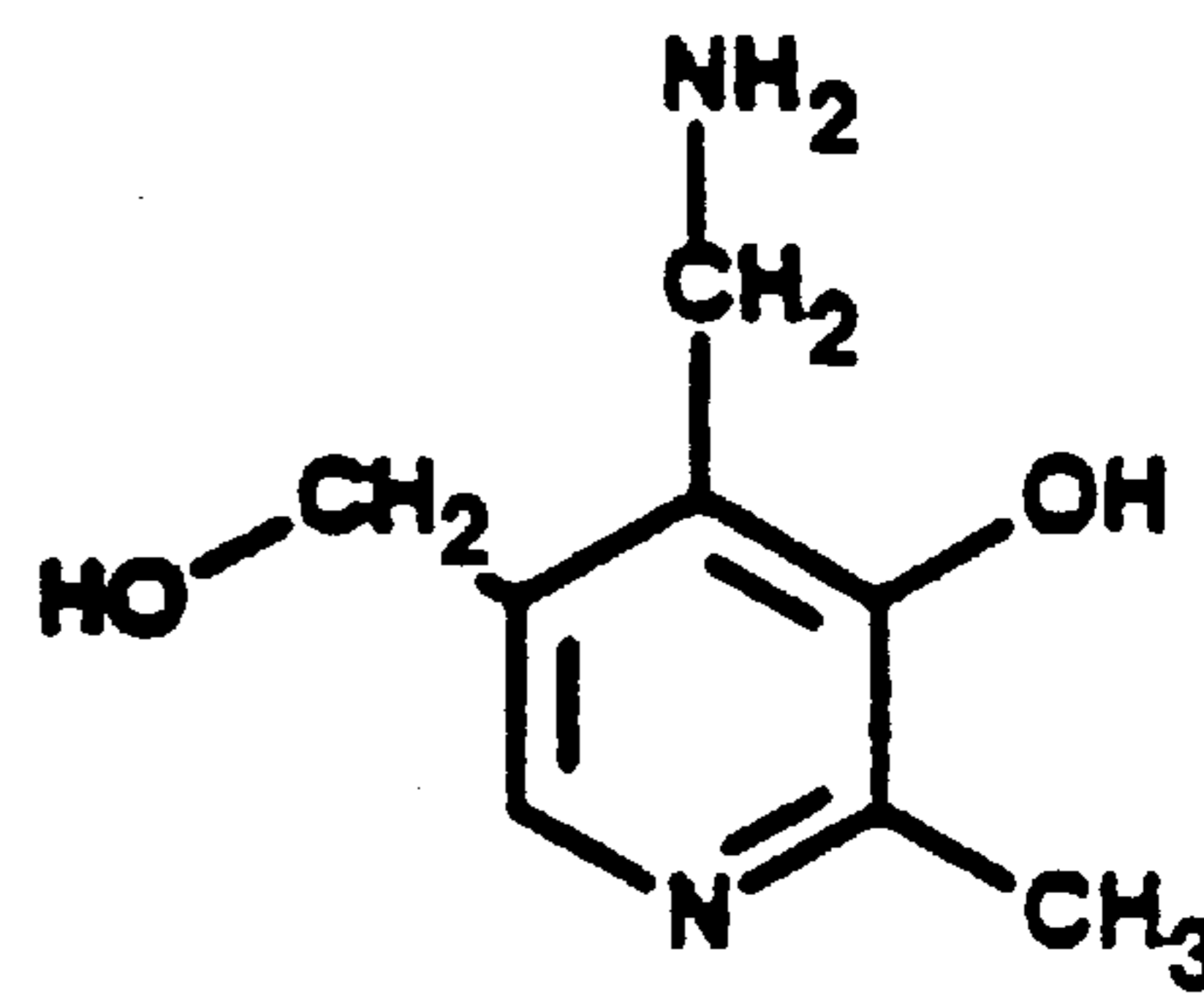
Pyridoxamine
