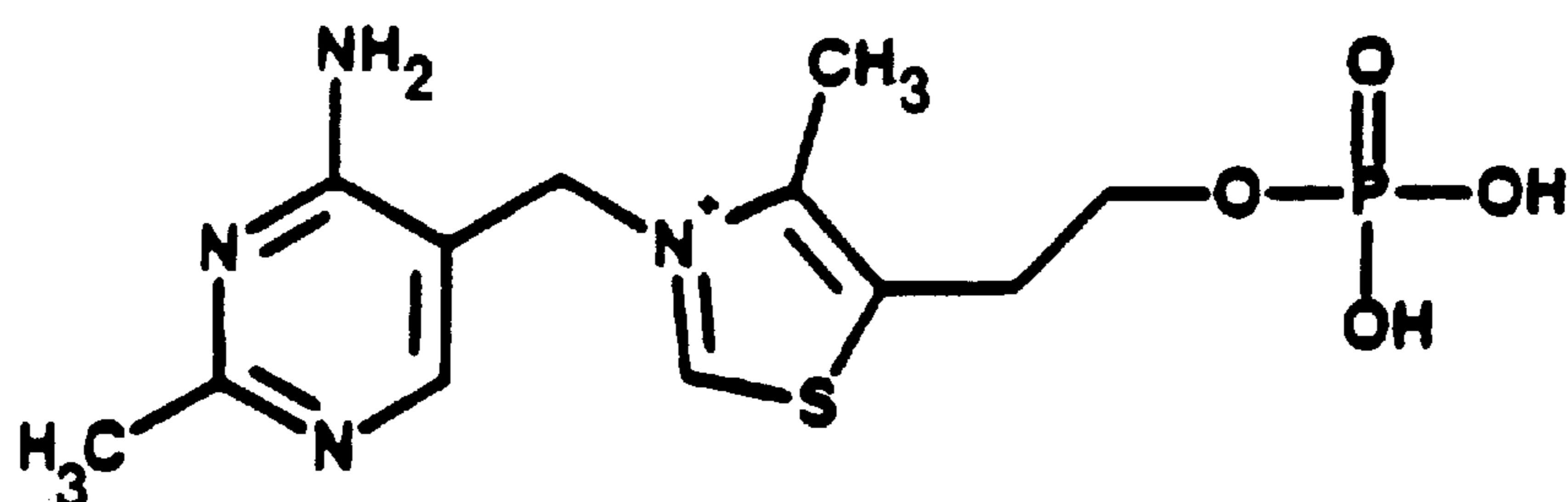
Thiamine-5'-Phosphate
