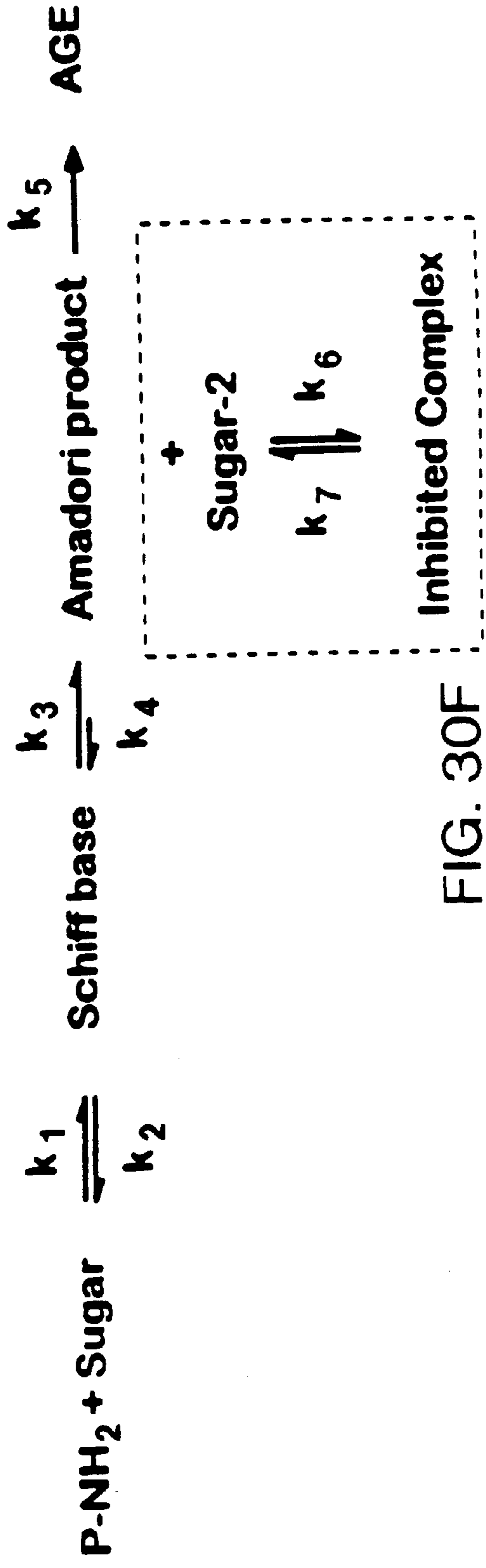
Scheme 6
