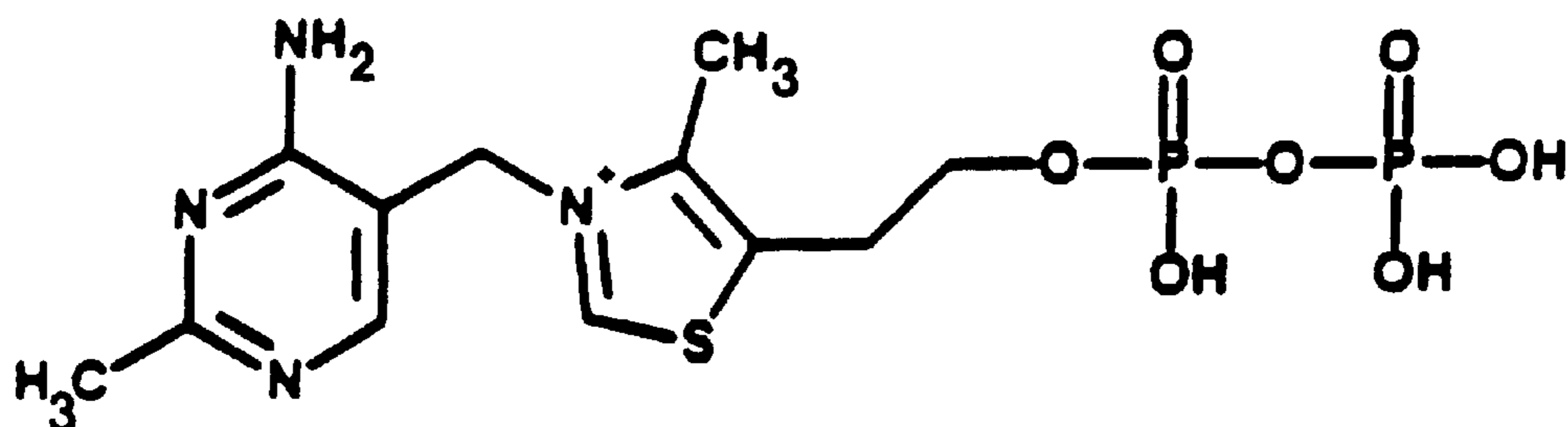
Thiamine Pyrophosphate
