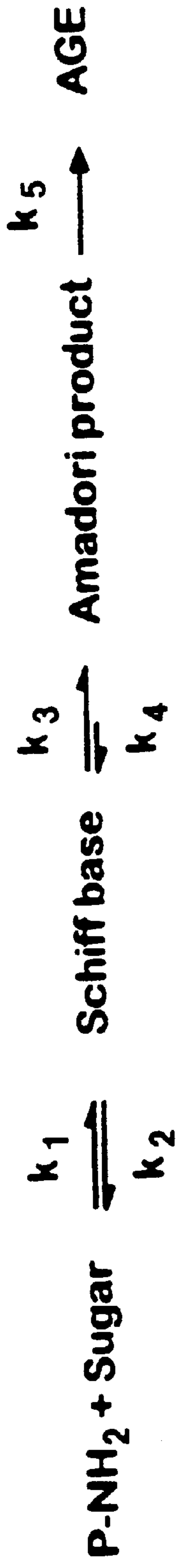
Scheme 5
