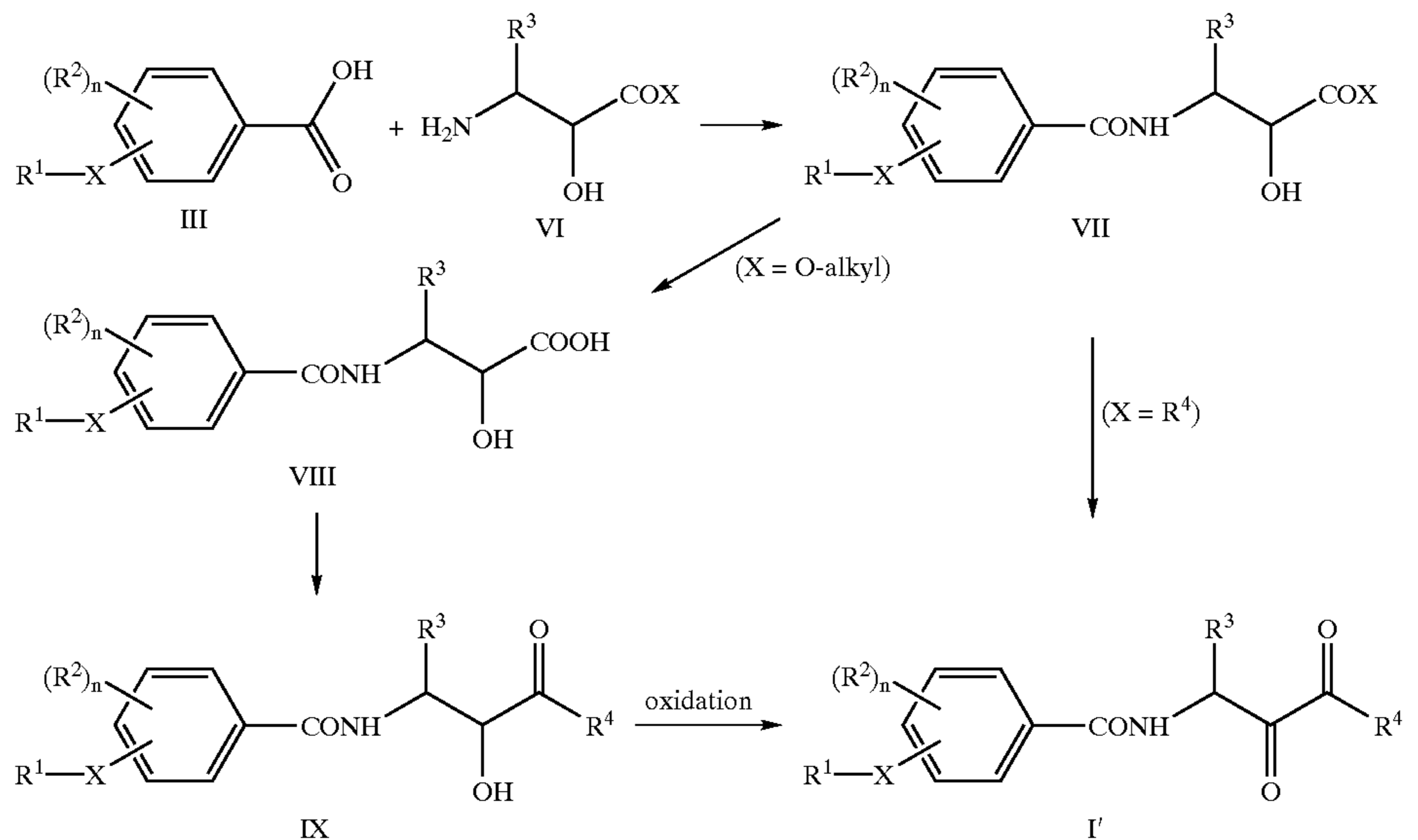
Scheme 2
