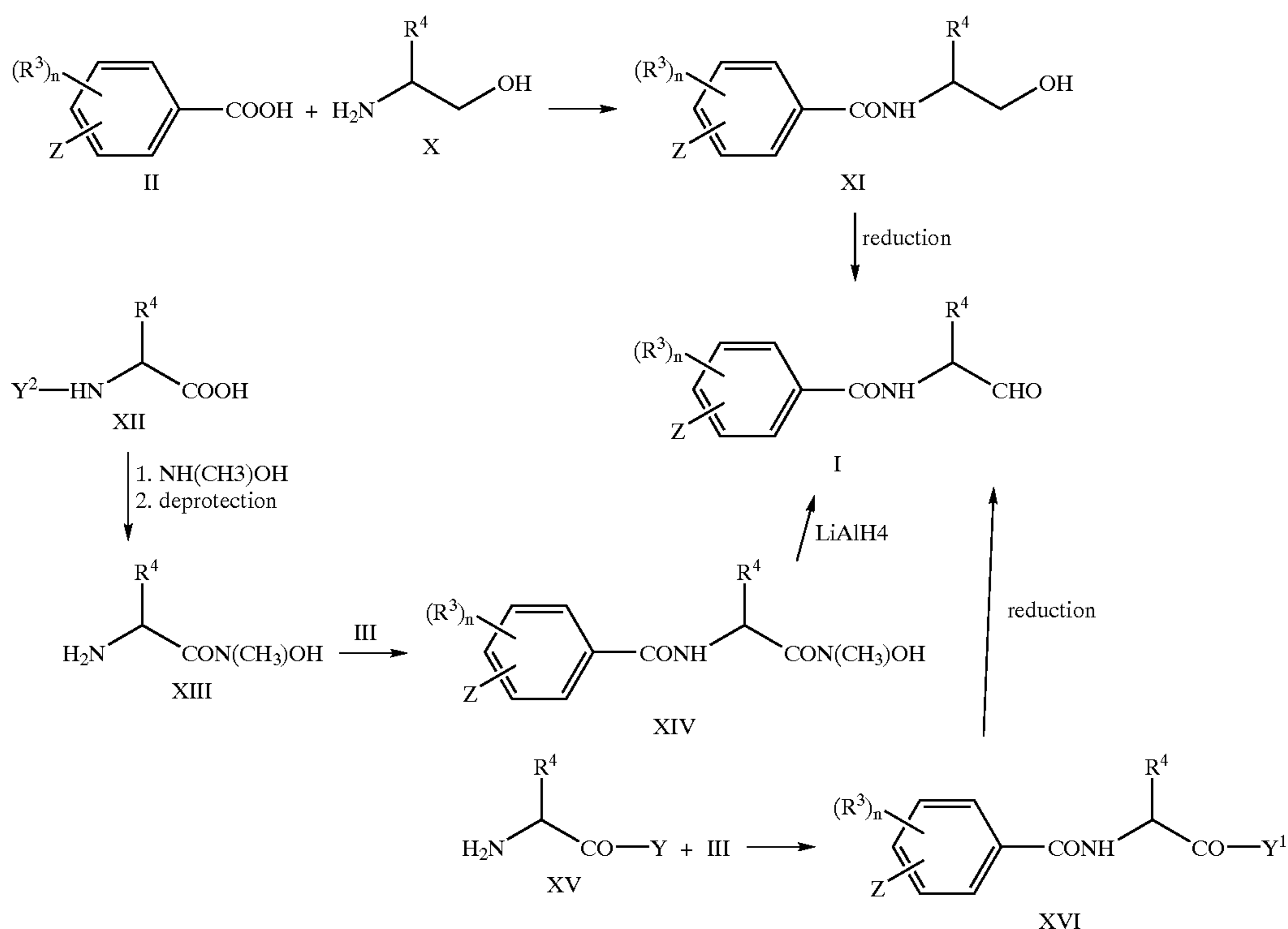
Synthesis scheme 3
