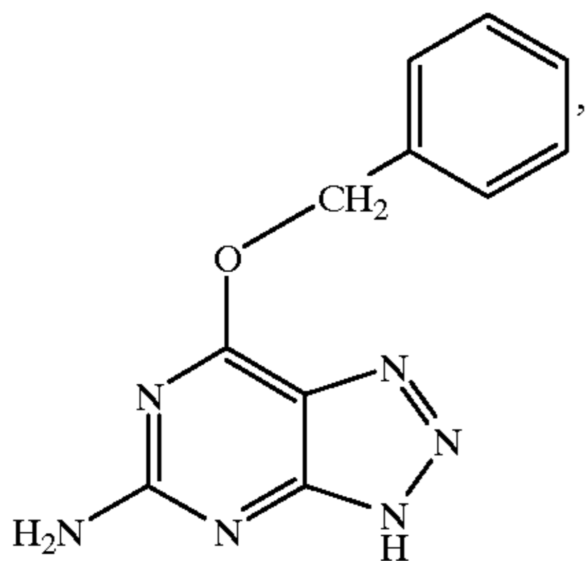
(a) 8-aza- O^6 -benzylguanine
