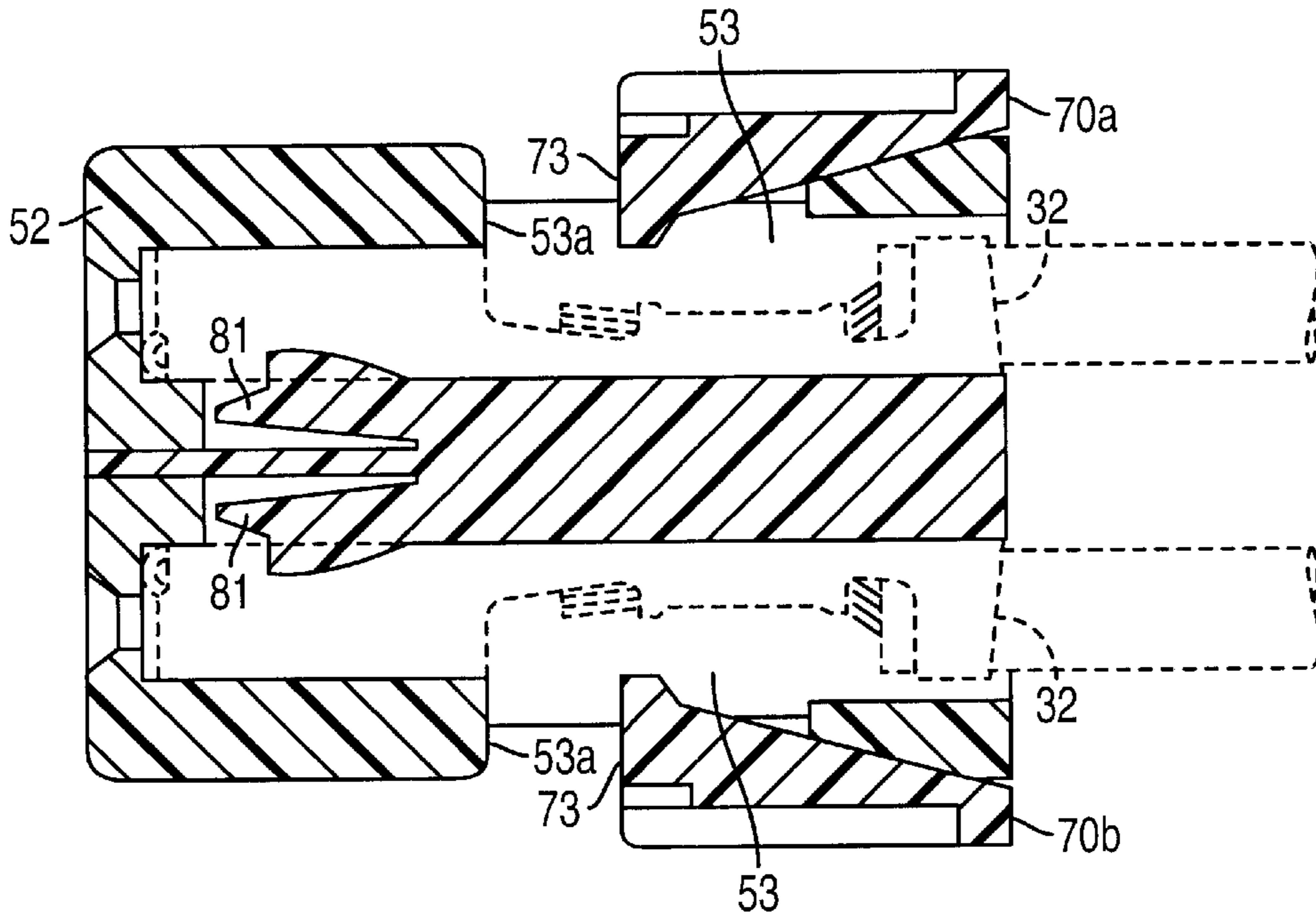
FIG. 17 PRIOR ART
