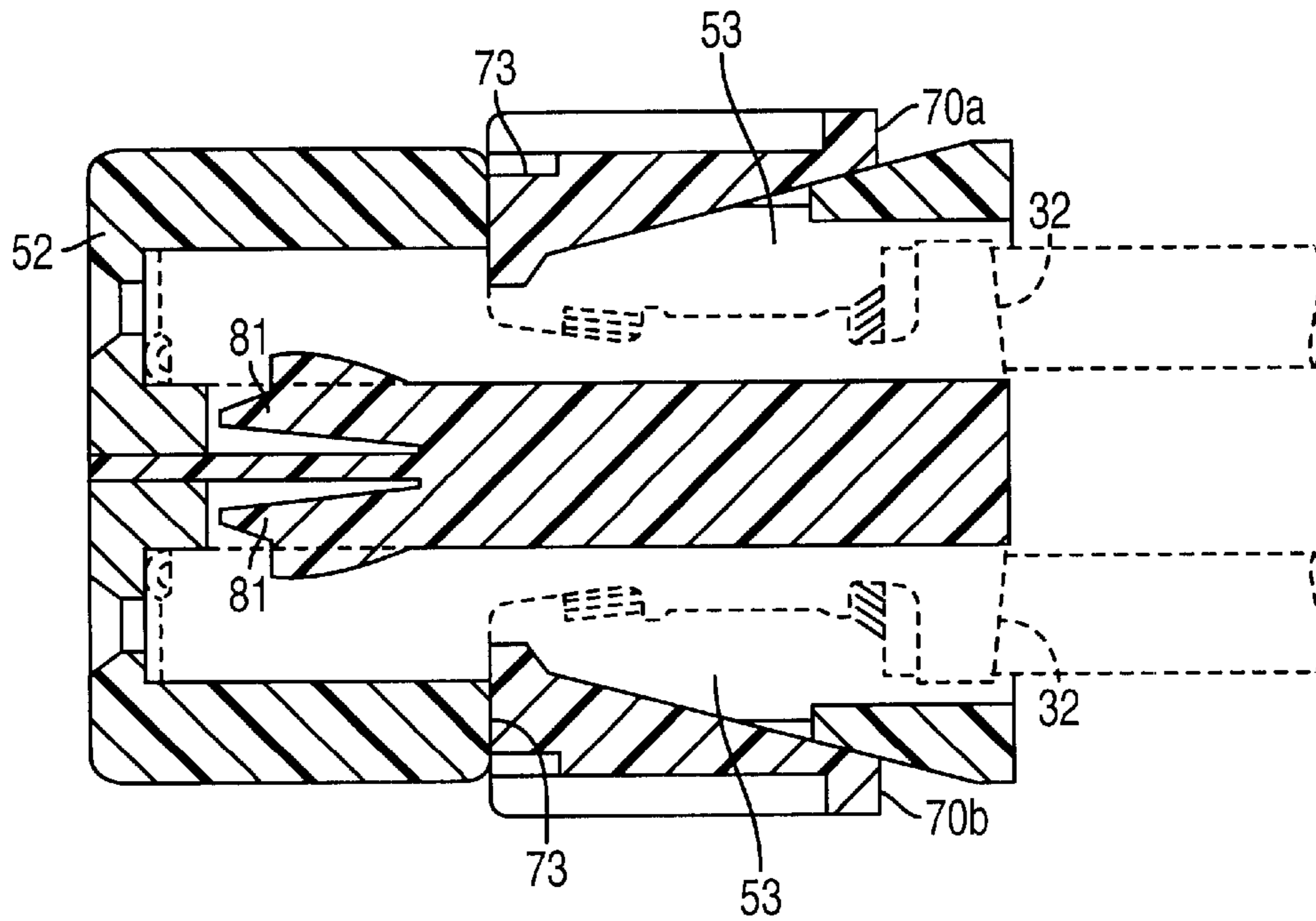
FIG. 18 PRIOR ART
