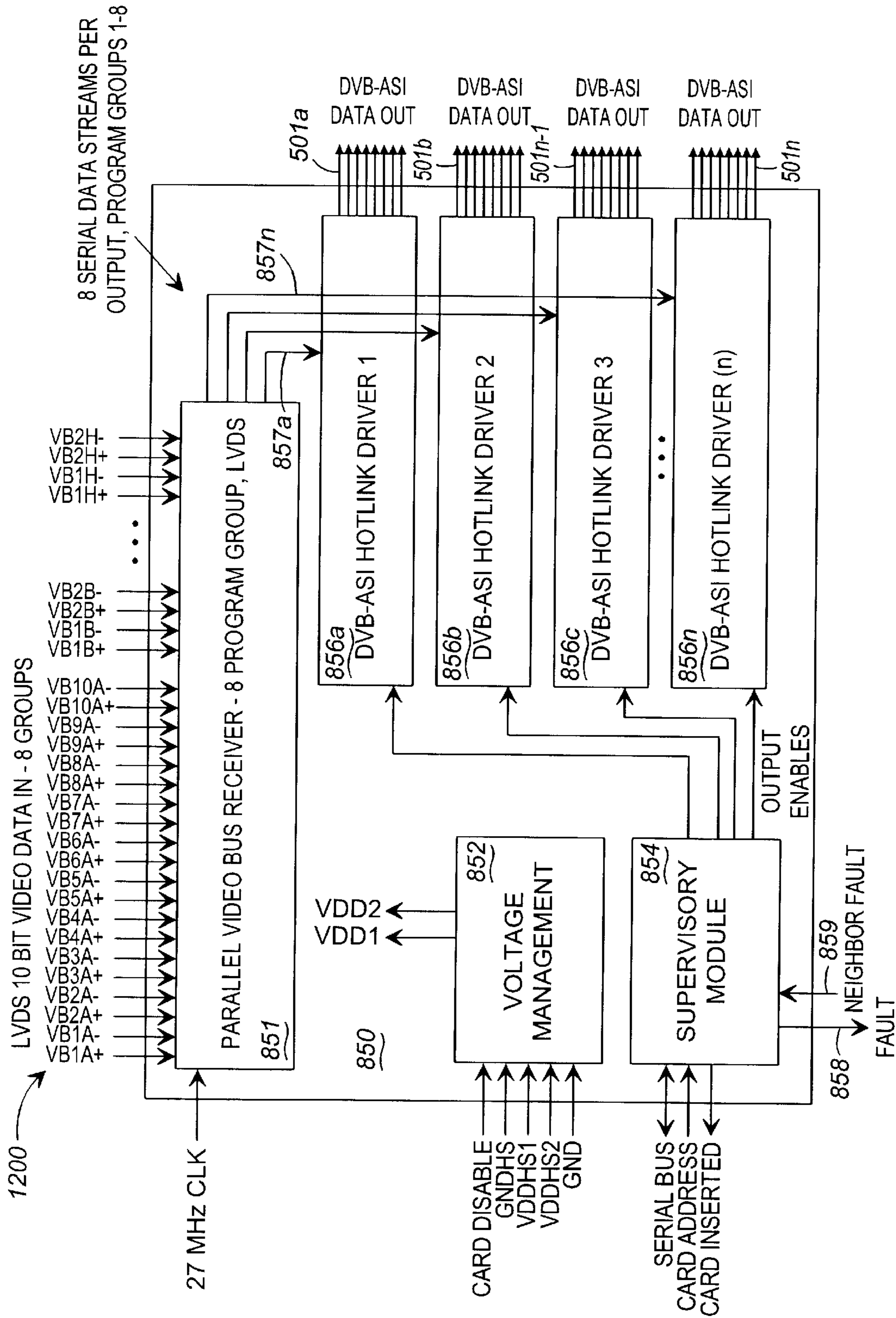
FIG. 11D MULTIPLE VIDEO OUTPUT MODULE BLOCK DIAGRAM
