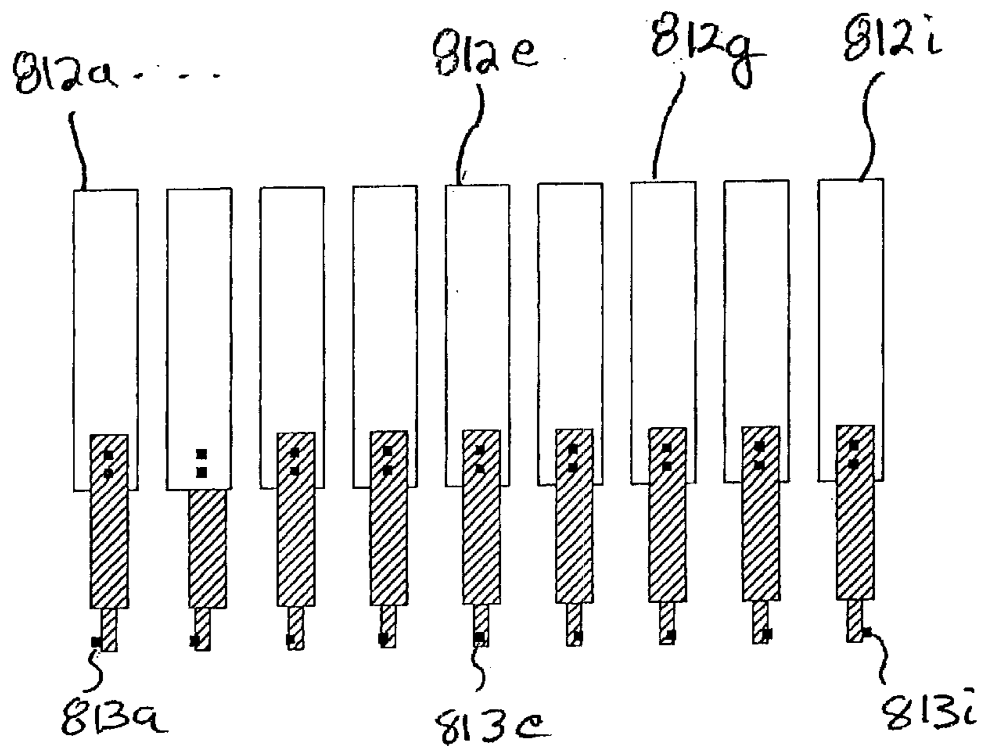
Figure 23B: A portion of the M1 to Contact, X component, Overlay Structure
