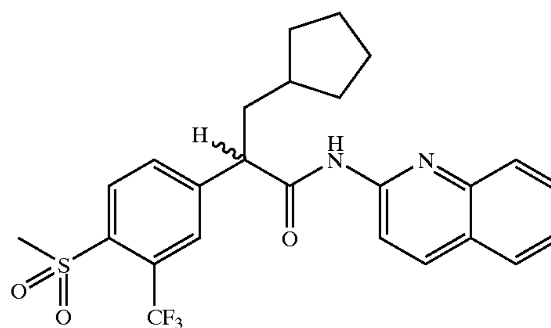
3-Cyclopentyl-2-(4-methanesulfonyl-3-trifluoromethyl-phenyl)-N-quinolin-2-yl-propionamide
