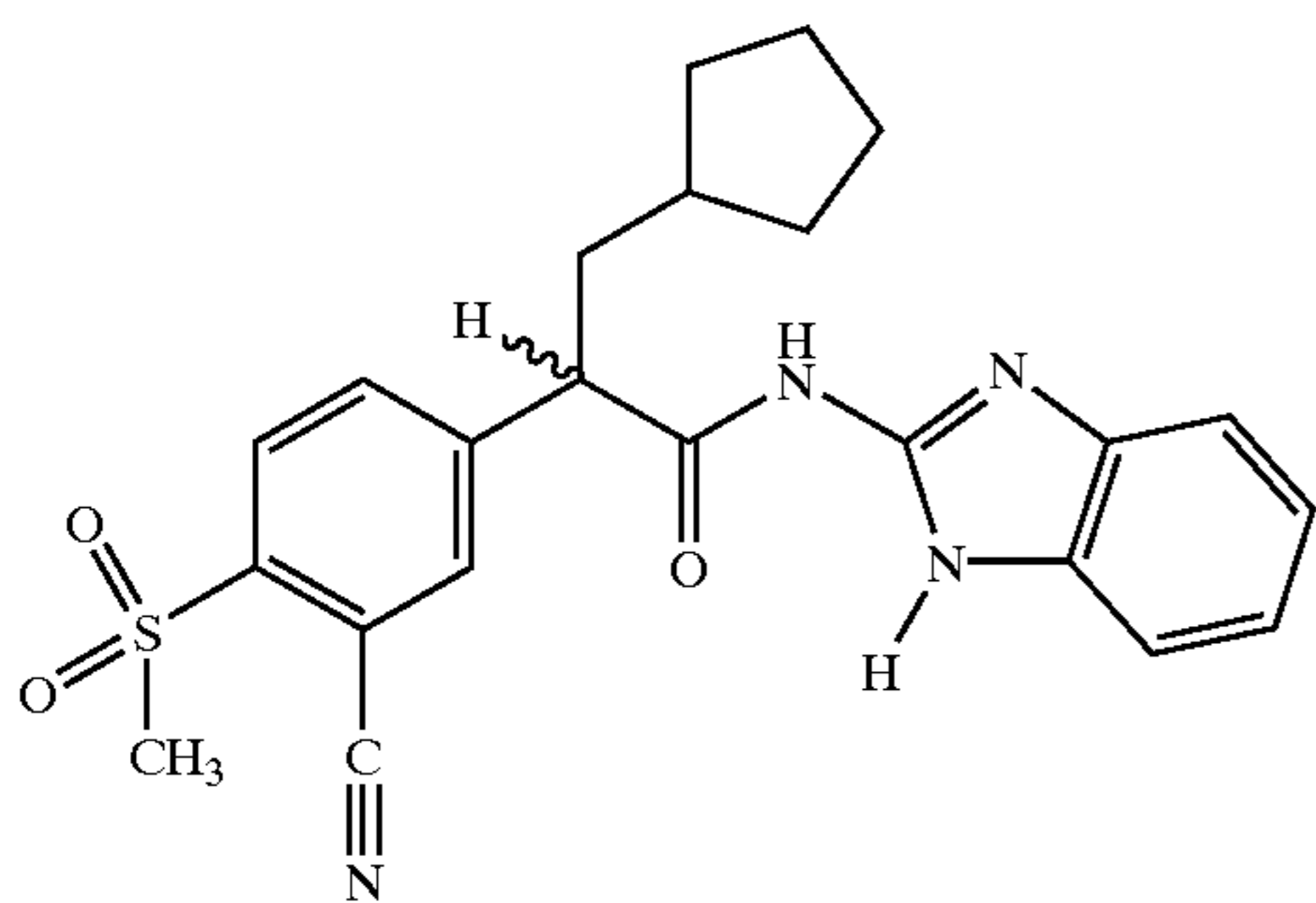
N-(1H-Benzimidazol-2-yl)-2-(3-cyano-4-methanesulfonyl-phenyl)-3-cyclopentyl-propionamide
