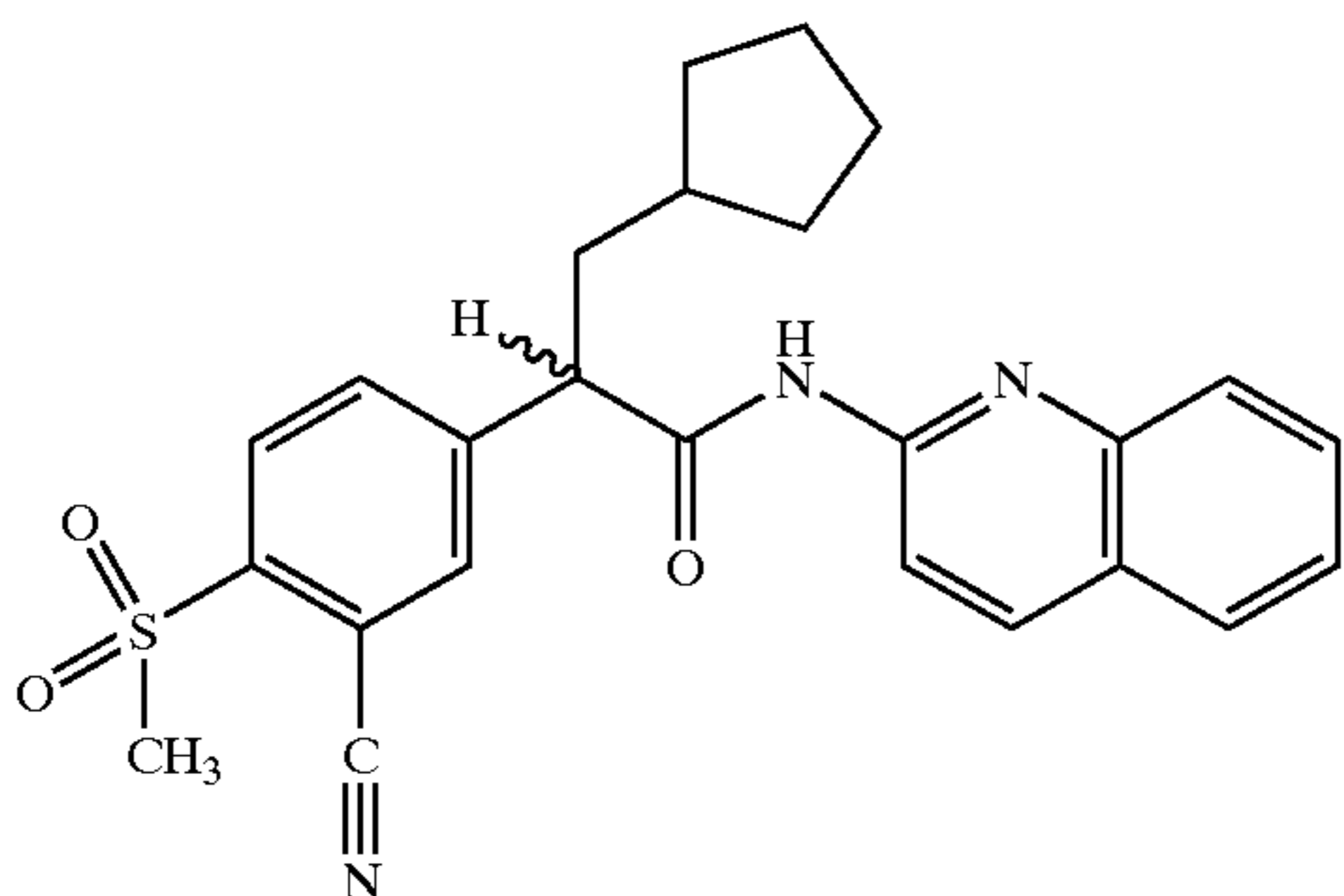
2-(3-Cyano-4-methanesulfonyl-phenyl)-3-cyclopentyl-N-quinolin-2-yl-propionamide
