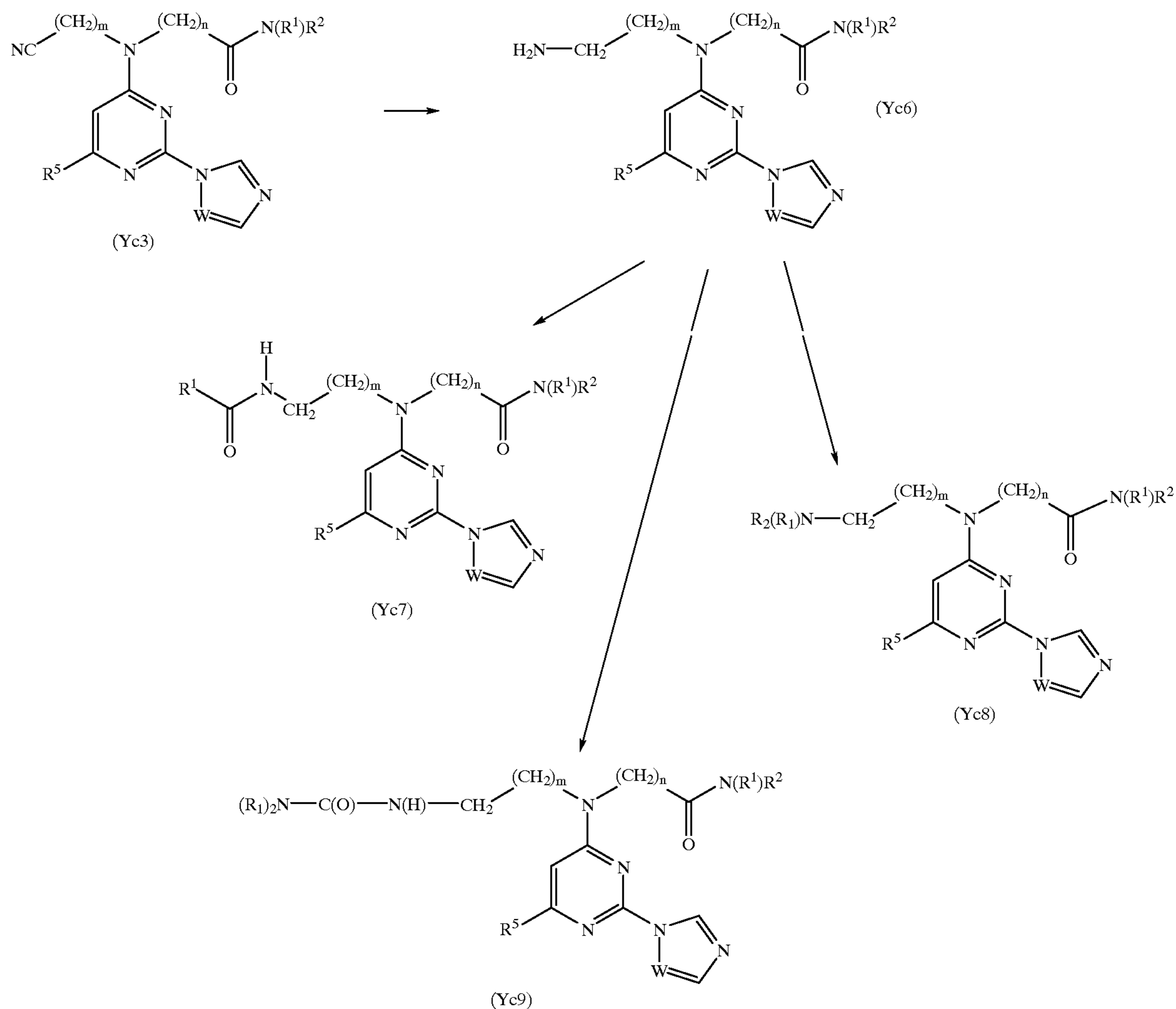
Reaction Scheme 6c
