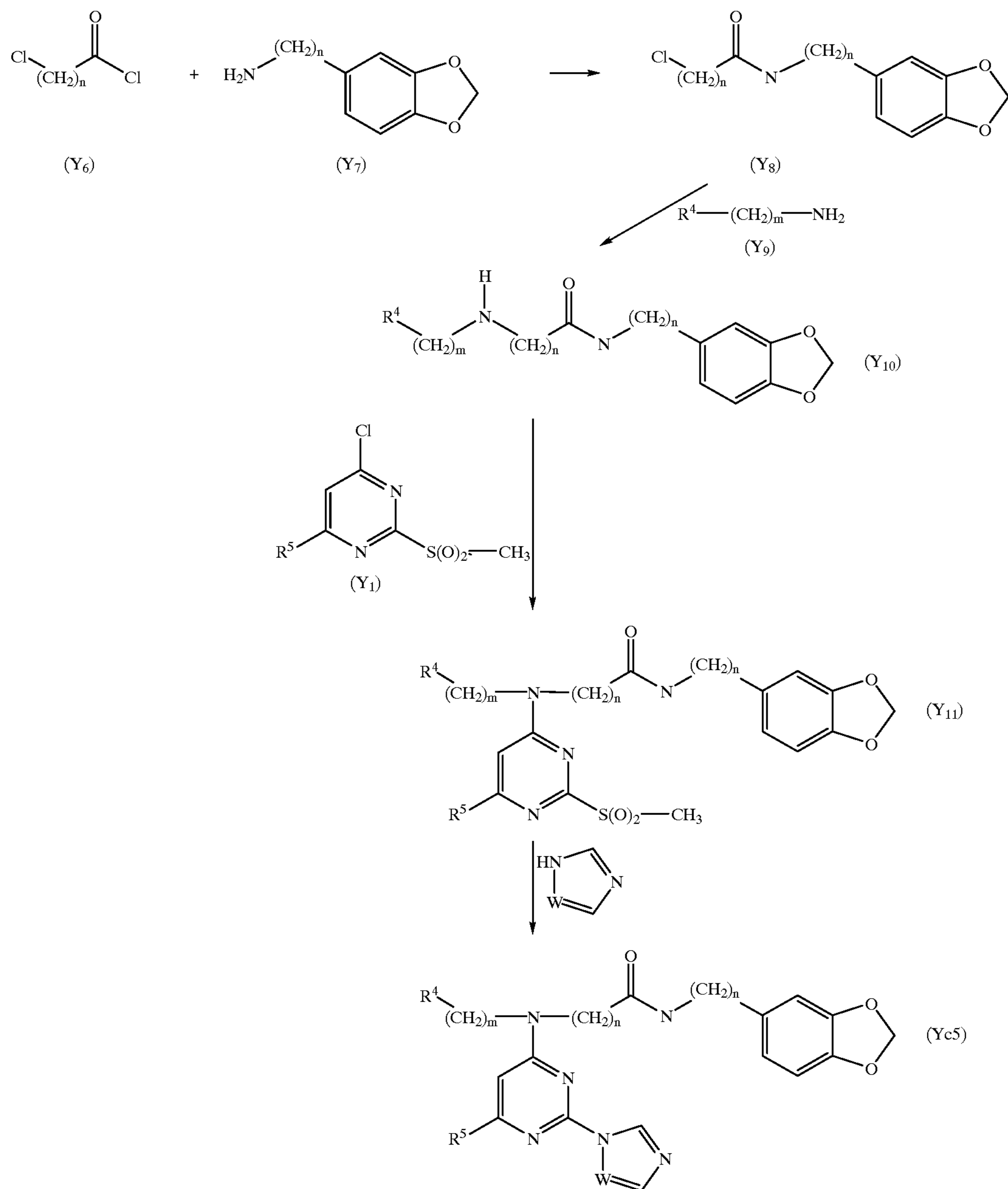
Reaction Scheme 6b
