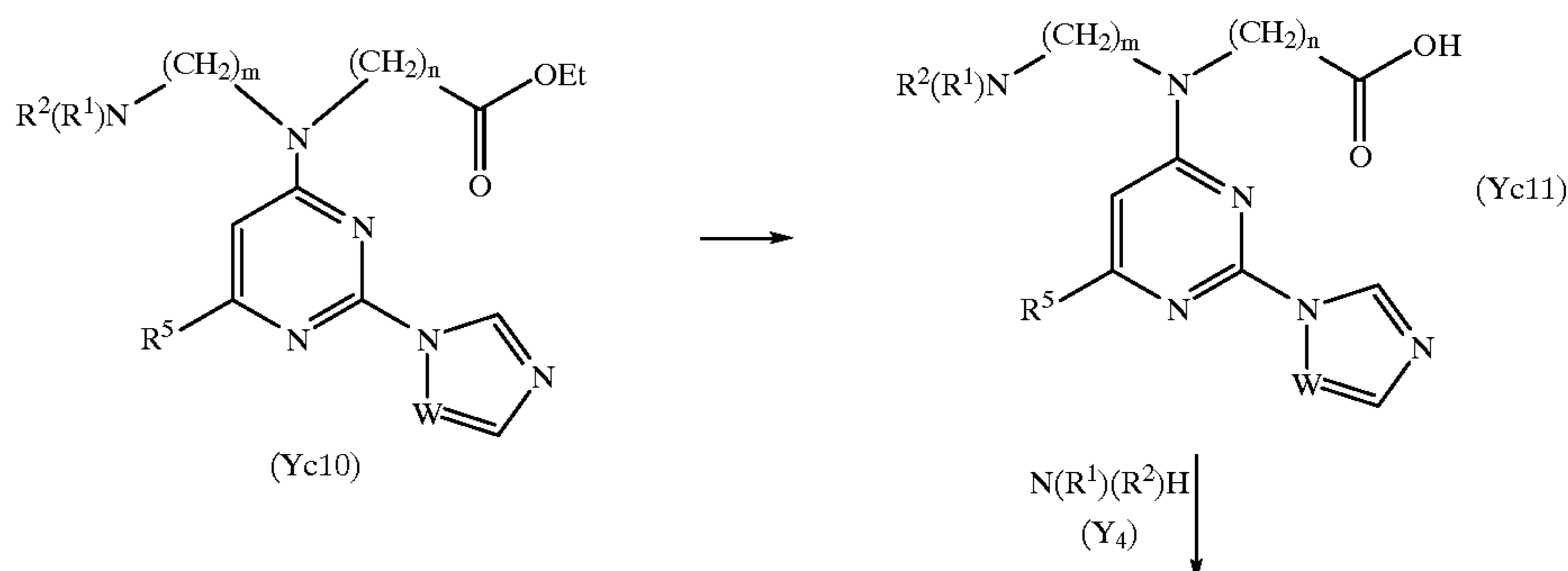
Reaction Scheme 6d
