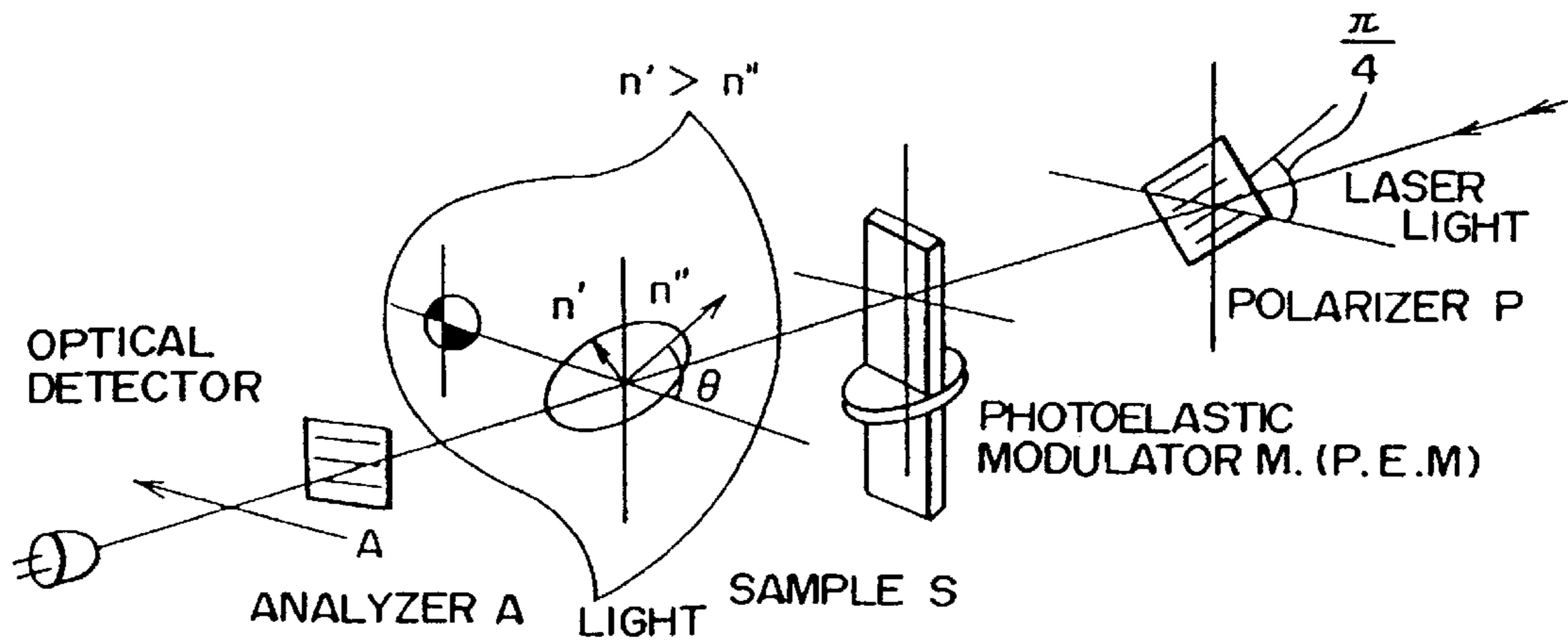
ARRANGEMENT OF OPTICAL ELEMENTS
