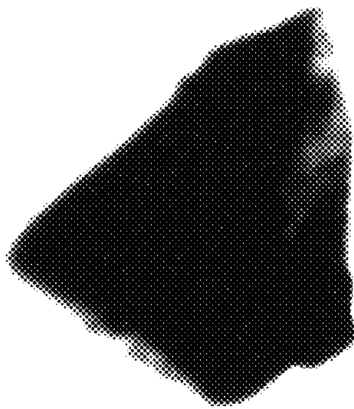
7S DOMAIN (50 \mu g/ml) FIG. 4b
