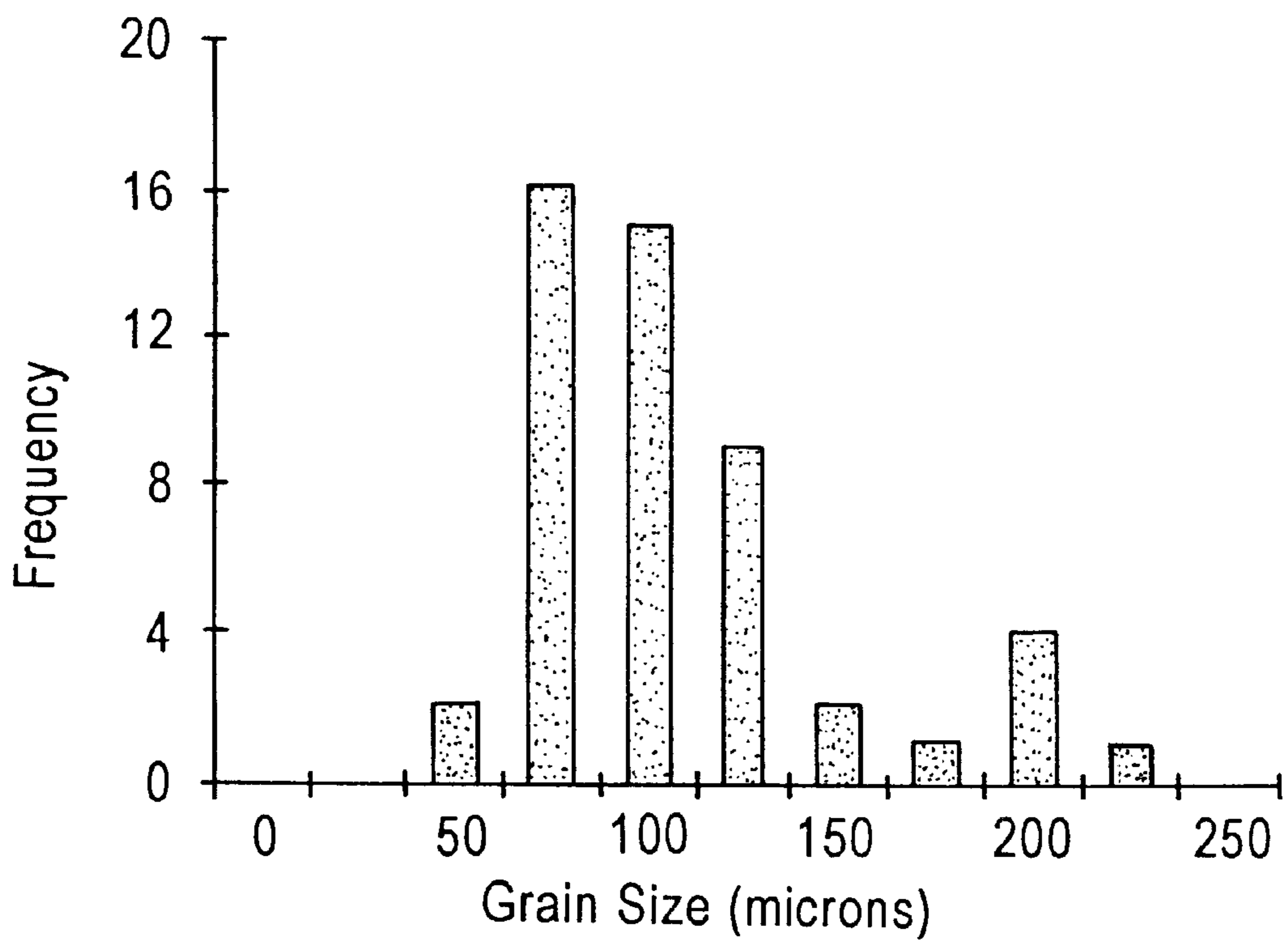
Grain Size Distribution
