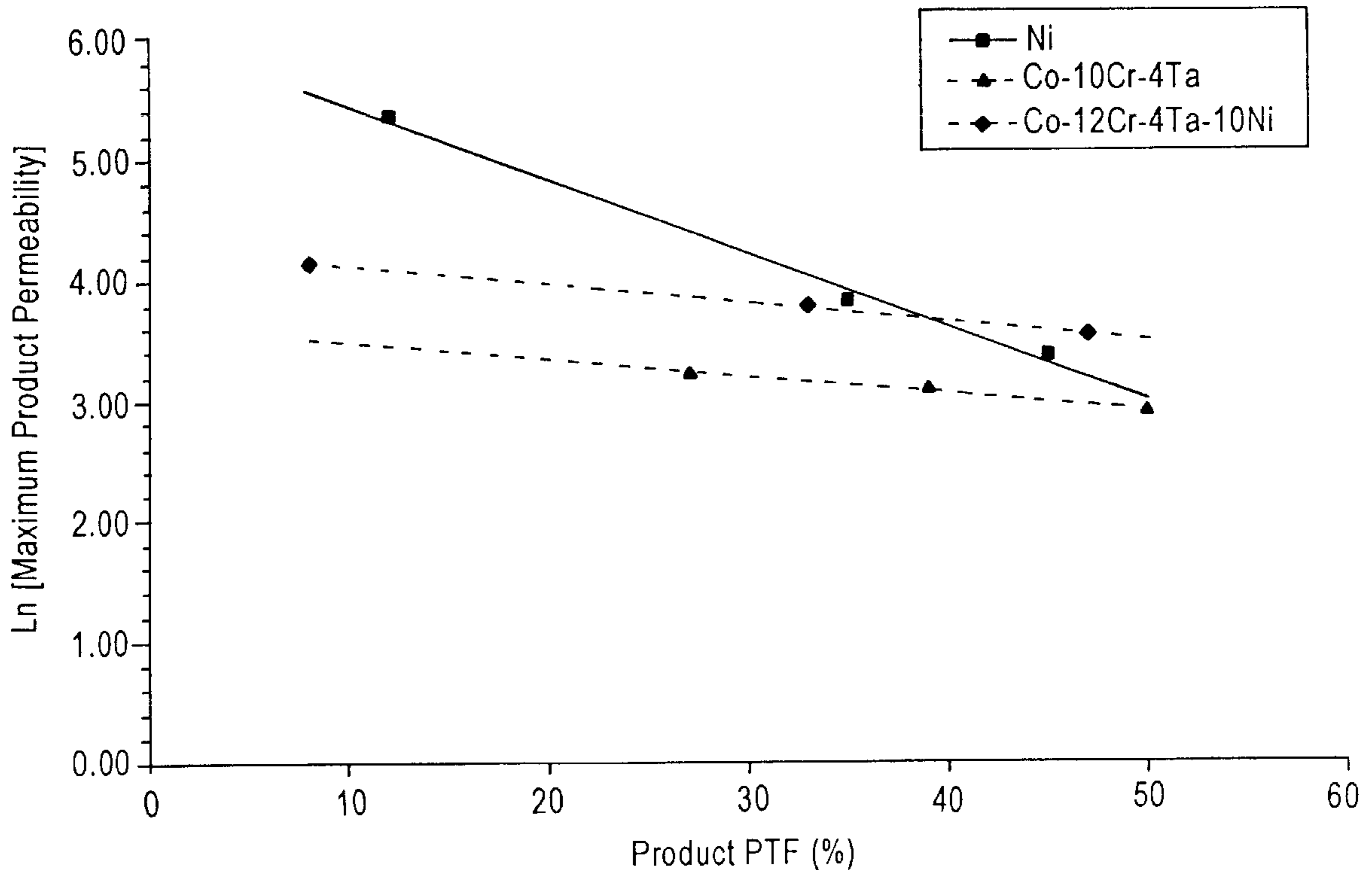
Relationship between PTF and maximum material permeability
