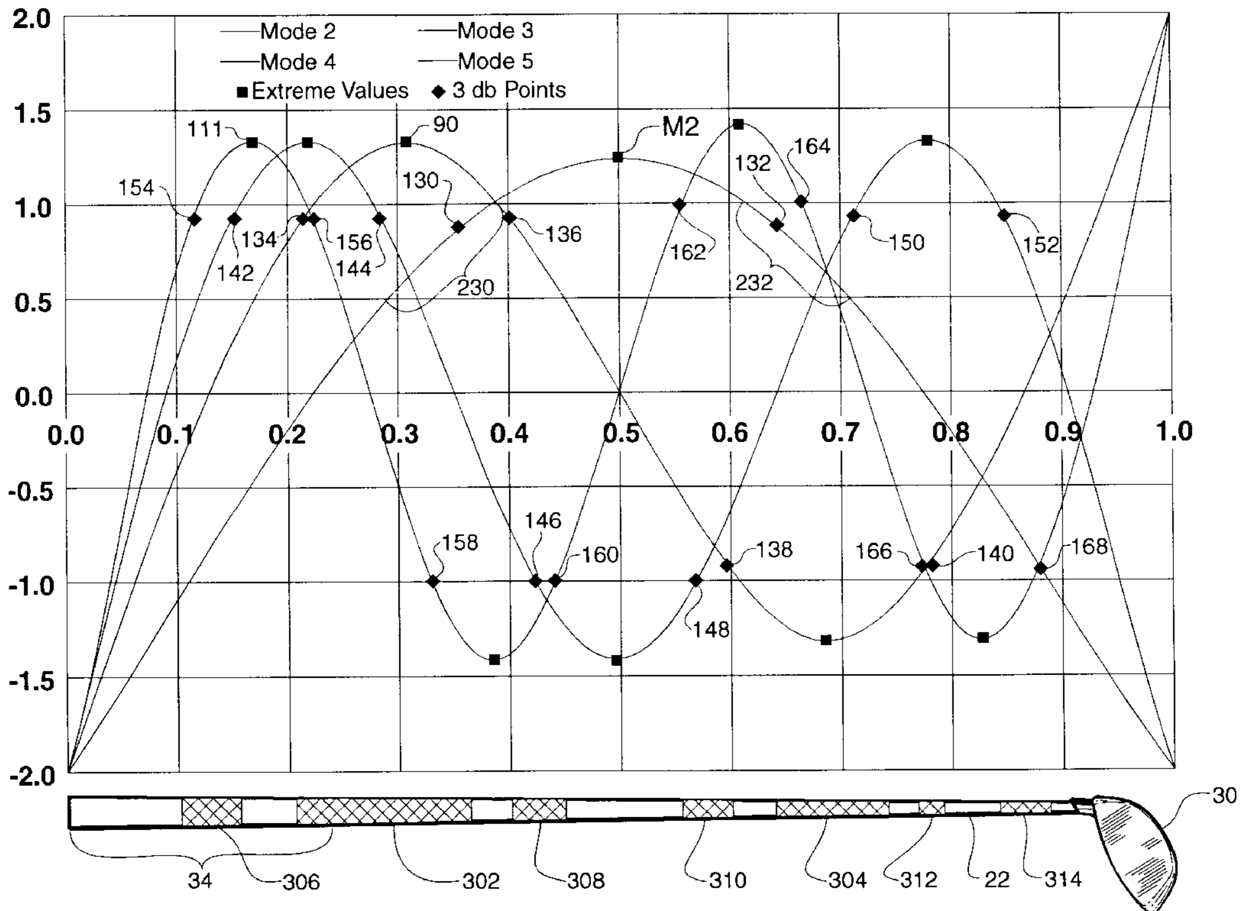
Normal Mode Shapes 2-5 for a Uniform Beam with Free-Free Boundary Conditions
