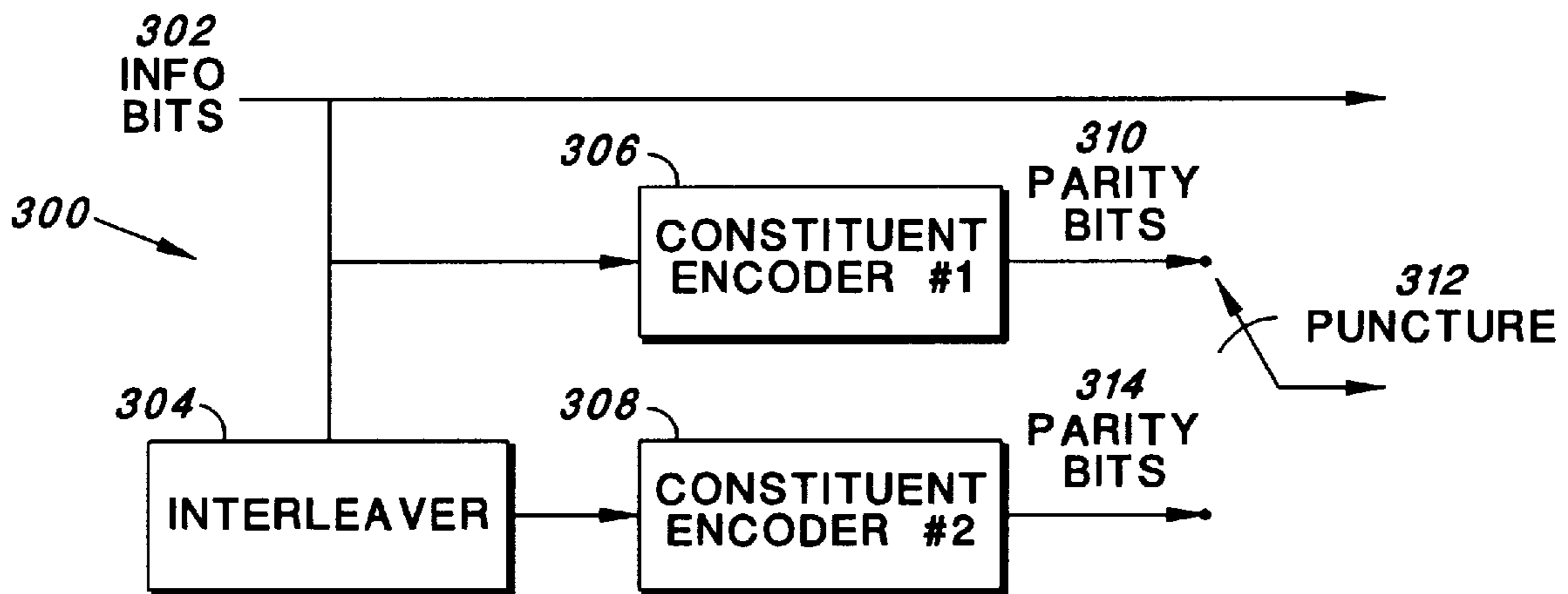
GENERIC TURBO CODE ENCODER BLOCK DIAGRAM
