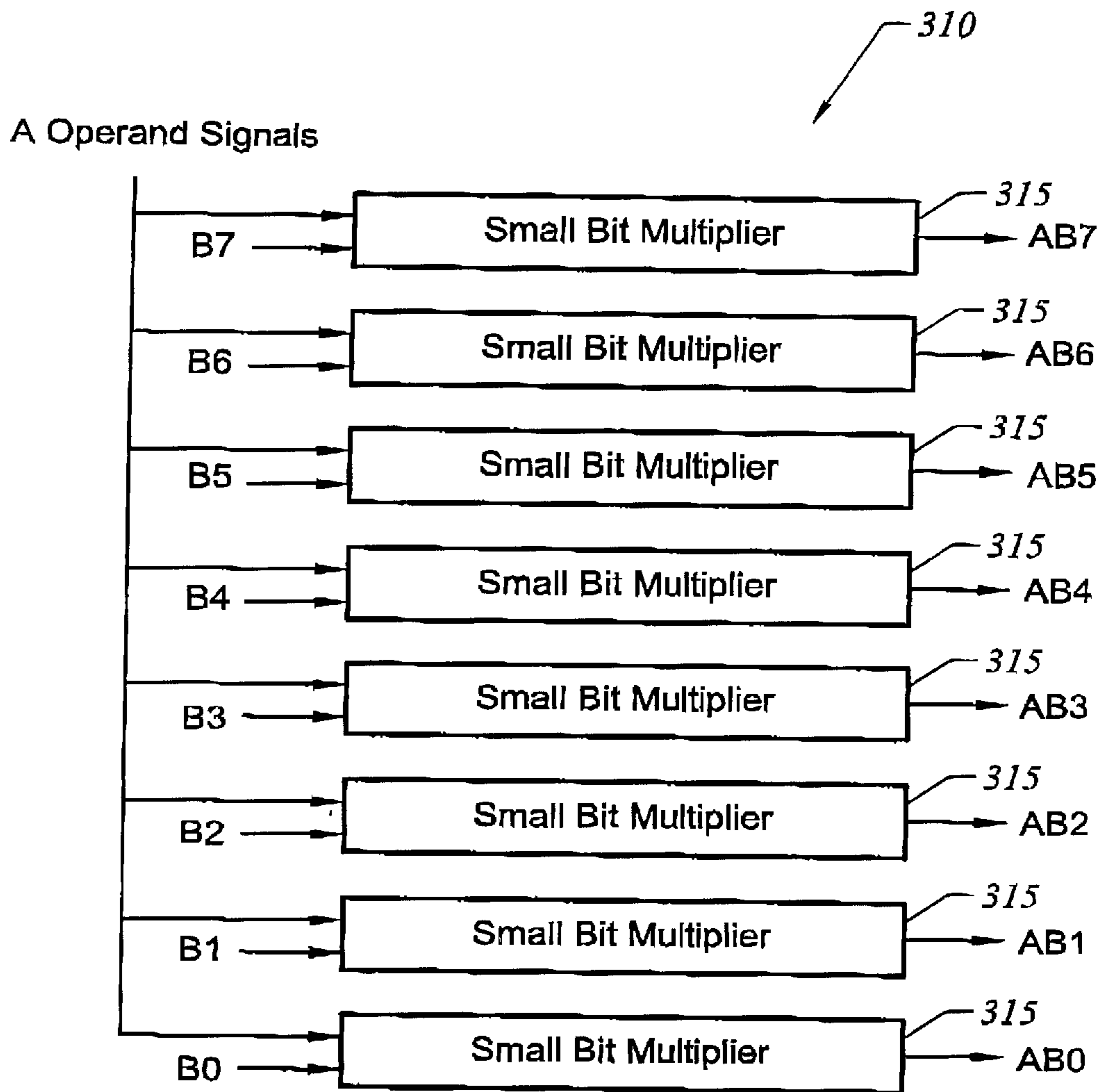
Small Bit Multiplier Array
