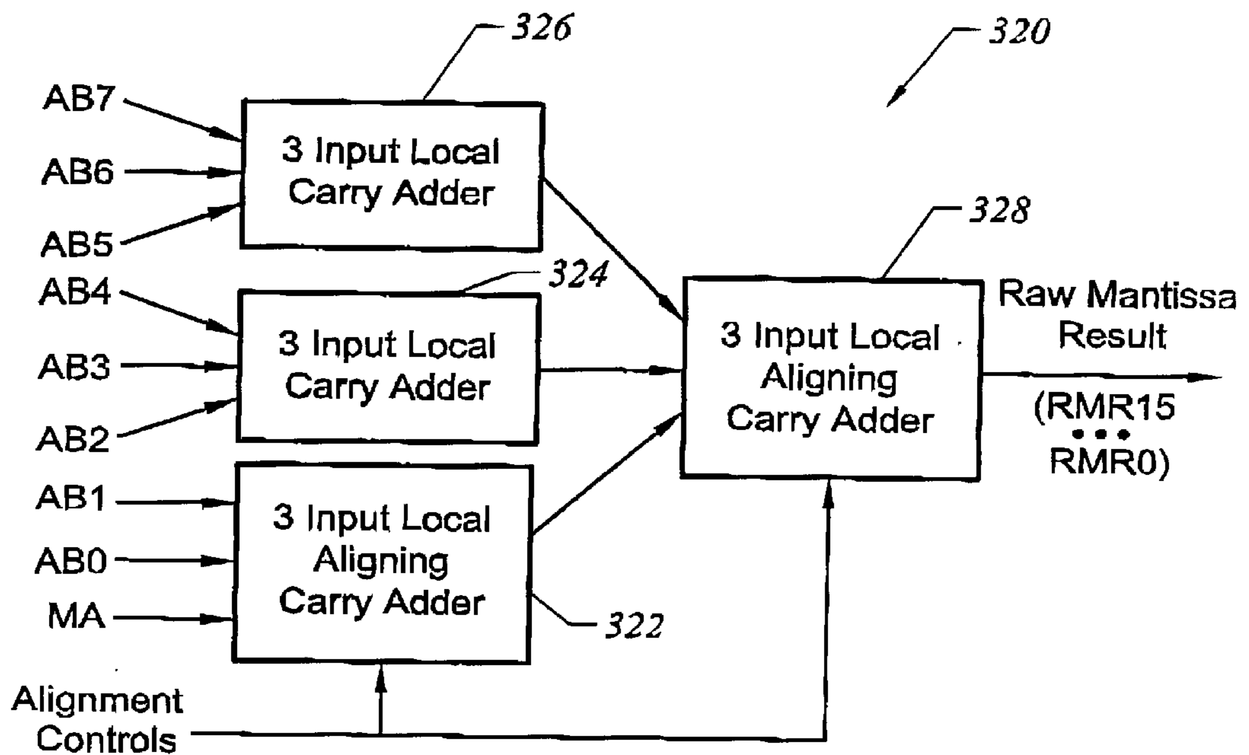
Single Precision Multiplier Adder Tree
