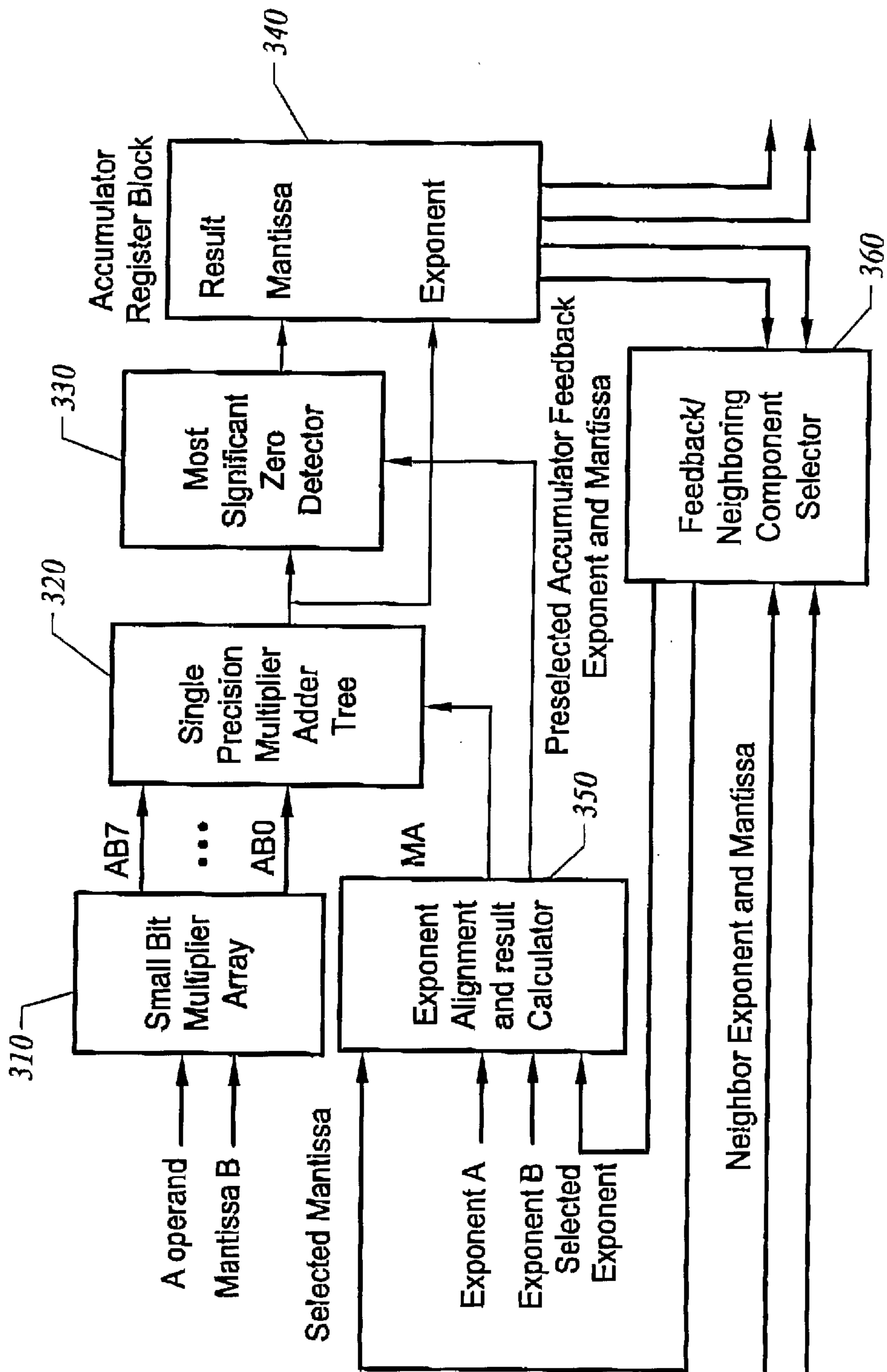
Single Precision Multiplier Block Diagram
