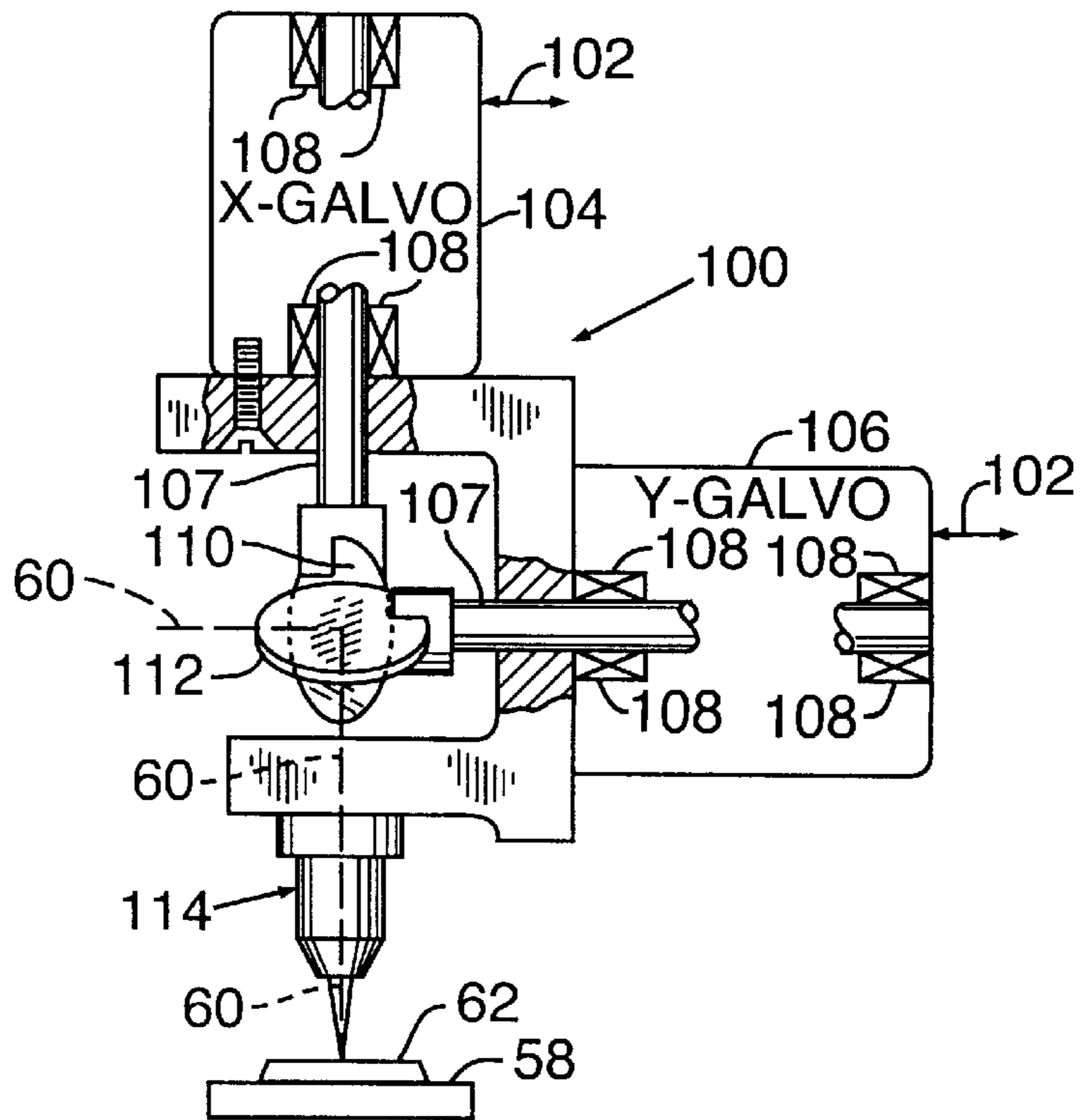
FIG. 3 (PRIOR ART)
