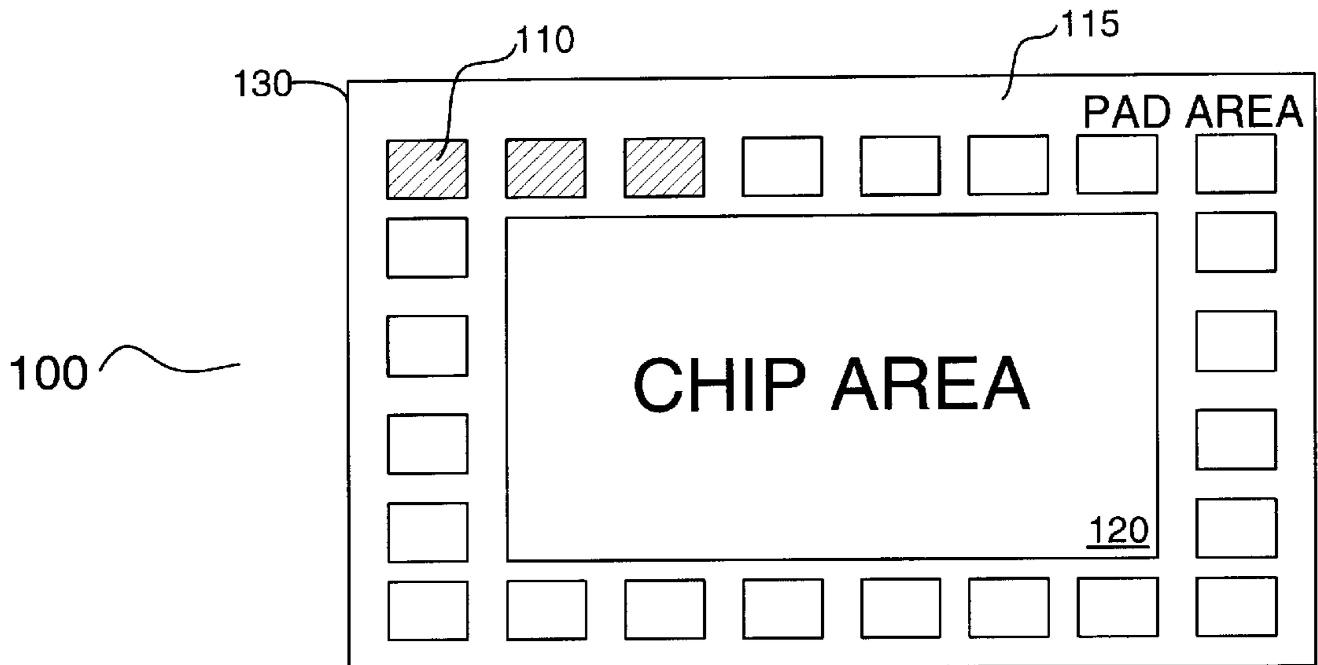
Fig. 1 (Prior Art)
