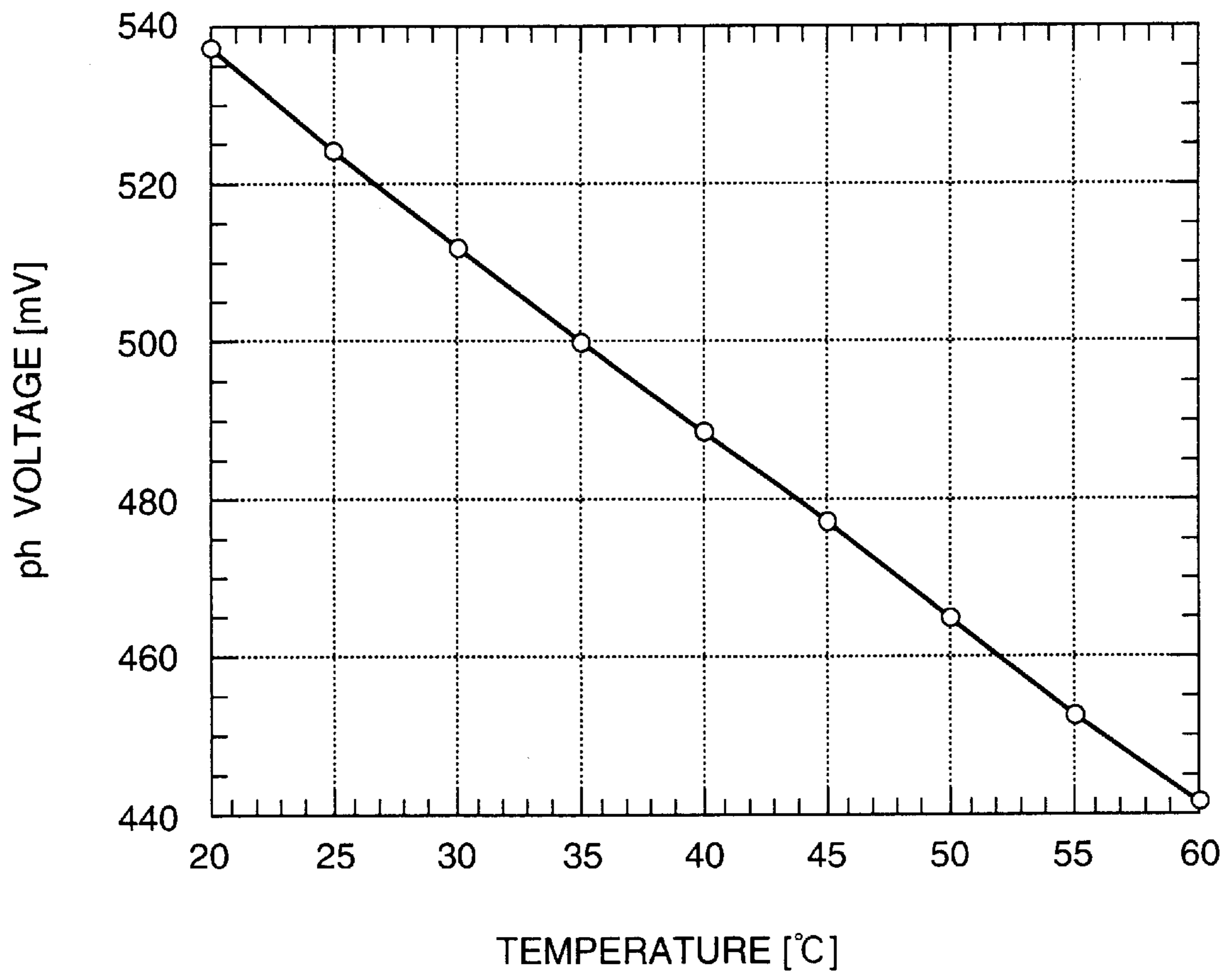
DNA CHIP TEMPERATURE-VOLTAGE CHARACTERISTIC
