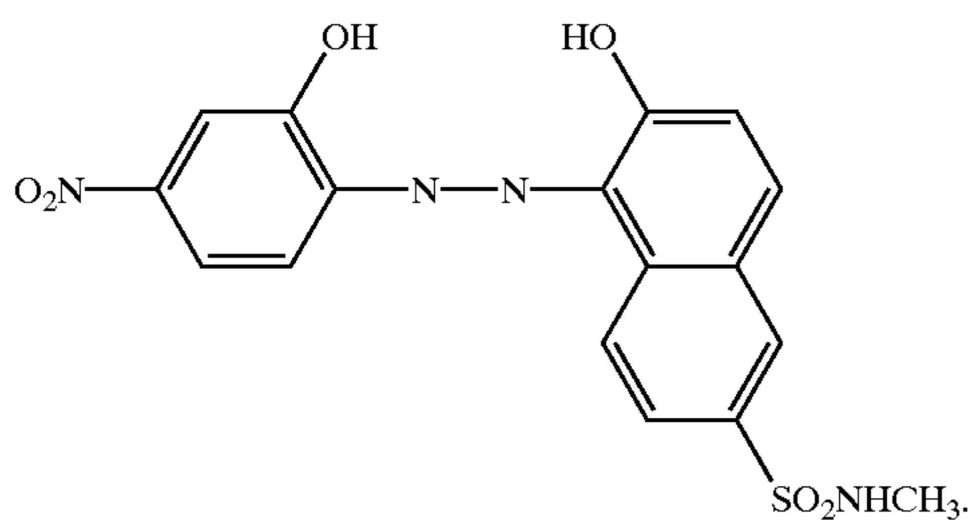
1:2 cobalt complex
