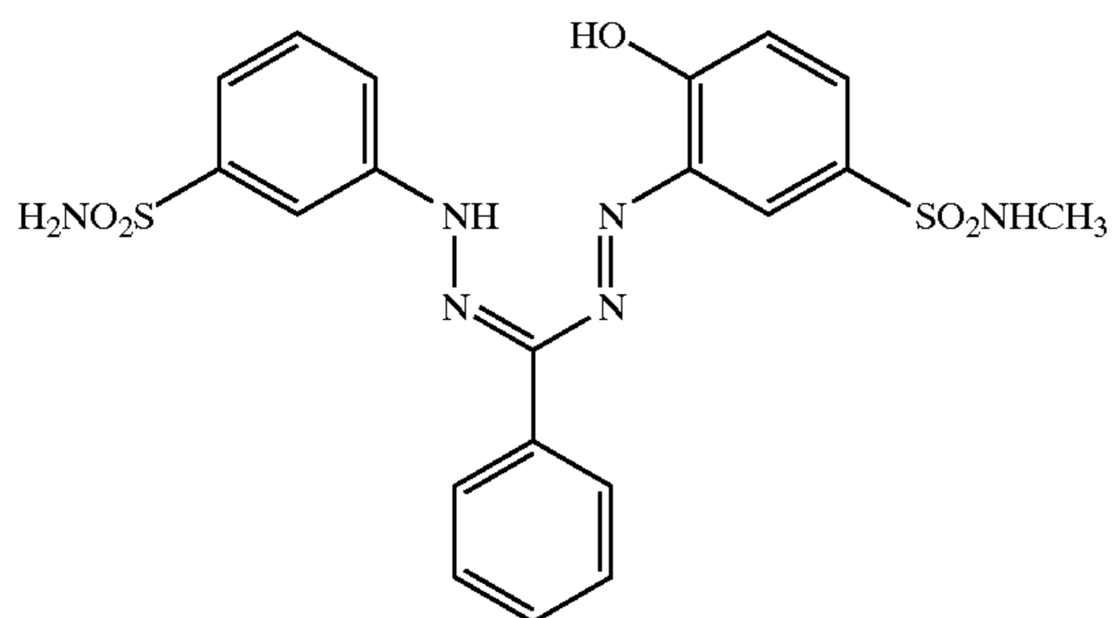
1:2 cobalt complex
