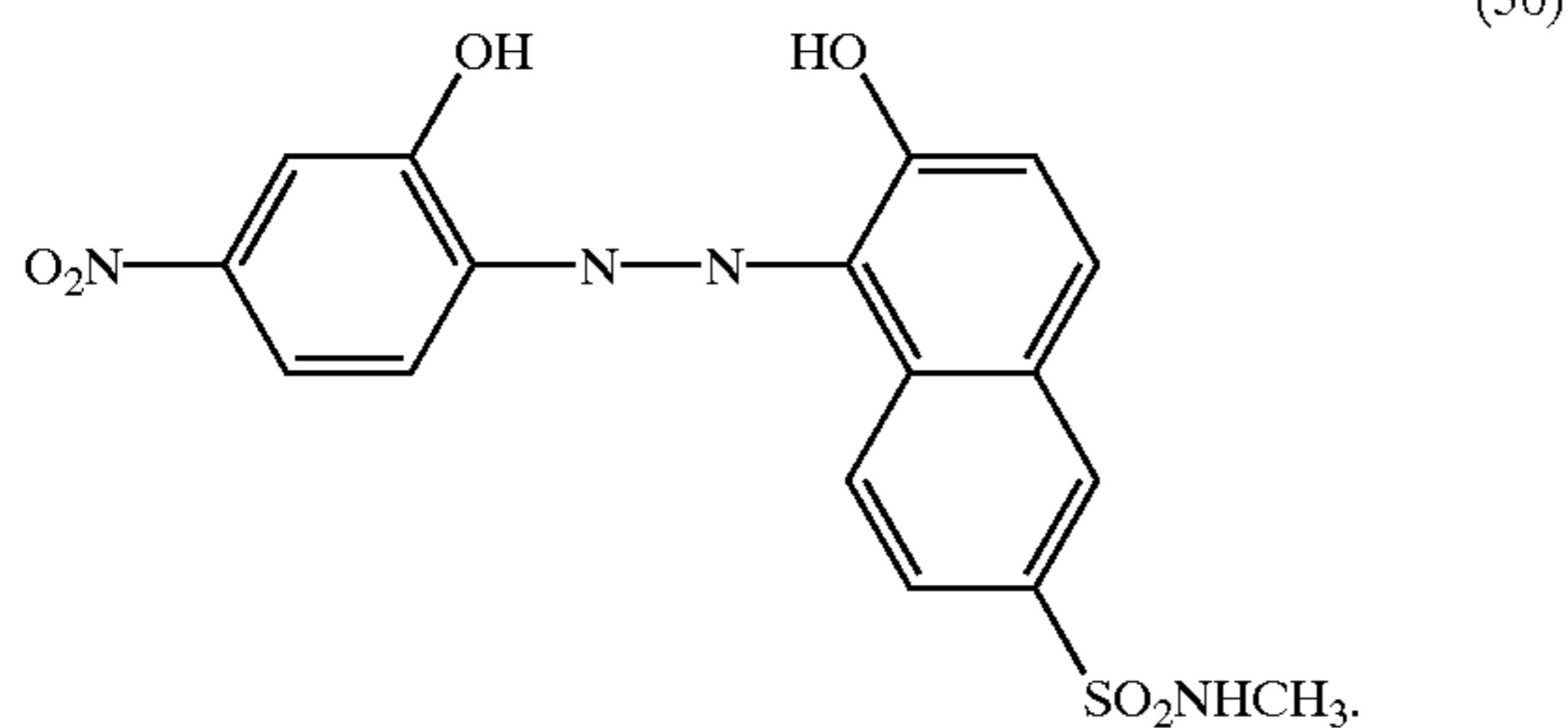
1:2 cobalt complex
