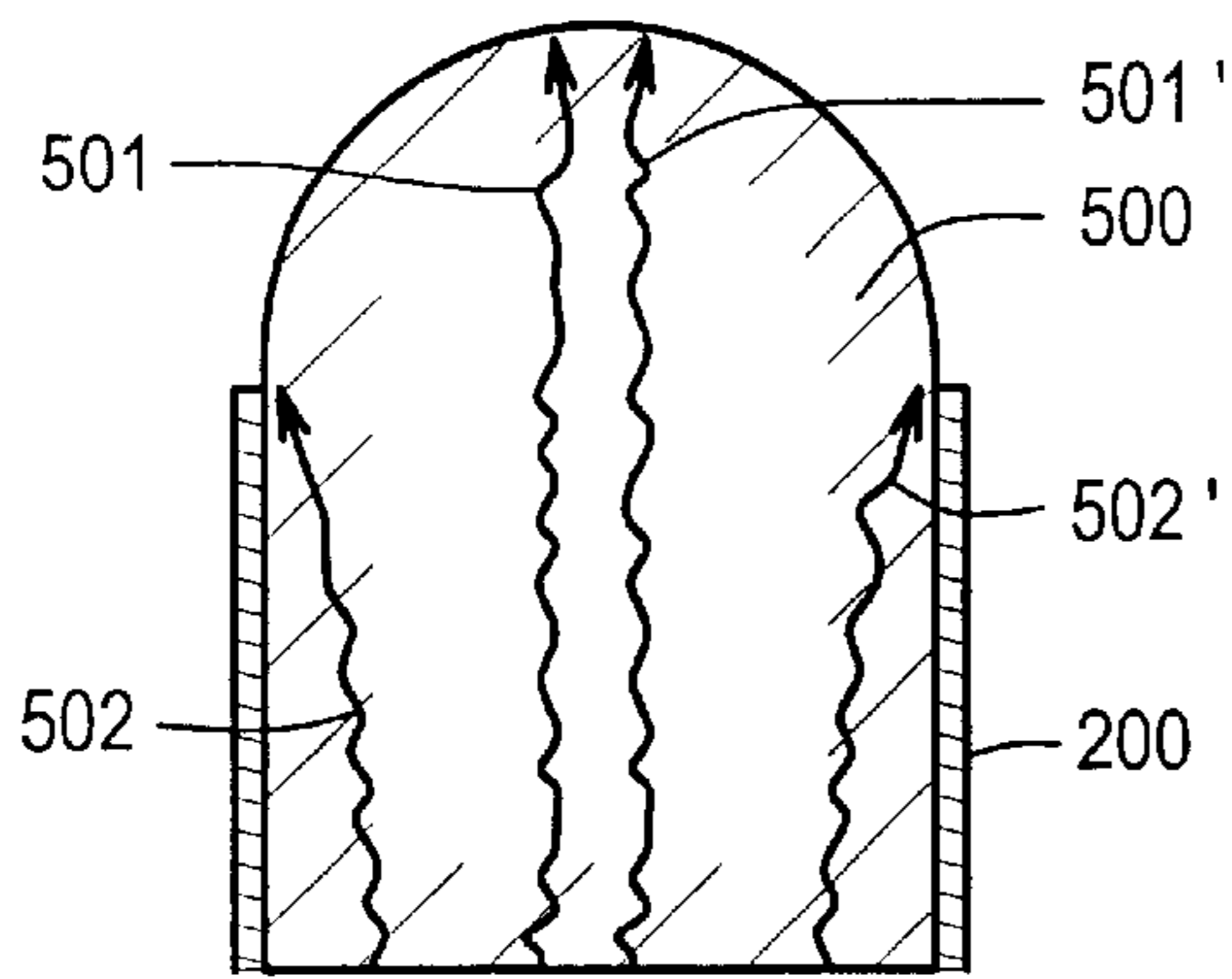
Fig. 2 Prior Art
