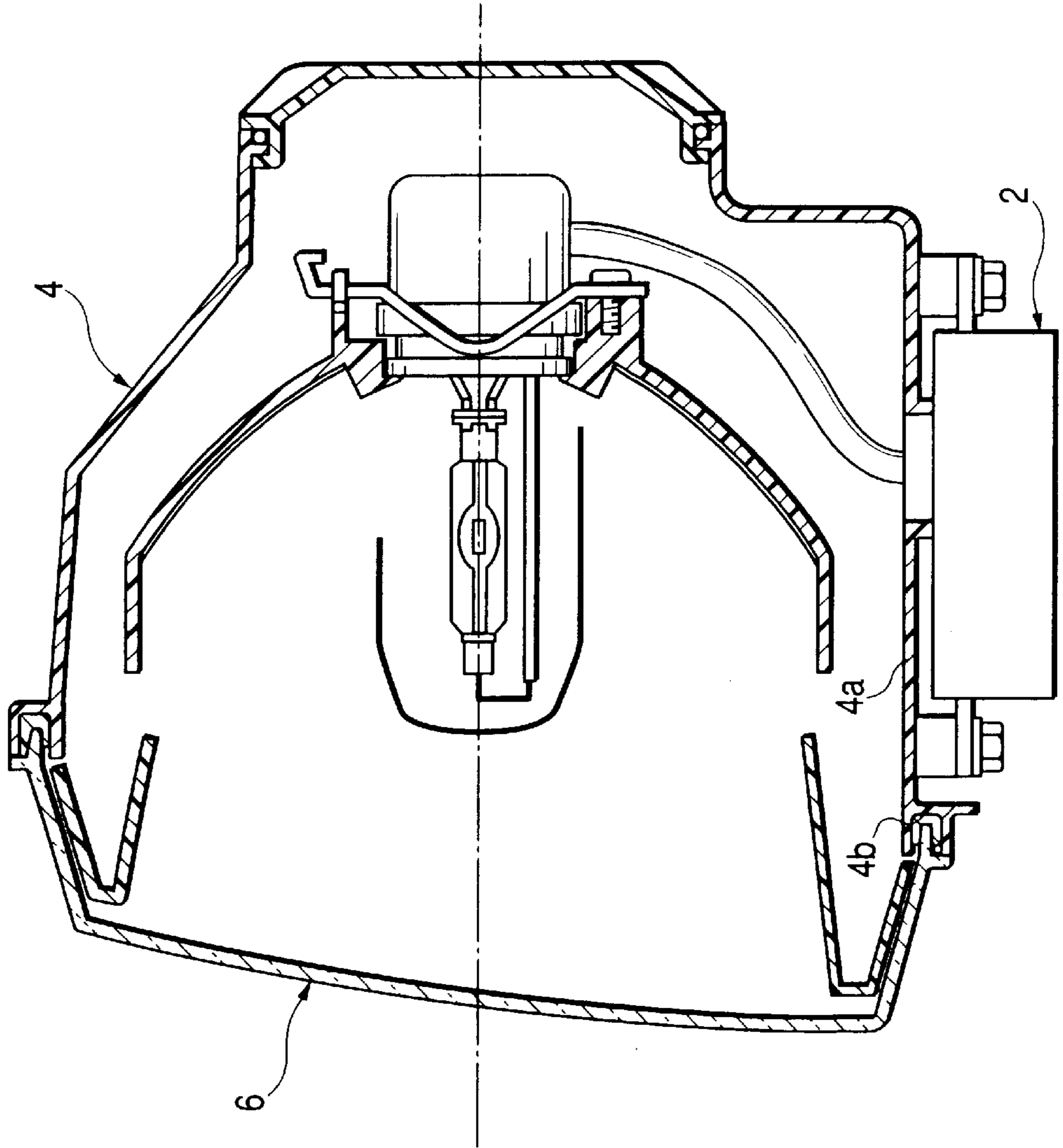
FIG. 4 PRIOR ART
