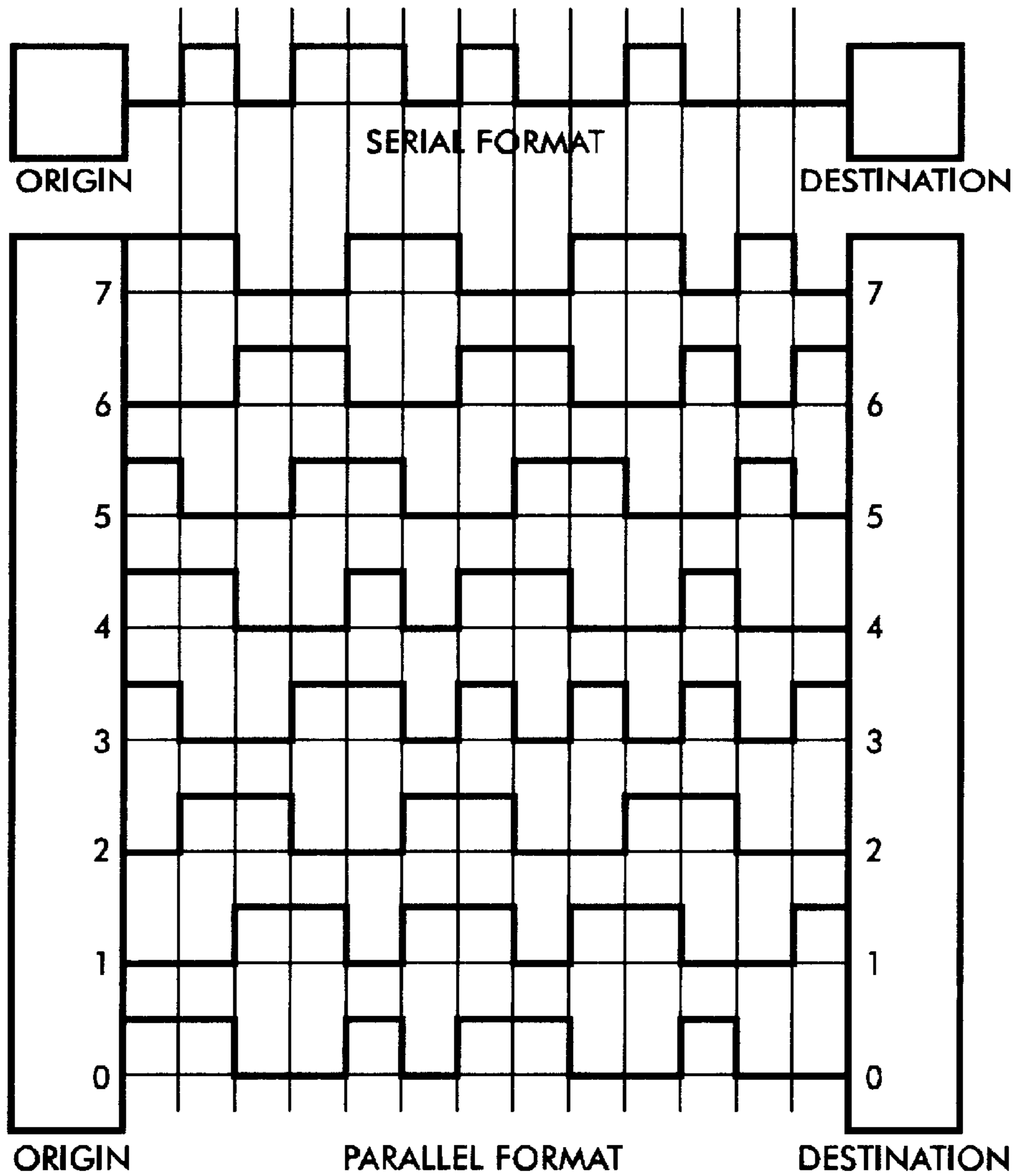
FIG.4 (PRIOR ART)
