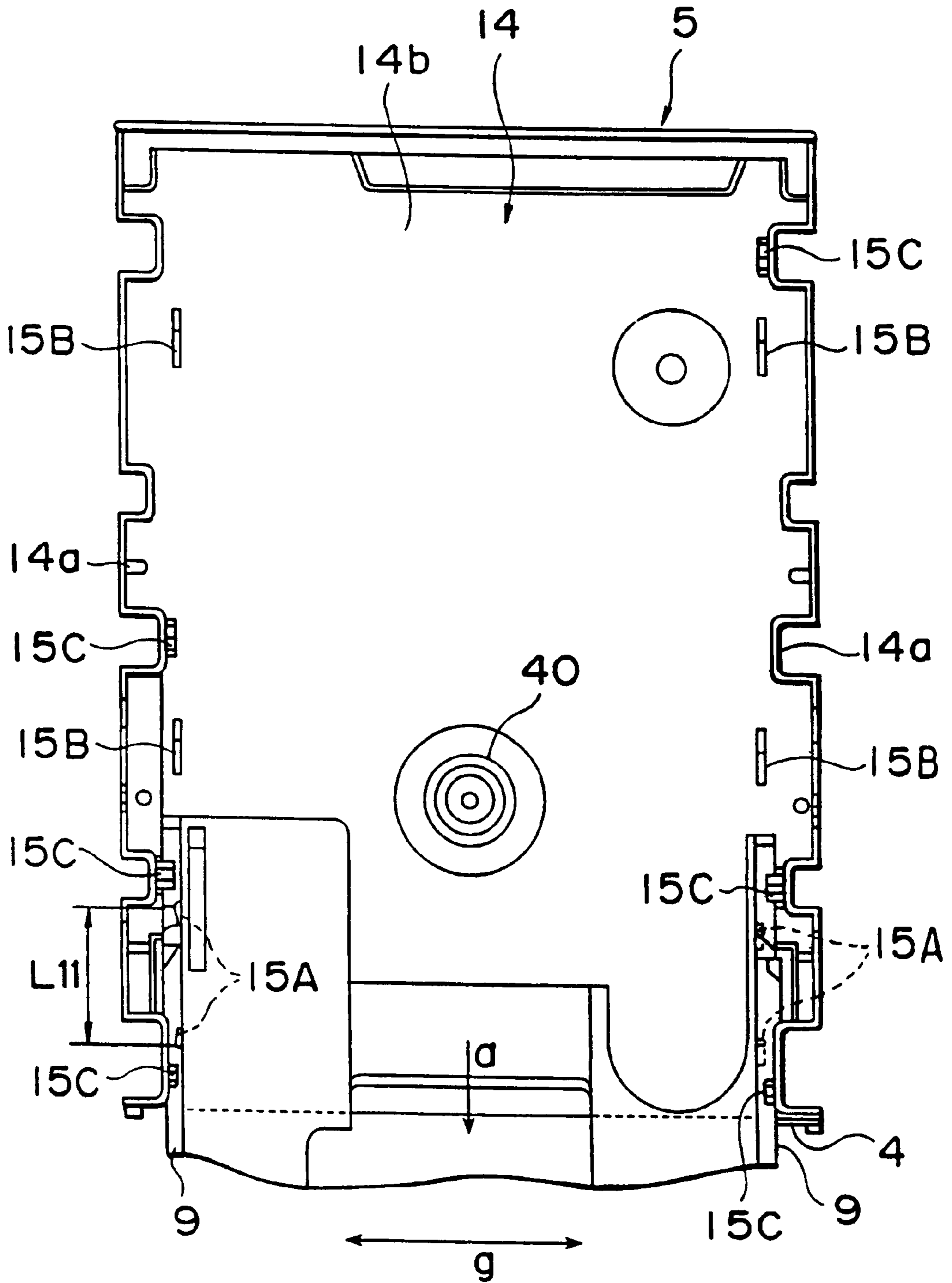
FIG. 10 PRIOR ART
