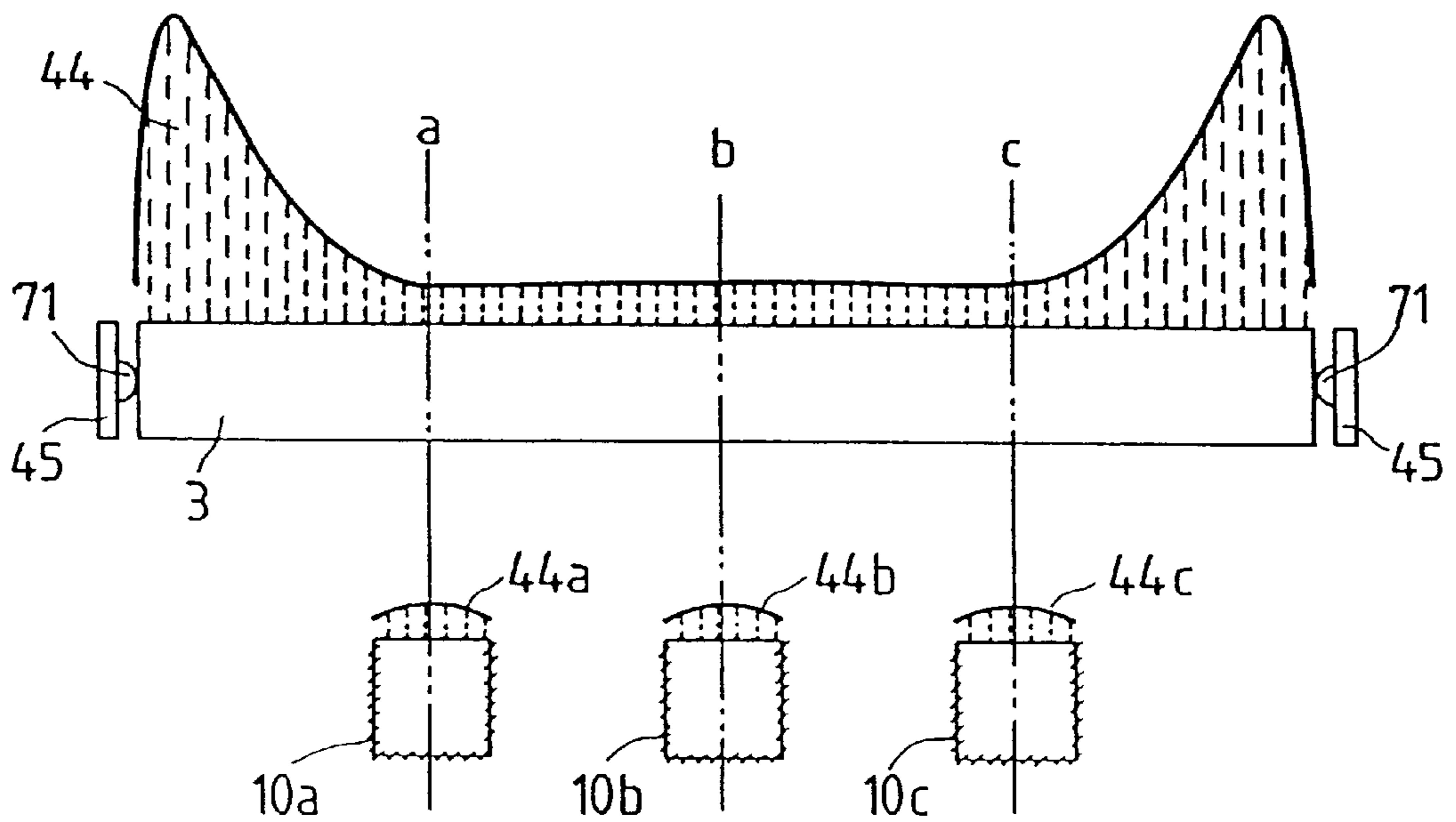
FIG. 9 PRIOR ART
