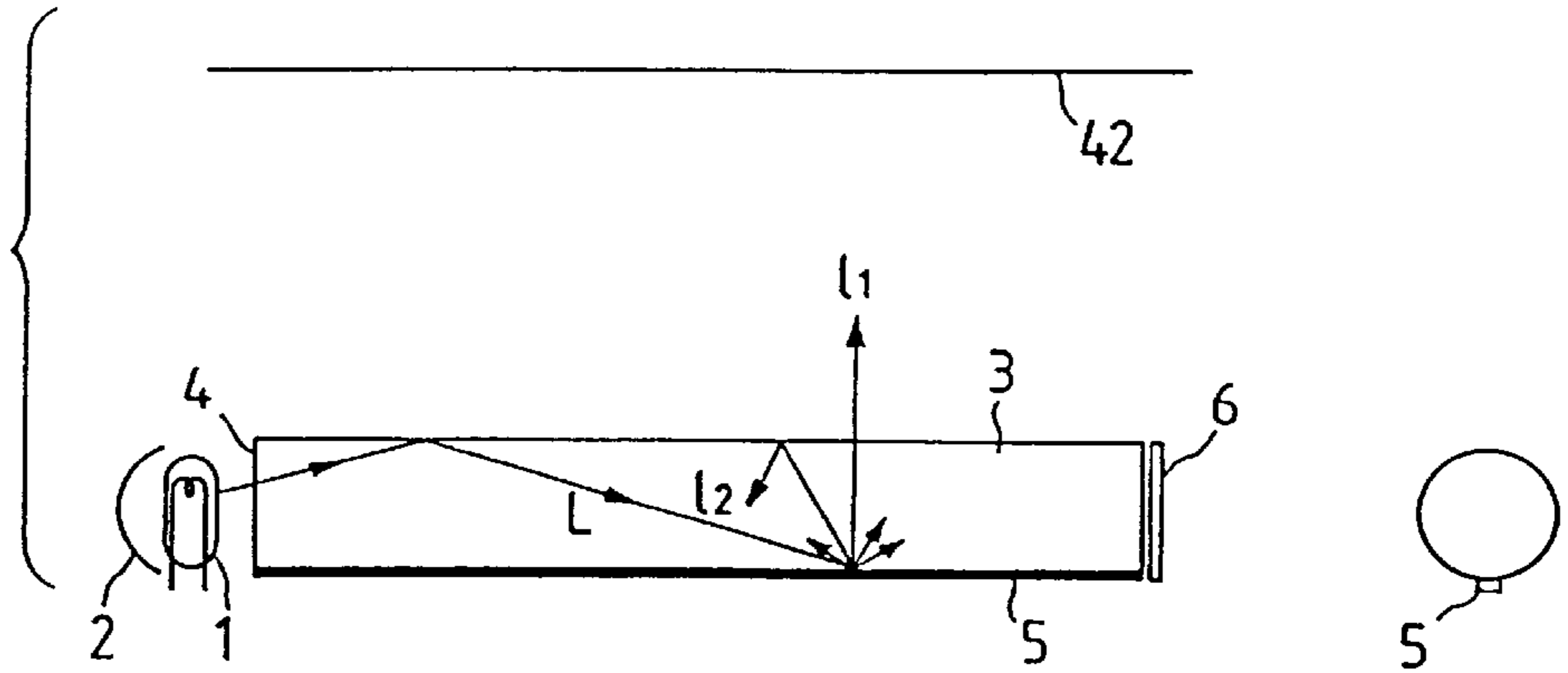
FIG. 5 PRIOR ART
