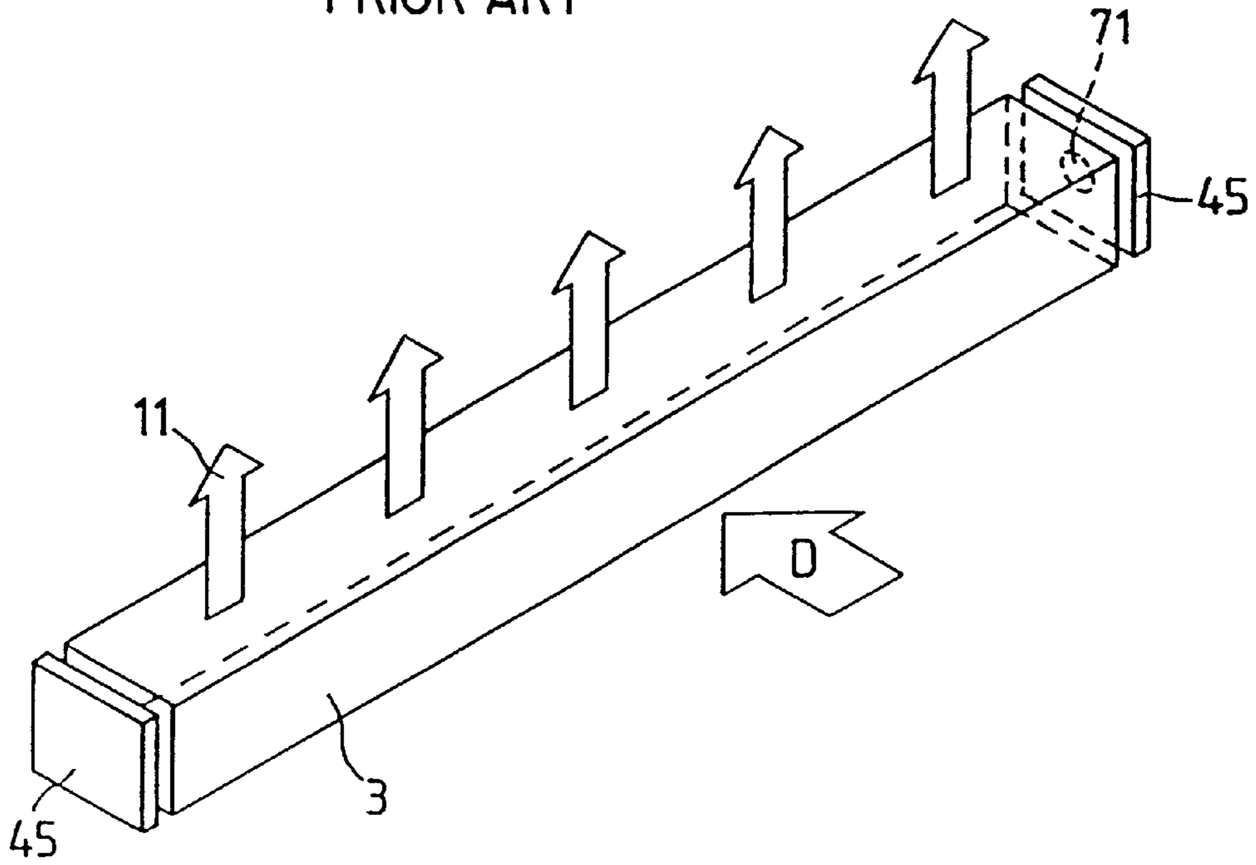
FIG. 8 PRIOR ART
