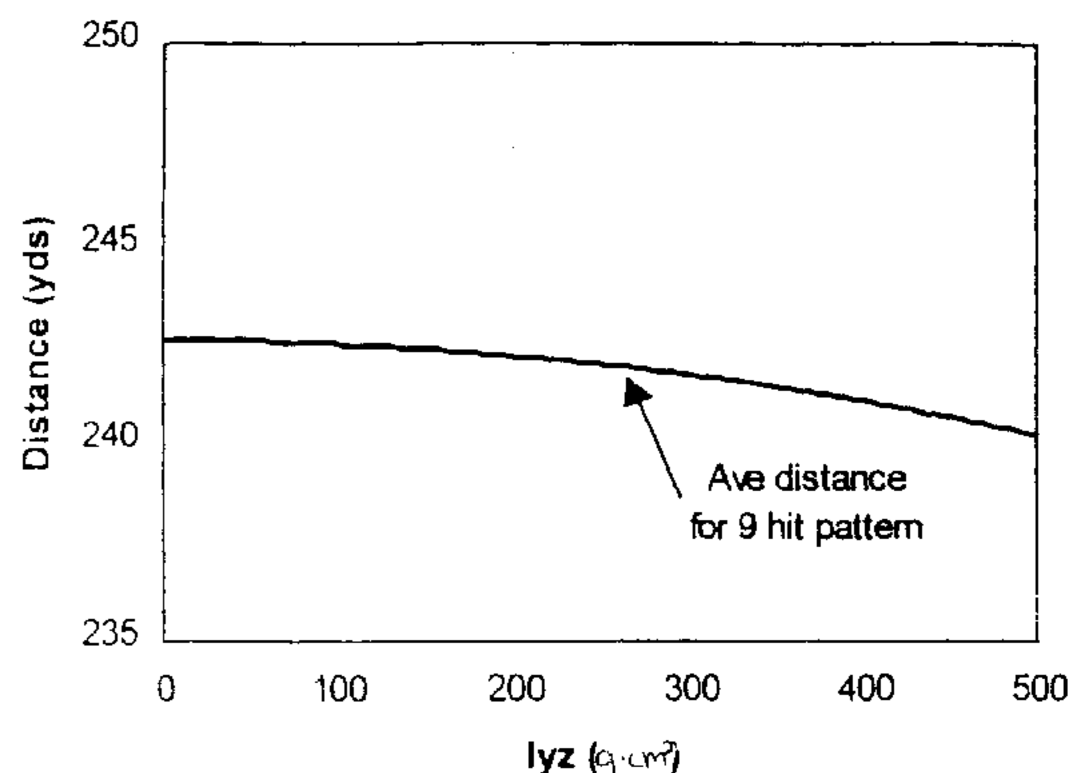
Effect of I_{yz} on distance 100 mph
