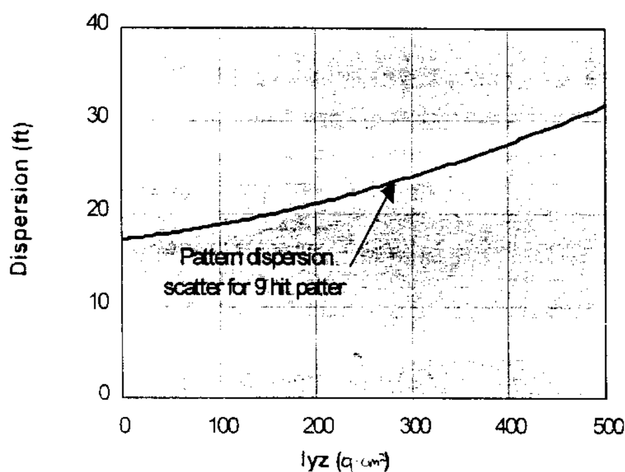
Effect of I_{yz} on Dispersion 100 mph
