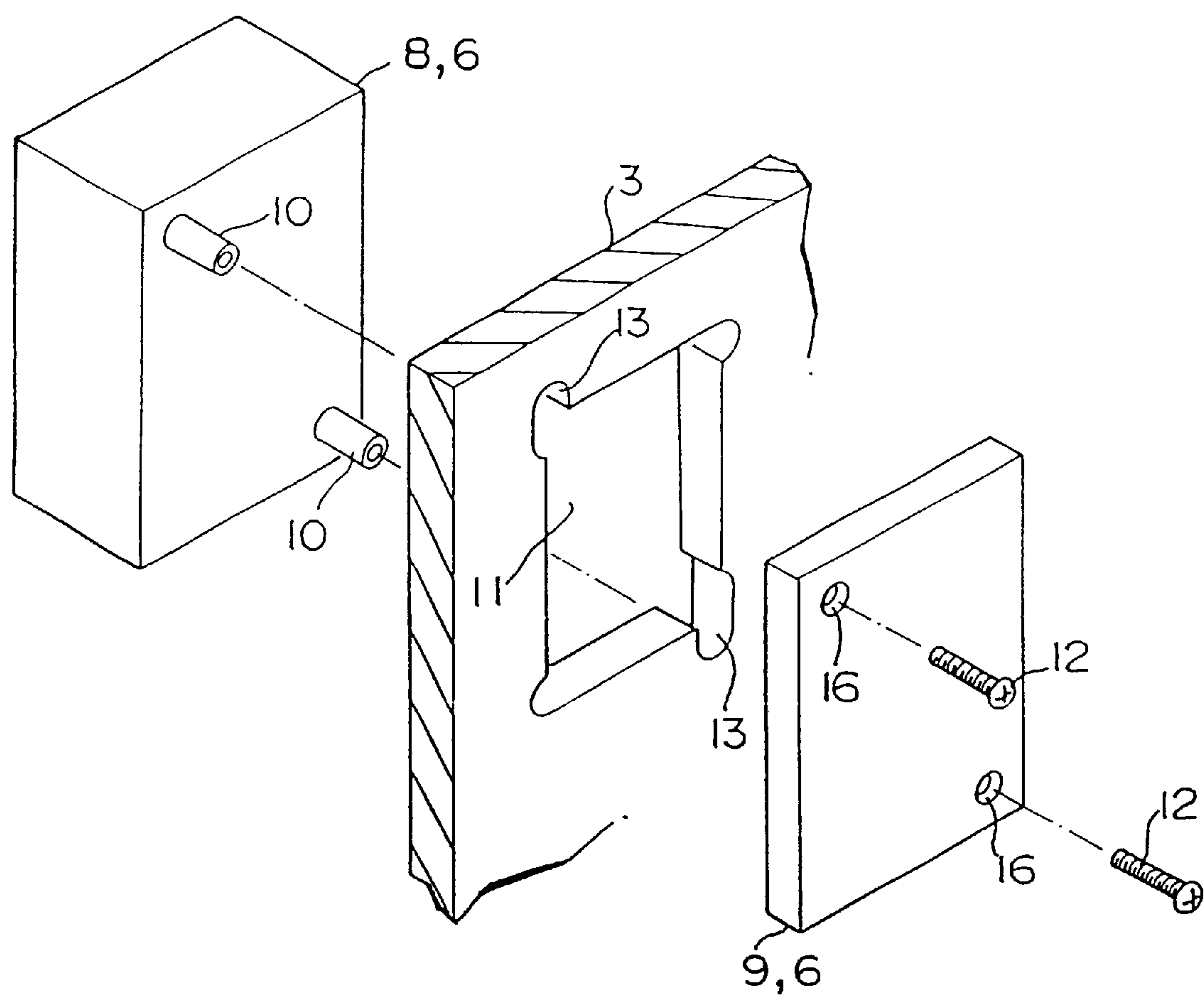
FIG. 47 (PRIOR ART)
