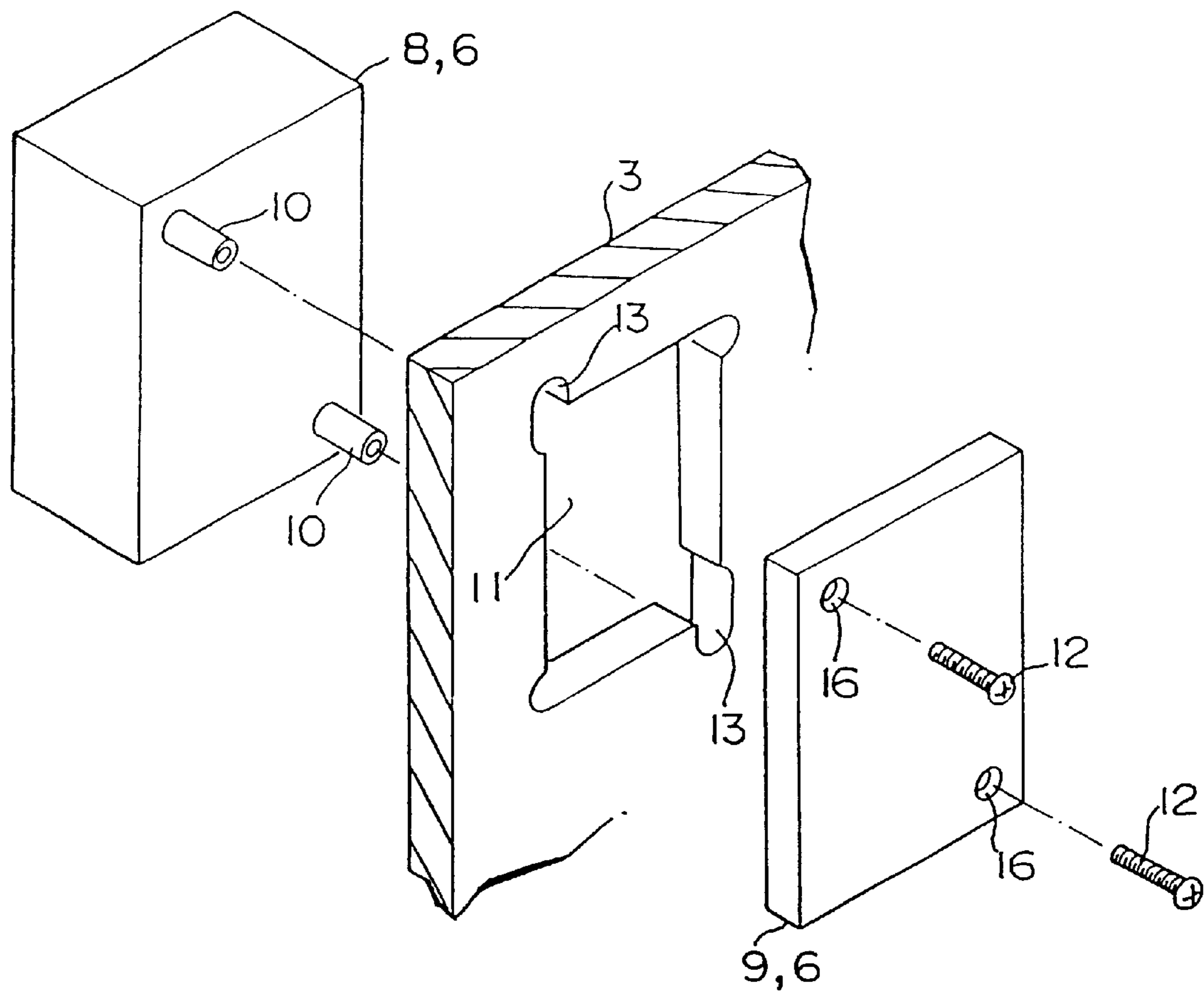
FIG. 47 (PRIOR ART)
