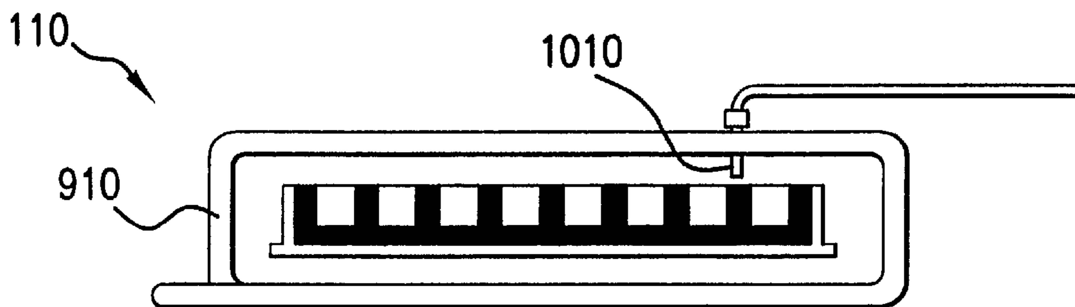
END VIEW-PLATE IN INDUCTION COIL WITH INFRARED FIBER OPTIC TEMPERATURE SENSOR
