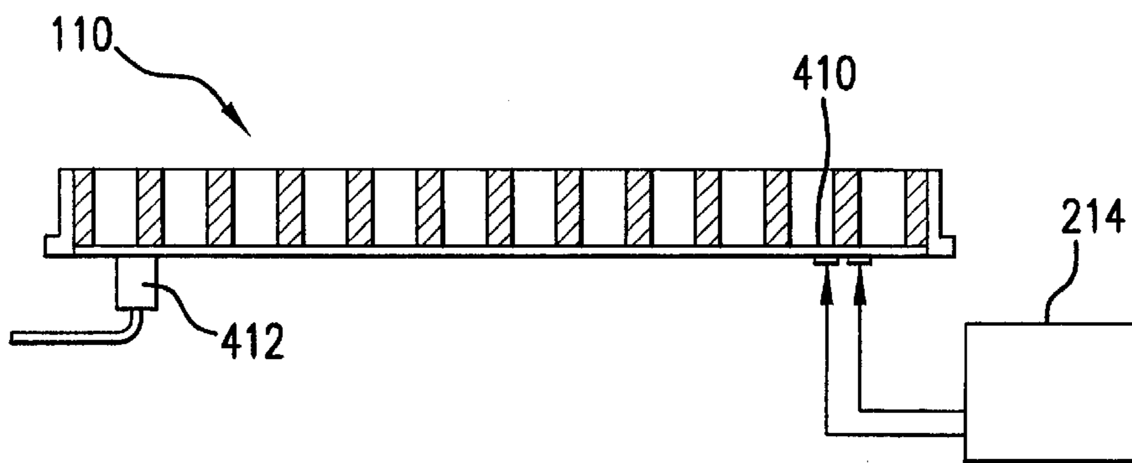
SECTION VIEW OF MICROTITER PLATE W/ OPTICALLY CLEAR HEATER AND CONTROLLER
