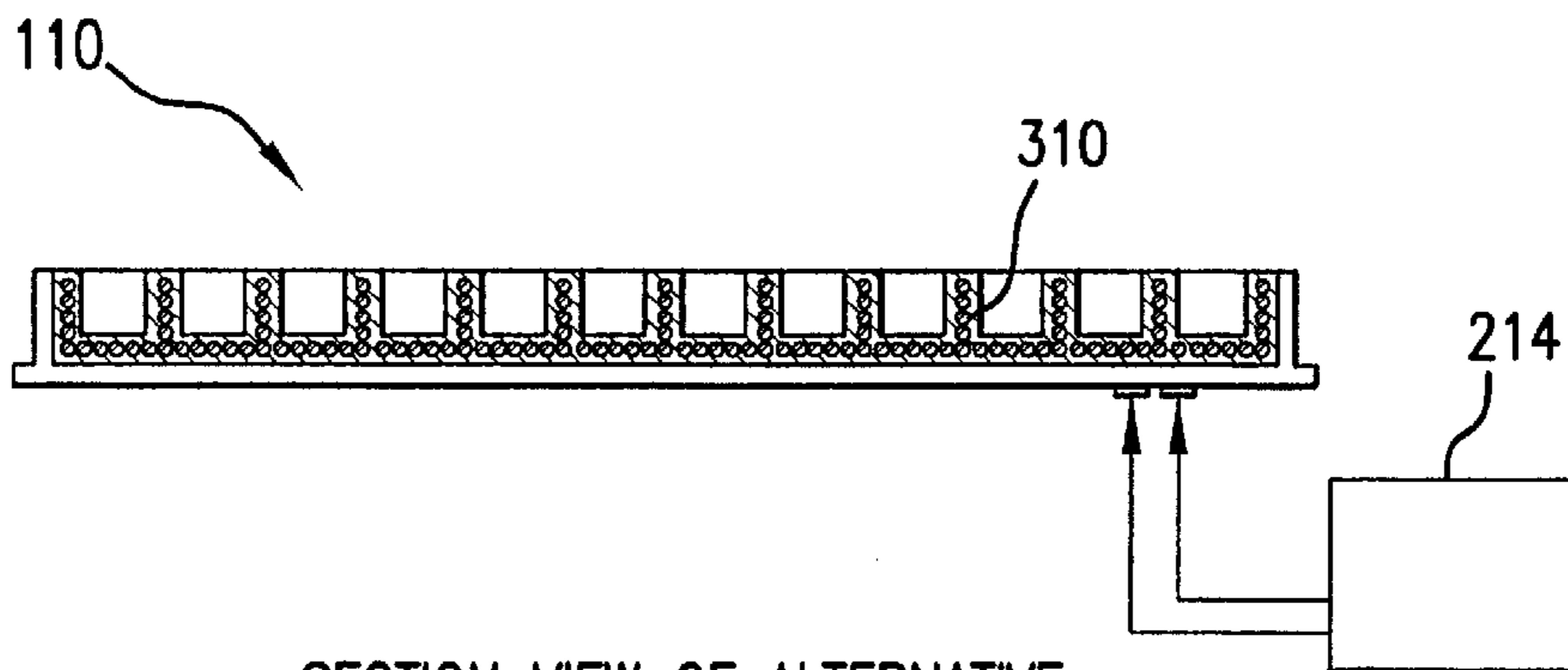
SECTION VIEW OF ALTERNATIVE HEATER W/CONTROLLER
