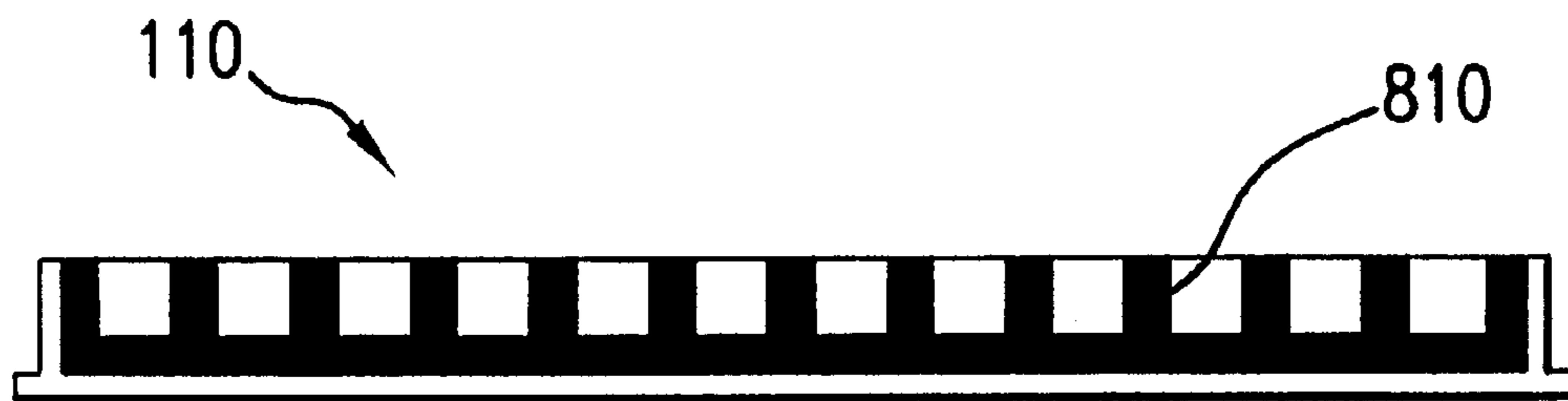
SECTION VIEW A-A' PLATE WITH FERROUS CONDUCTIVE MATERIAL FOR NON-CONTACT HEATING
