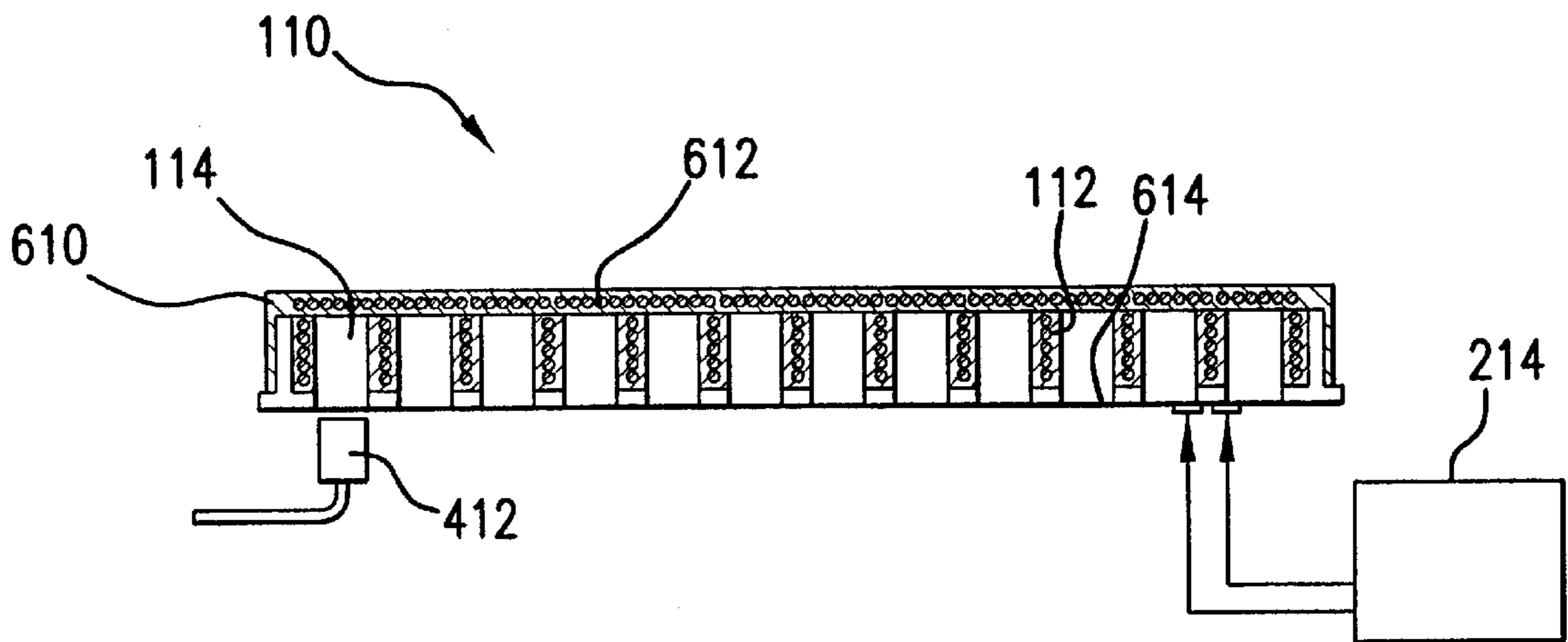
SECTION VIEW OF MICROTITER PLATE W/OPTICALLY CLEAR BOTTOM, INTEGRATED HEATER, CONTROLLER & HEATED LID
