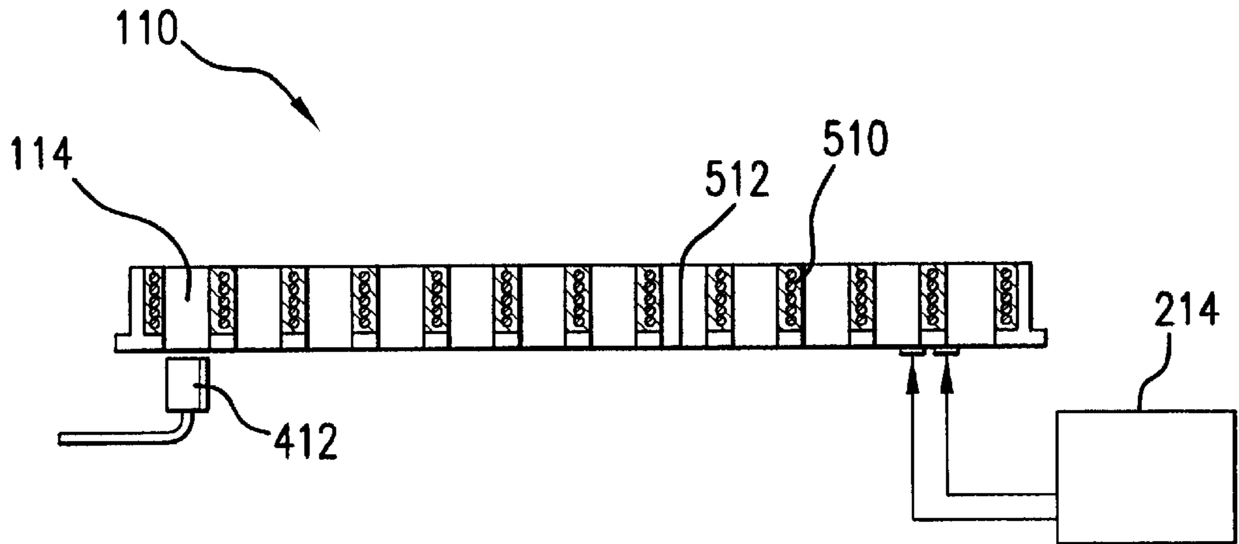
SECTION VIEW OF MICROTITER PLATE W/OPTICALLY CLEAR BOTTOM, INTEGRATED HEATER AND CONTROLLER
