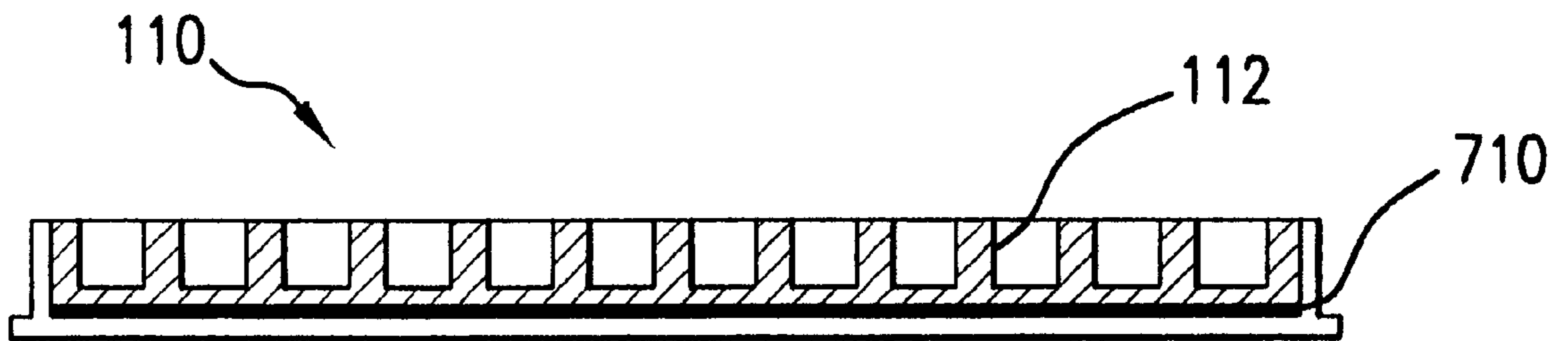
SECTION VIEW A-A' PLATE WITH INTEGRATED FERROUS PLATE FOR NON-CONTACT HEATING
