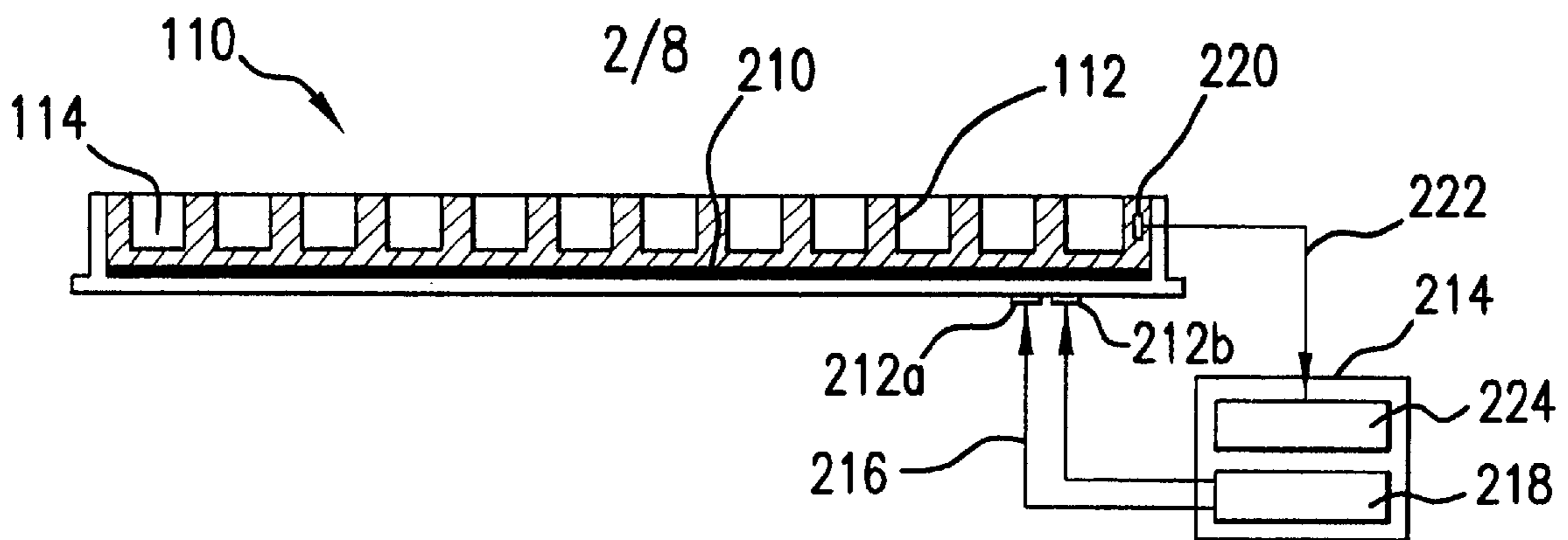
SECTION VIEW A-A' WITH CONTROLLER
