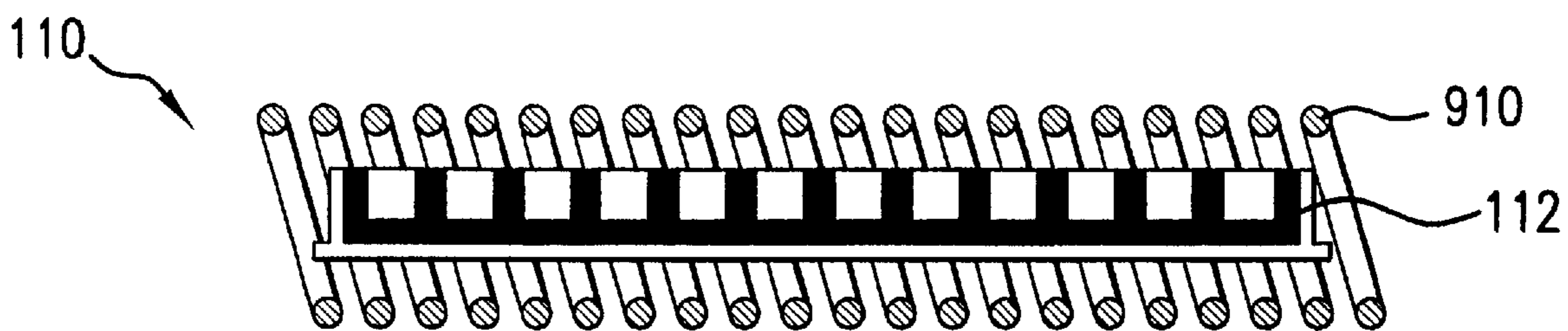
SECTION VIEW-PLATE IN INDUCTION COIL WITH INFRARED FIBER OPTIC TEMPERATURE SENSOR
