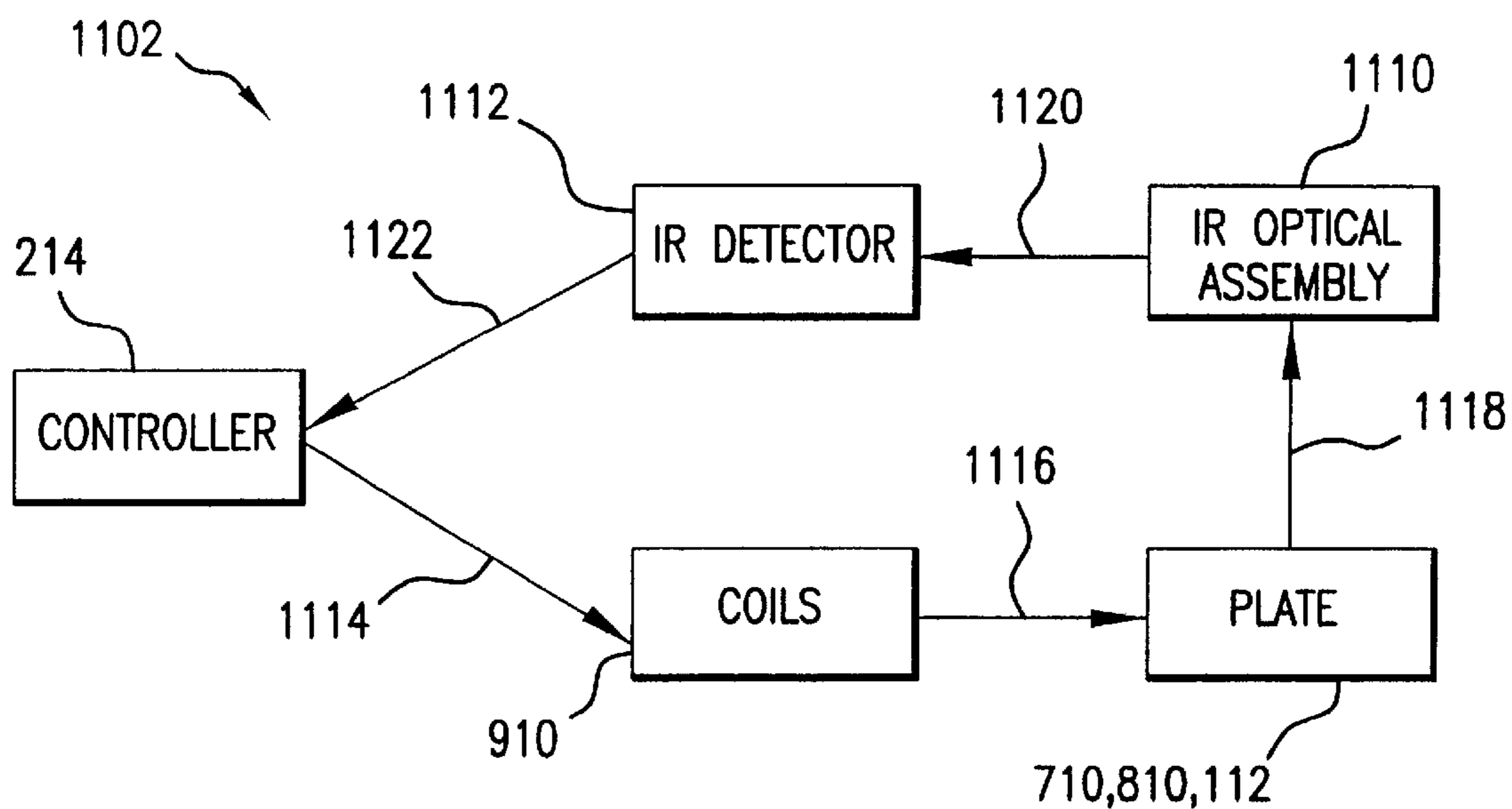
SCHEMATIC-INDUCTIVE HEATING AND NON-CONTACT TEMPERATURE MEASUREMENT & CONTROL SYSTEM
