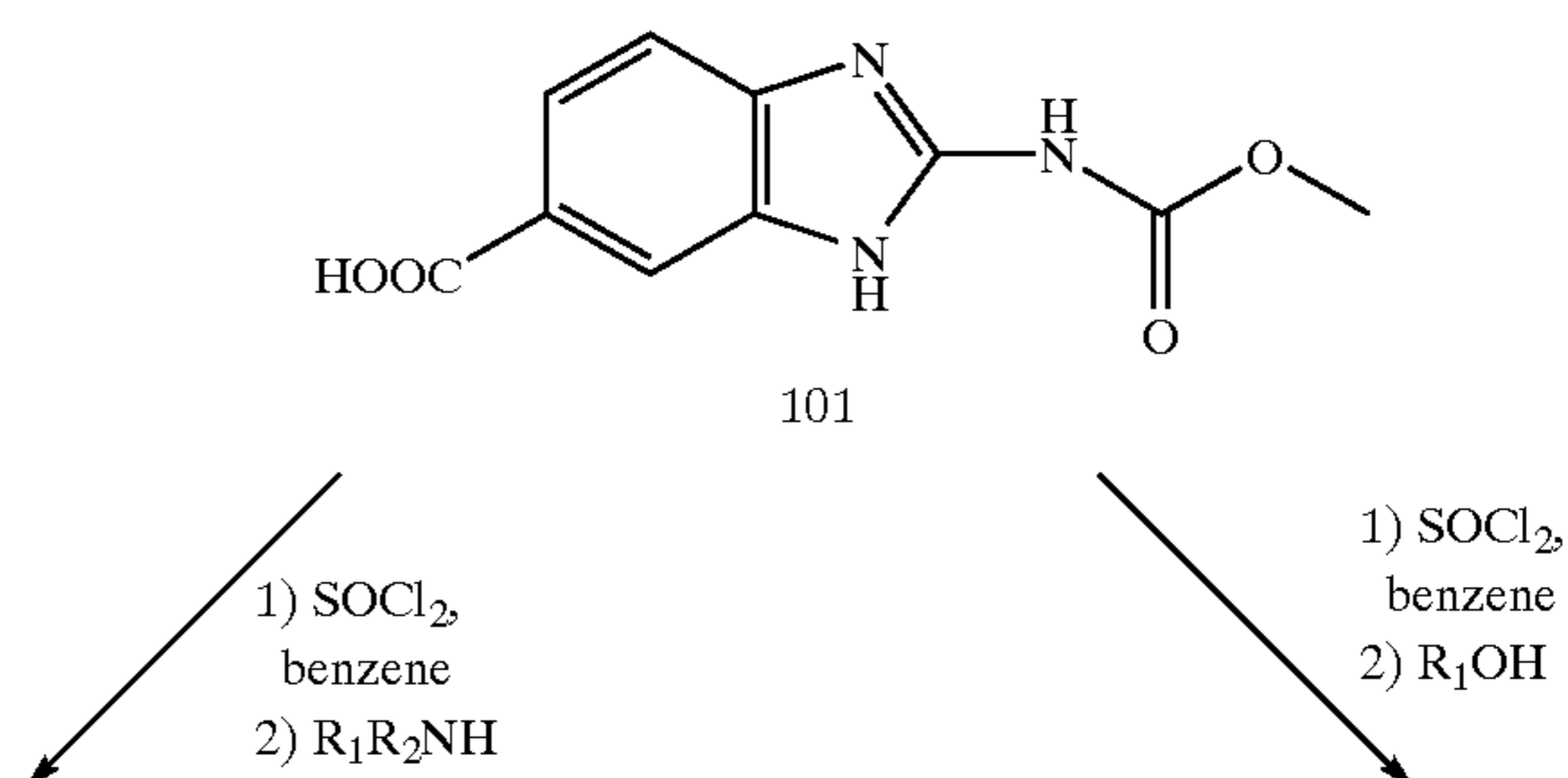
Reaction Scheme 1
