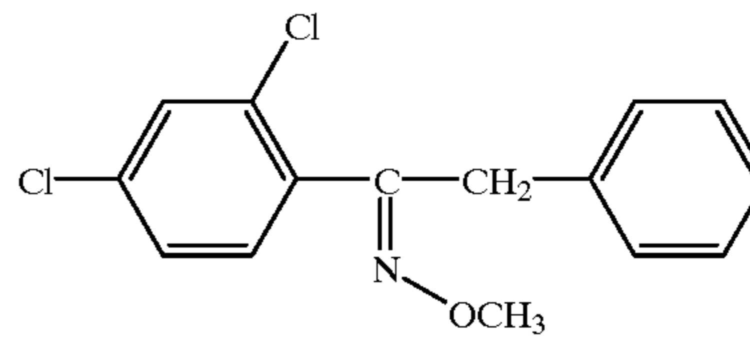
(PYRIFENOX)
