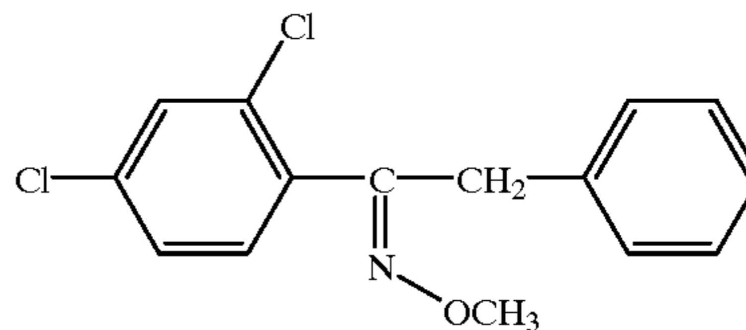
(PYRIFENOX)
