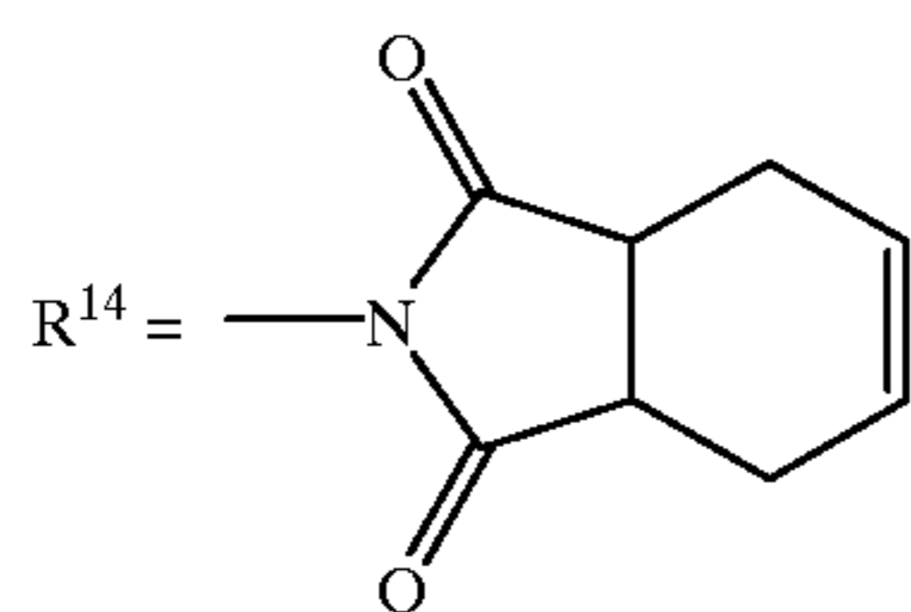
(CAPTAN)
