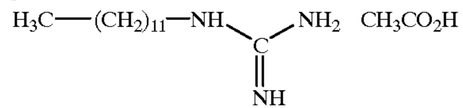
(DODINE)
