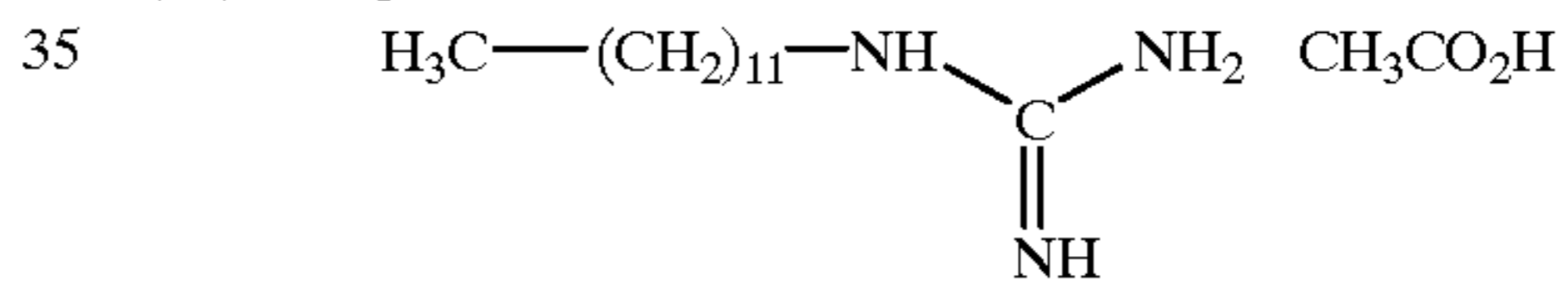
(DODINE)
