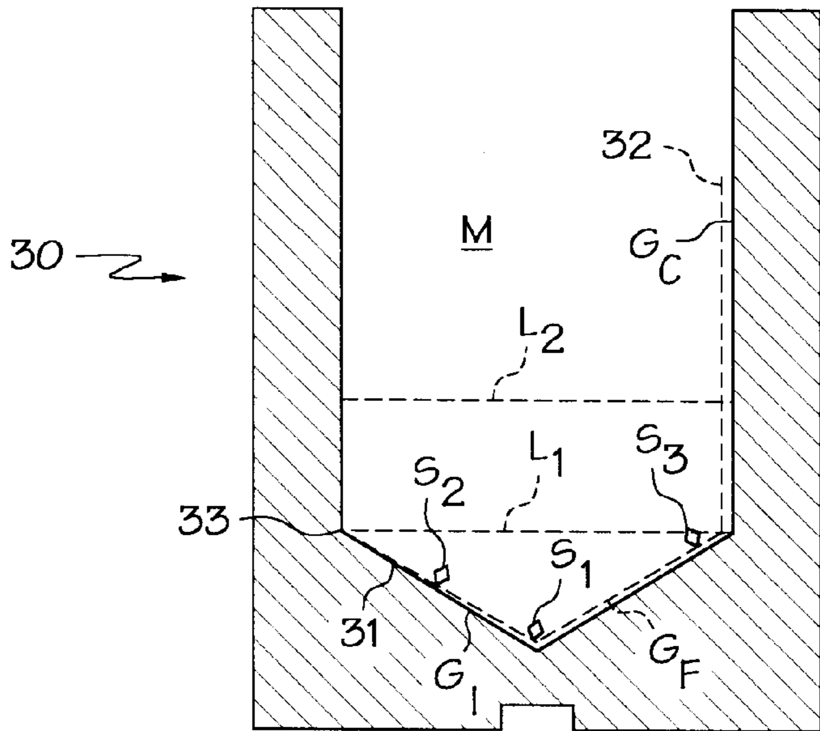
FIG. 2 PRIOR ART
