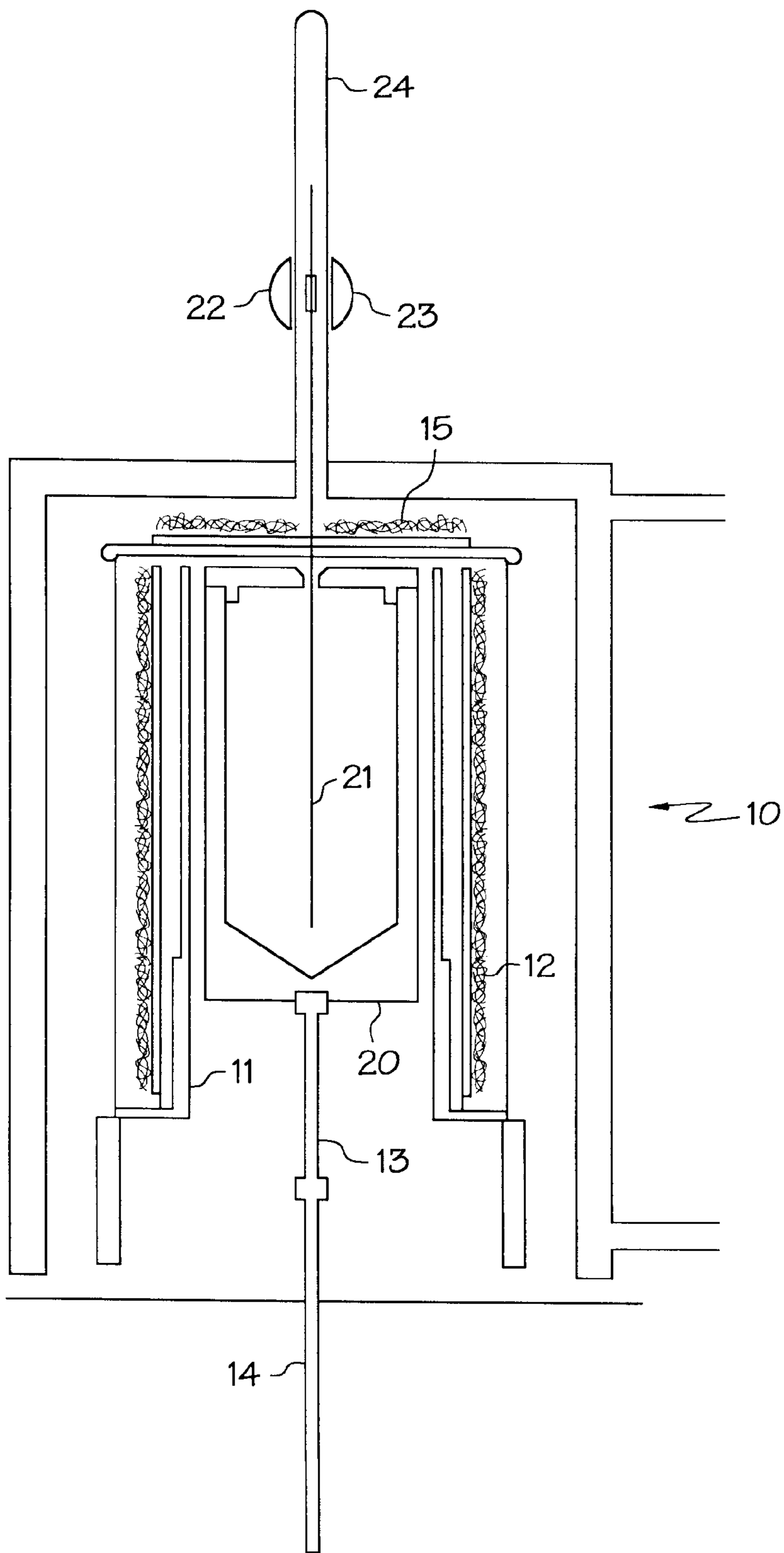
FIG. 1 PRIOR ART
