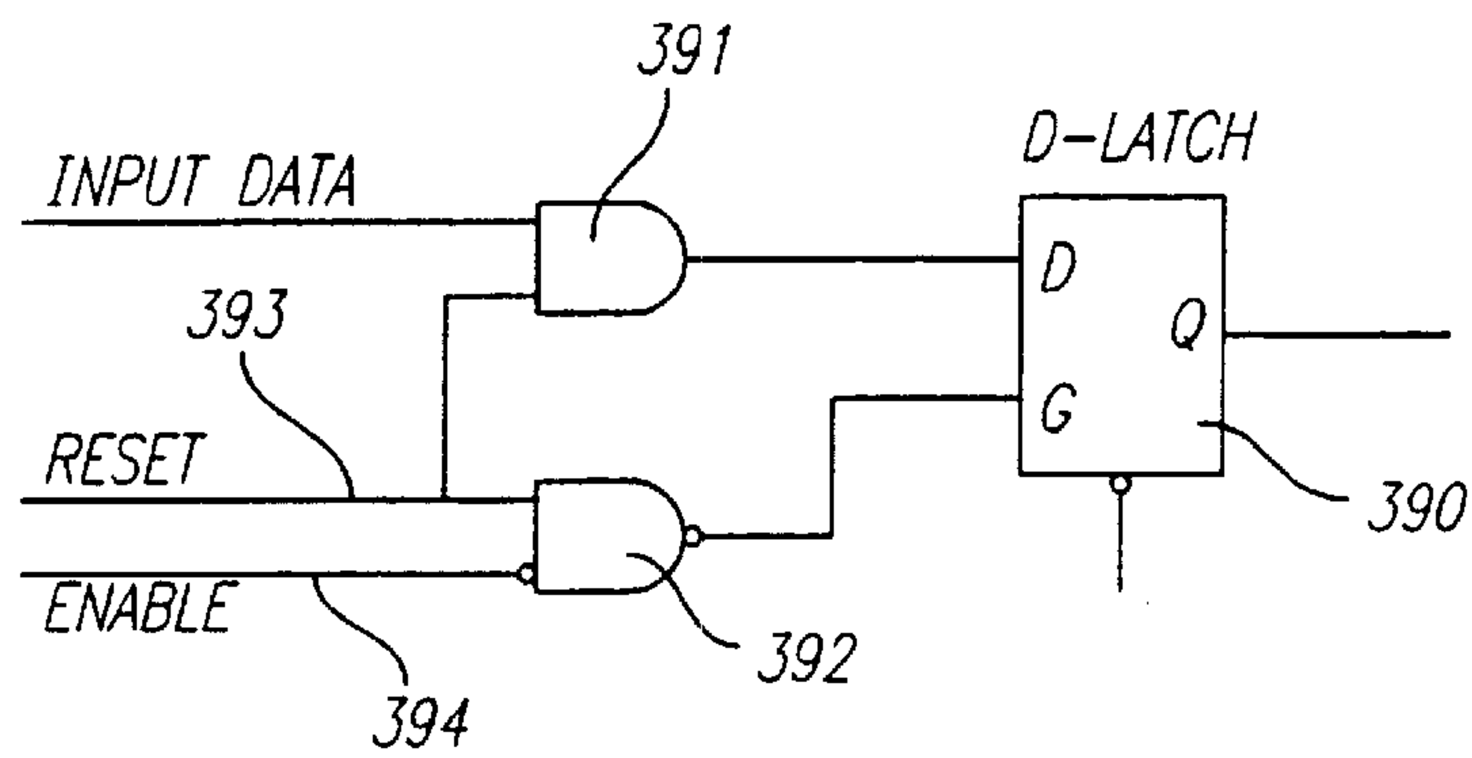
FIG. 37 FAILING IMPLEMENTATION OF A LATCH WITH CLEAR
