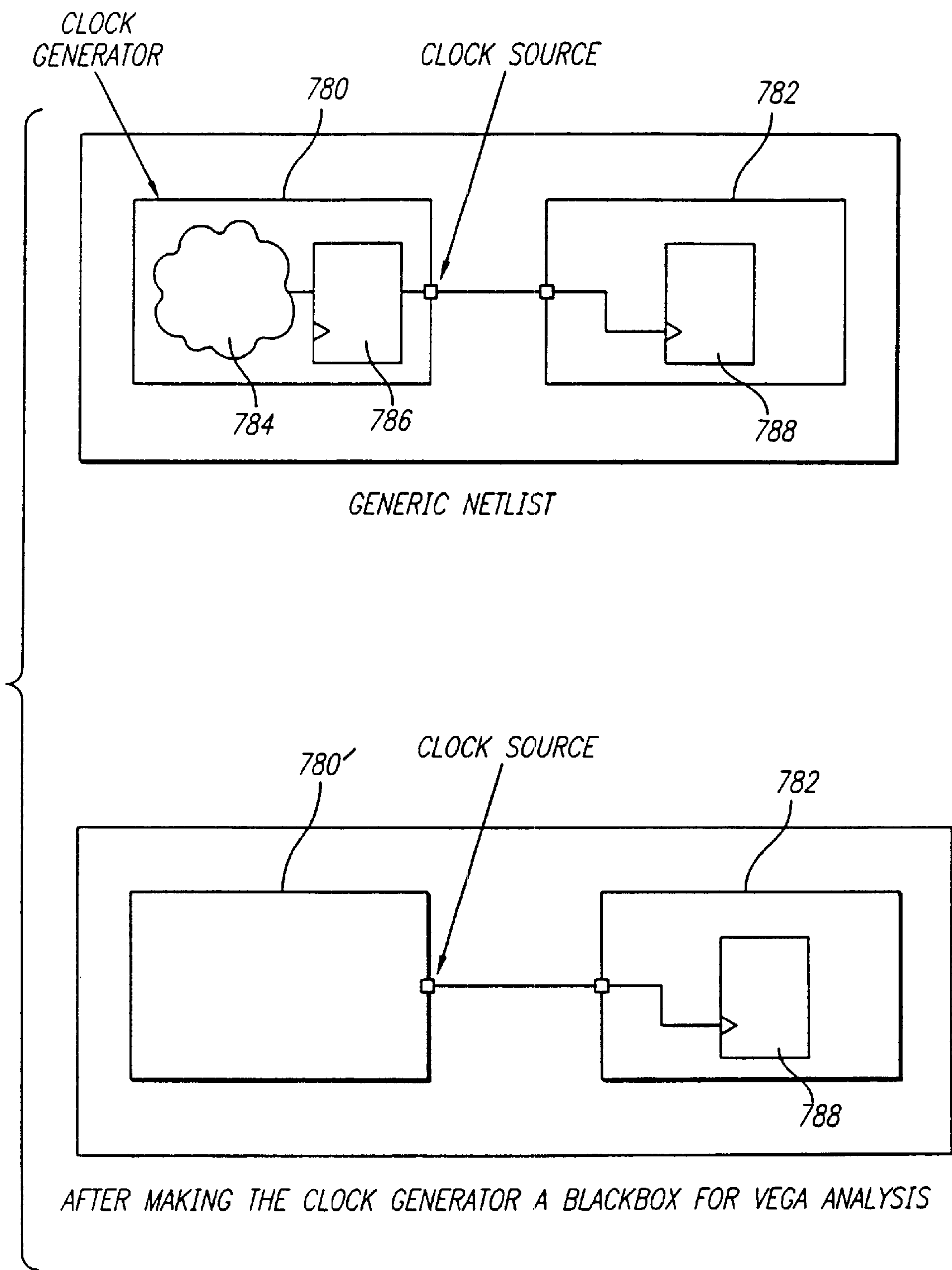
FIG. 43 HANDLING CLOCK GENERATORS WITH A "BACKBOX_DESIGN" DIRECTIVE.
