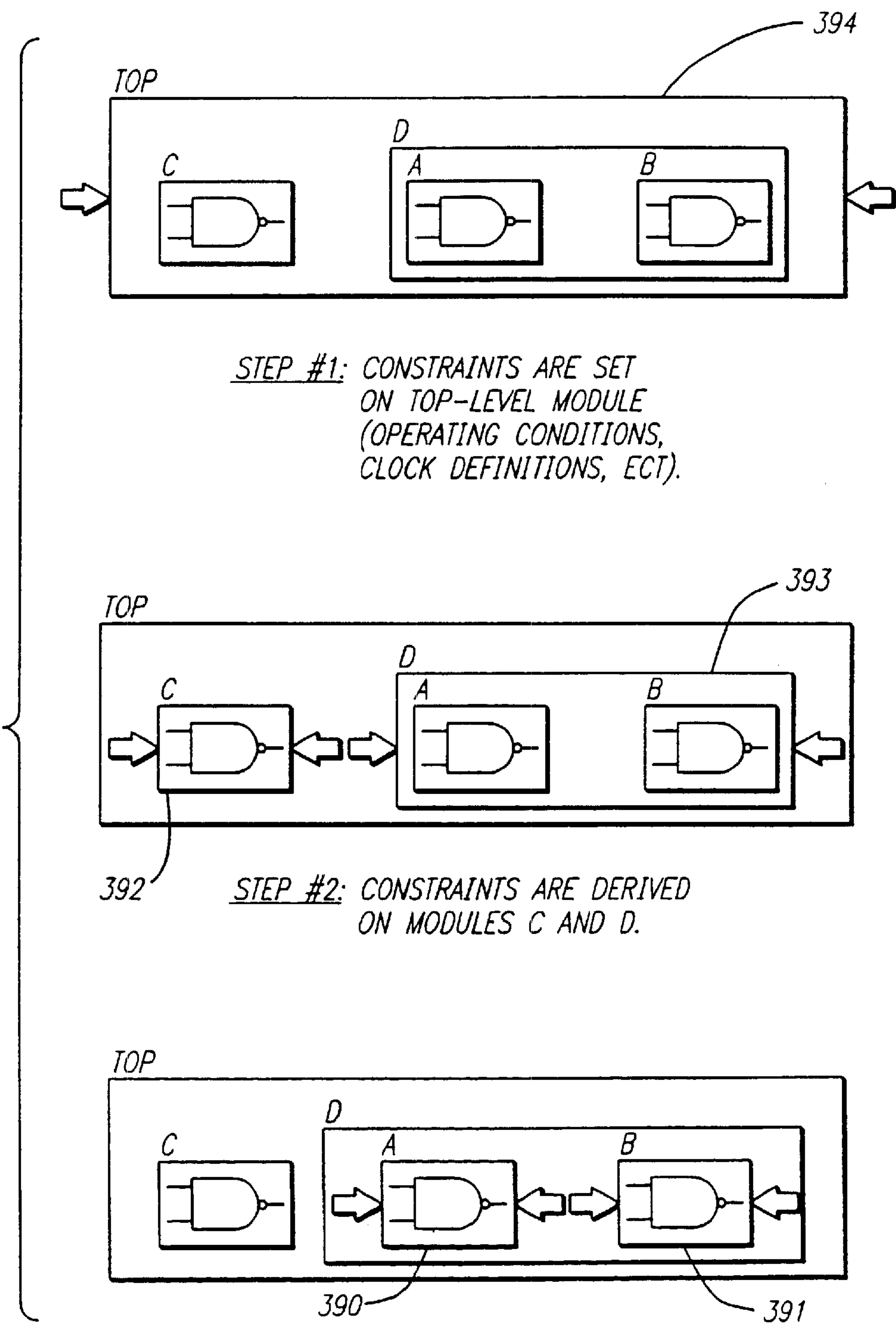
FIG. 16 TOP-DOWN CHARACTERIZATION
