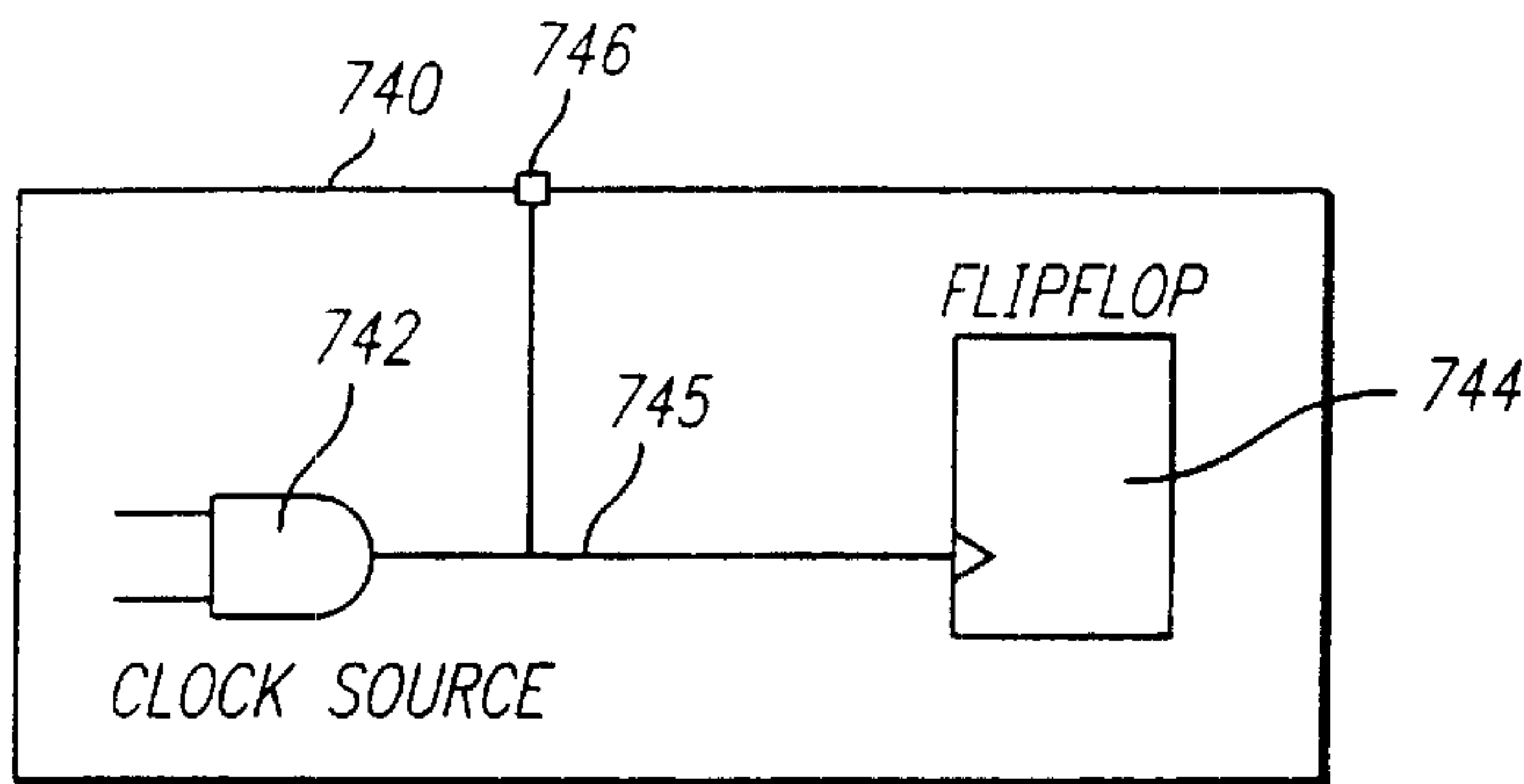
FIG. 41A CLOCK SOURCE RETRIEVED THROUGH USING A CONNECTED PORT
