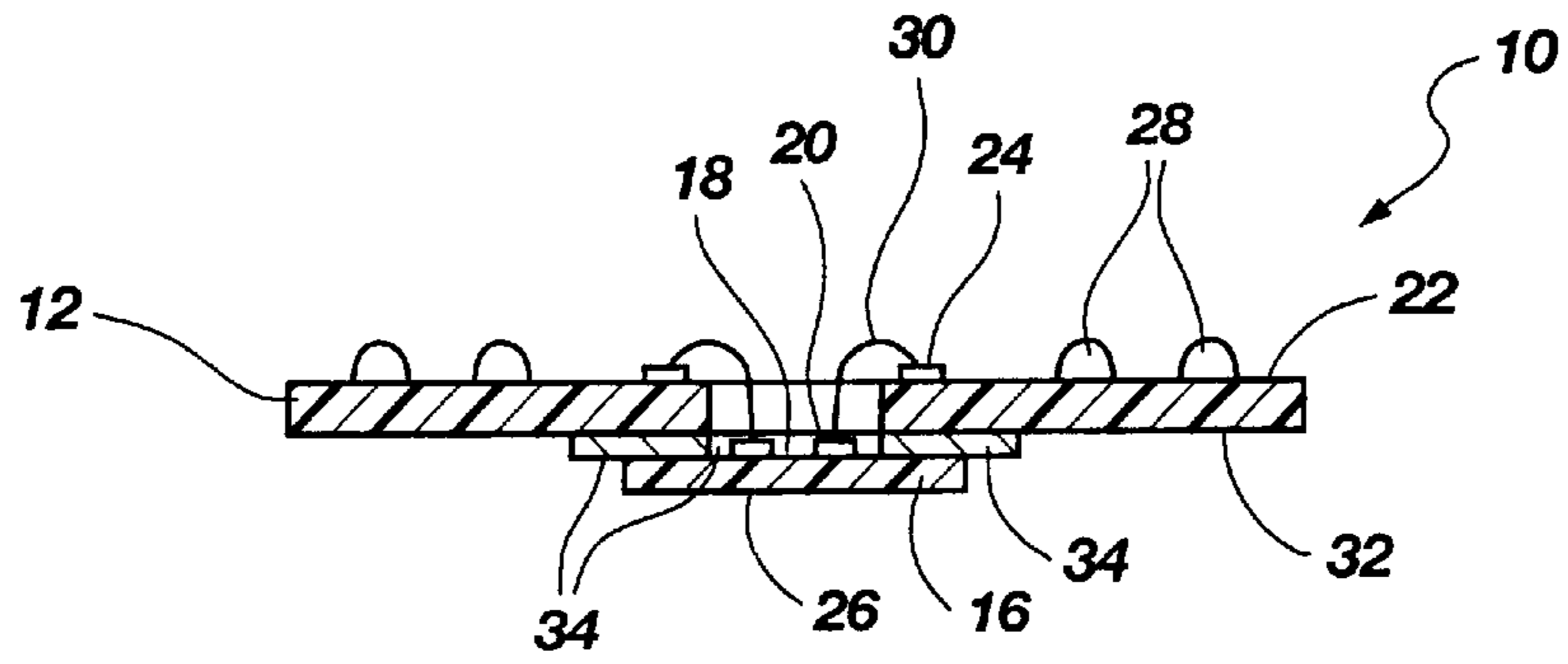
Fig. 2 (PRIOR ART)
