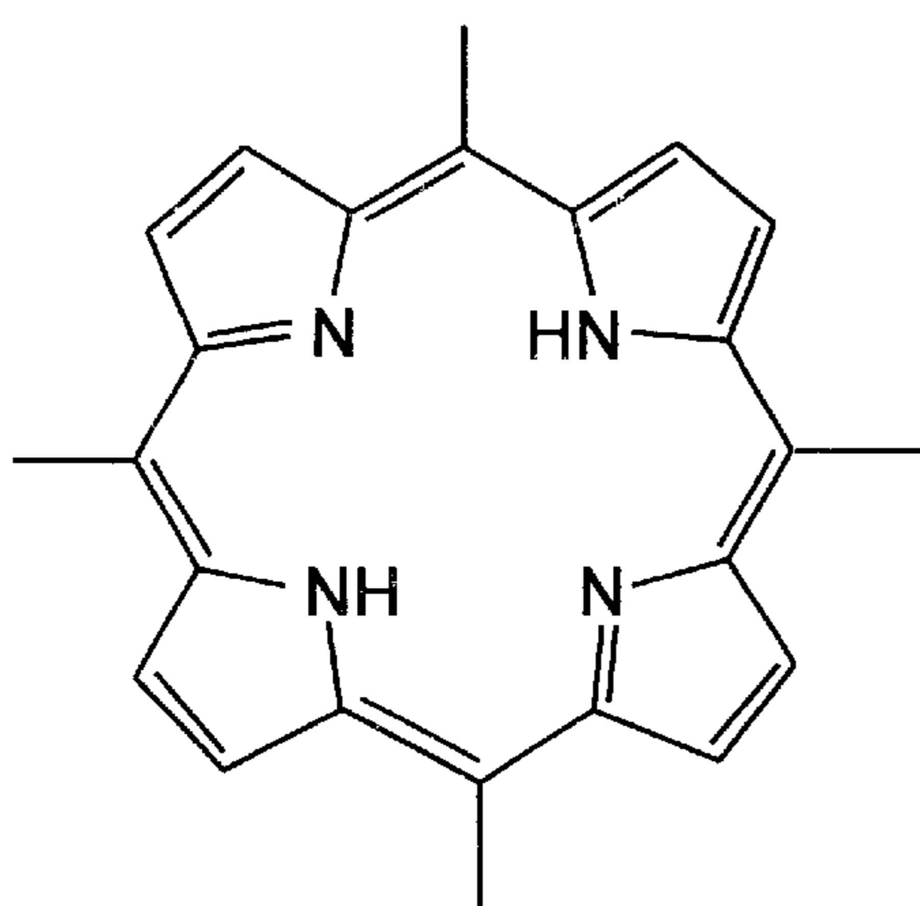
A MESO-SUBSTITUTED PORPHYRIN
