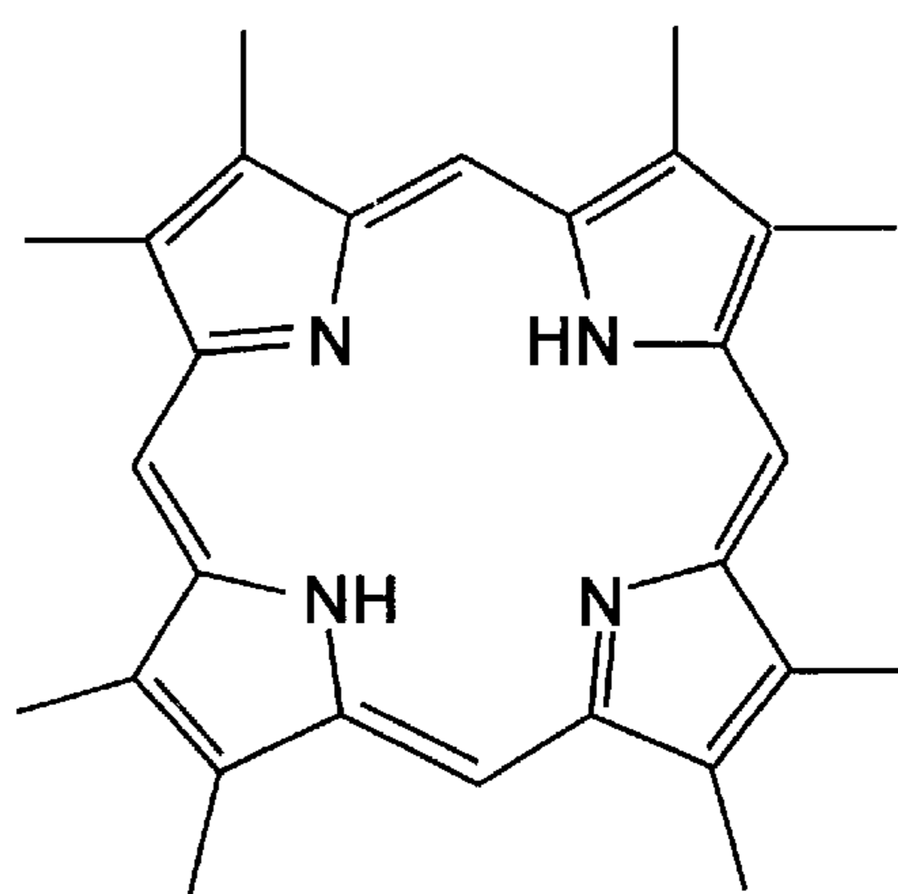
A \beta -SUBSTITUTED PORPHYRIN
