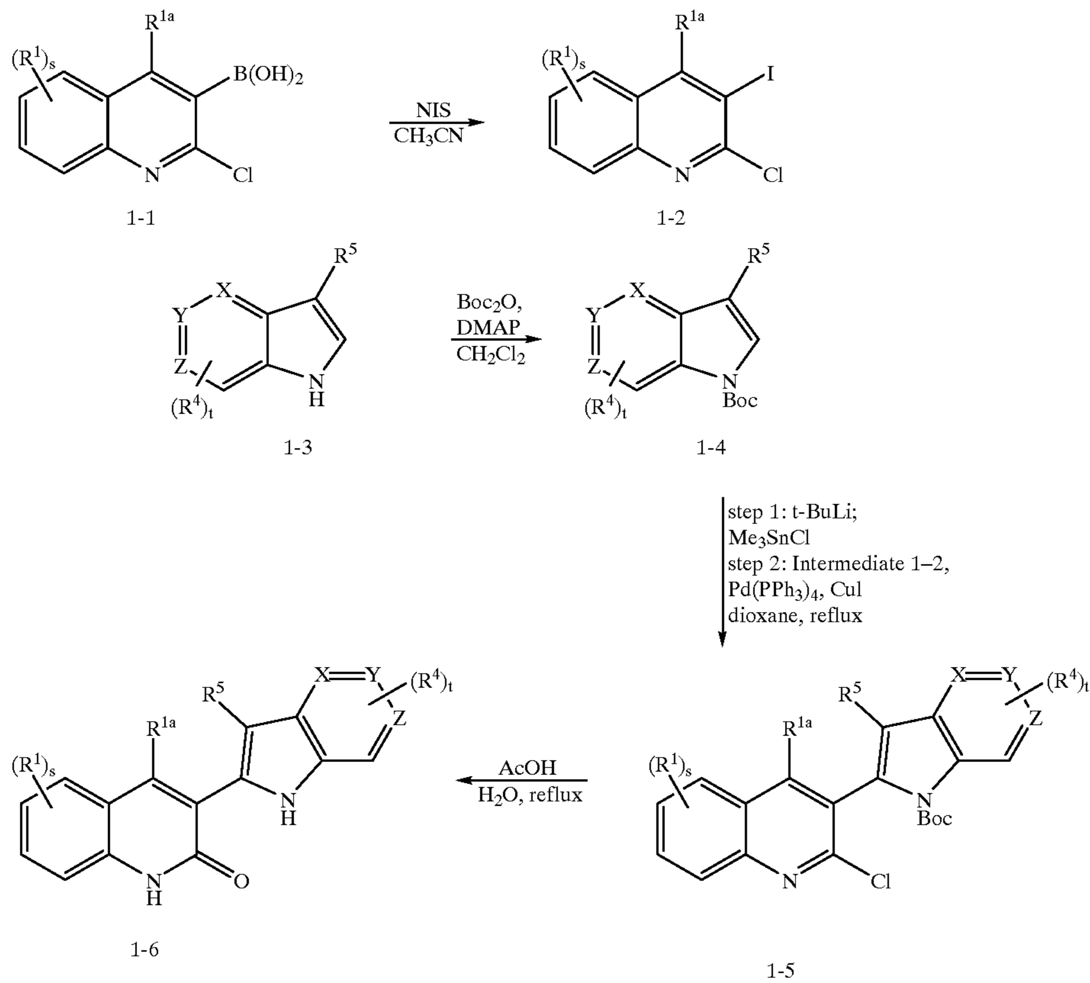
SCHEME 1
