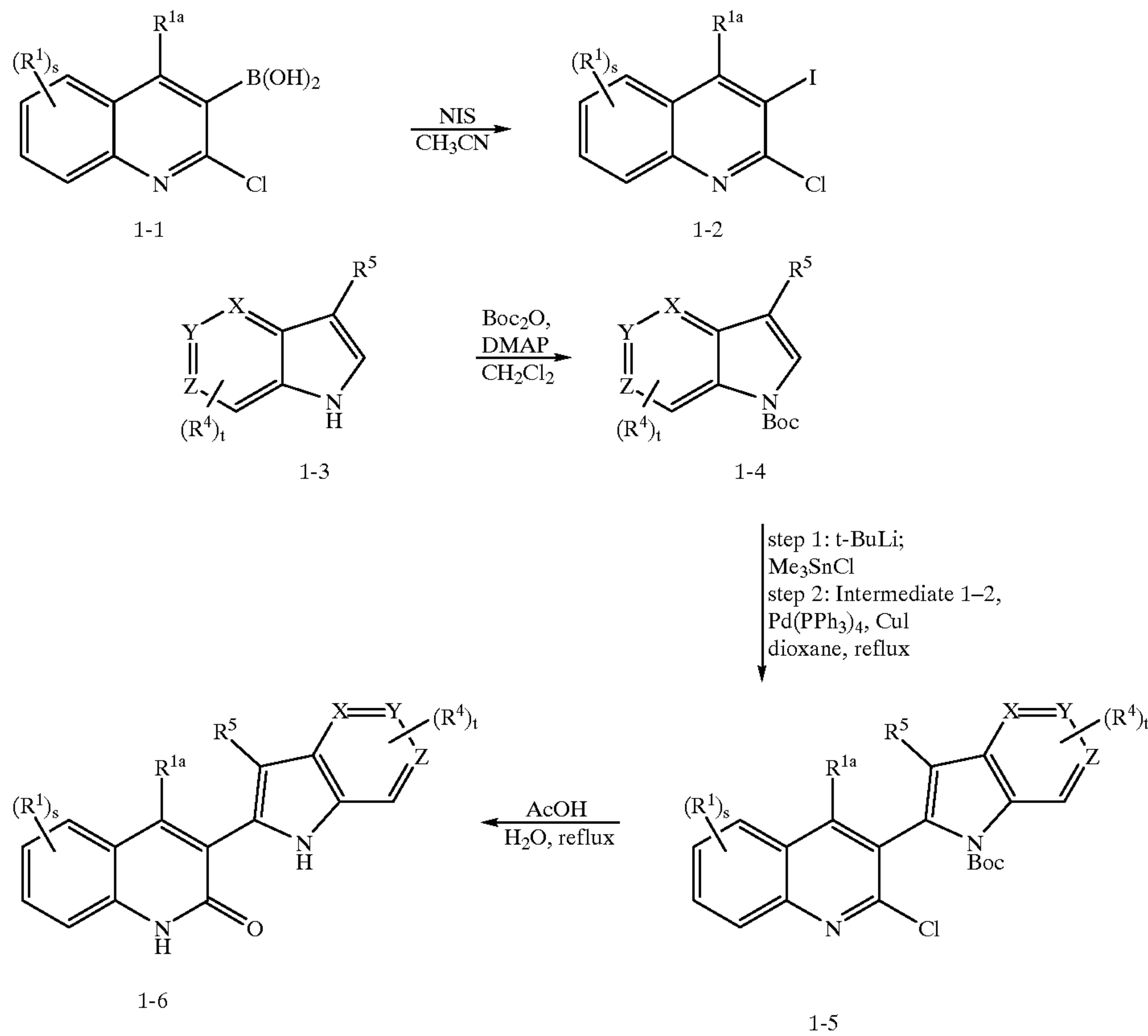
SCHEME 1
