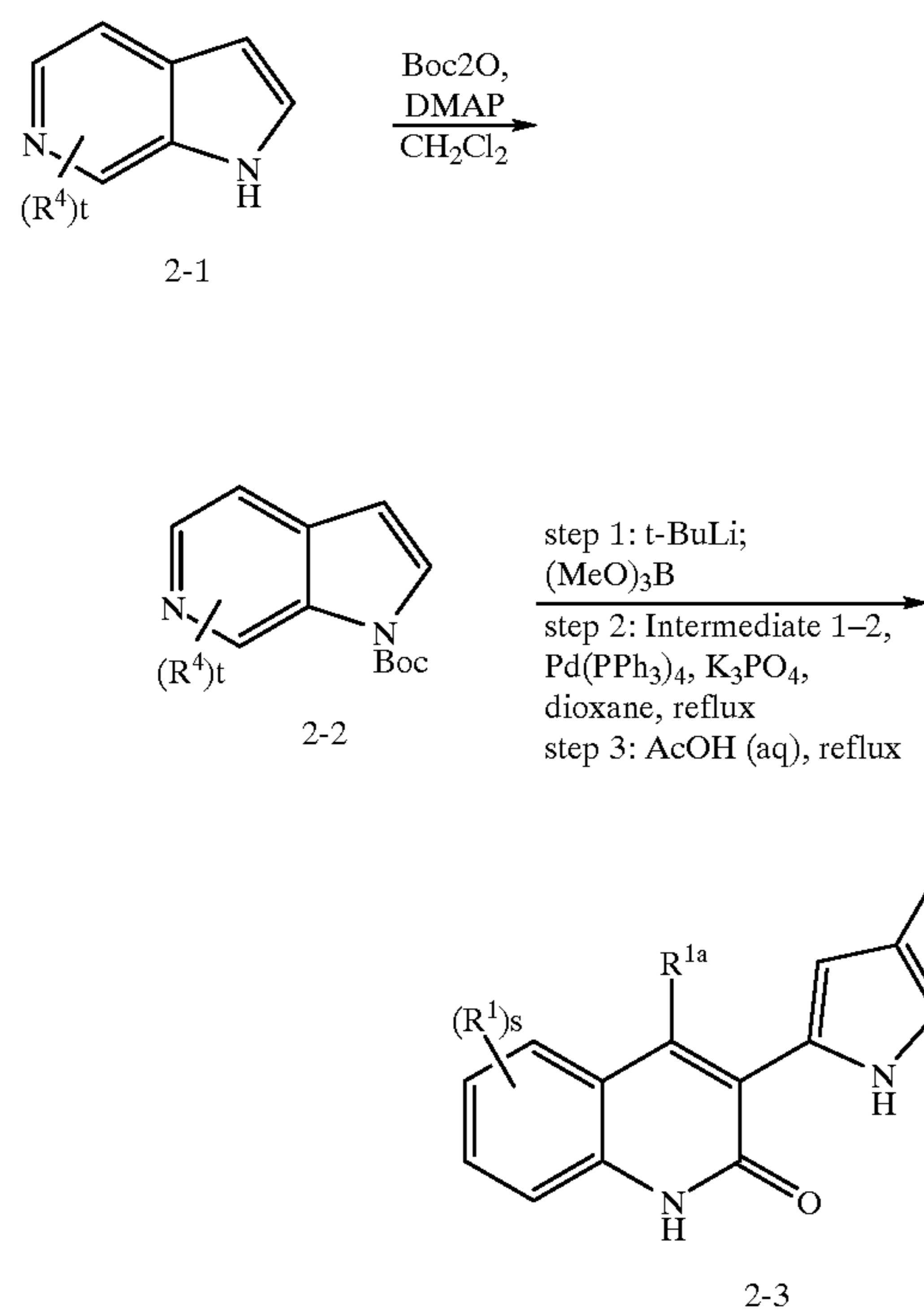
SCHEME 2
