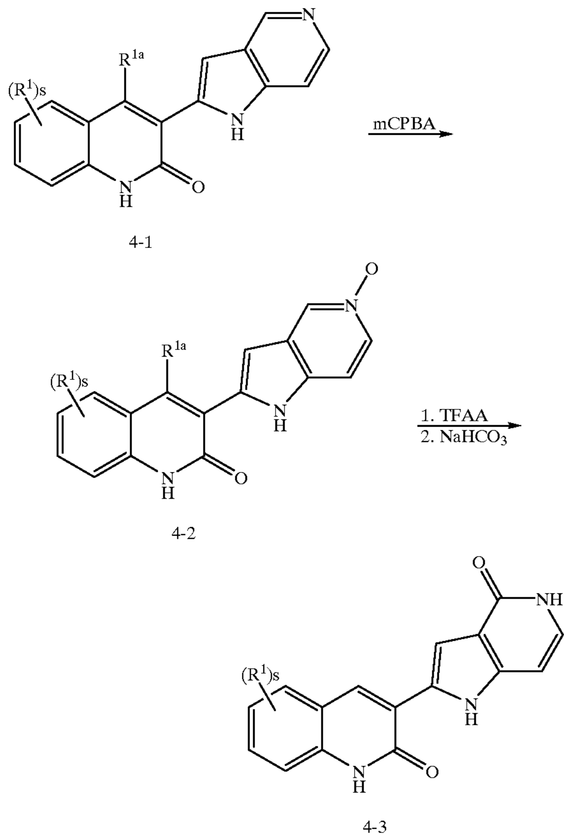
SCHEME 4
