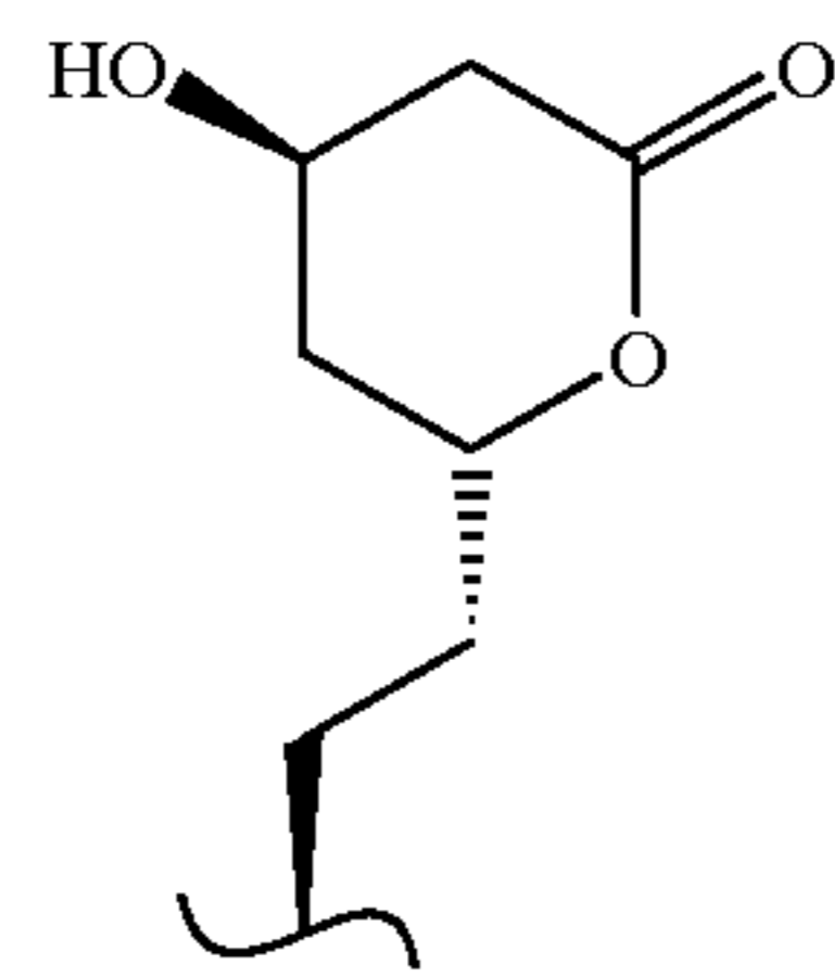
Lactone
