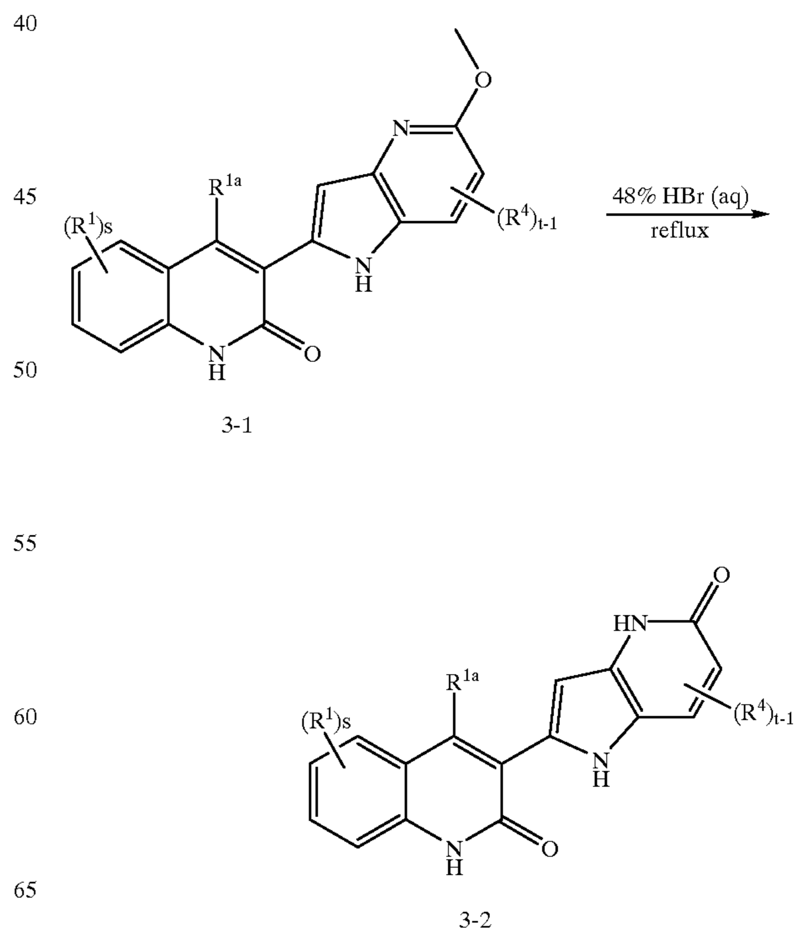
SCHEME 3
