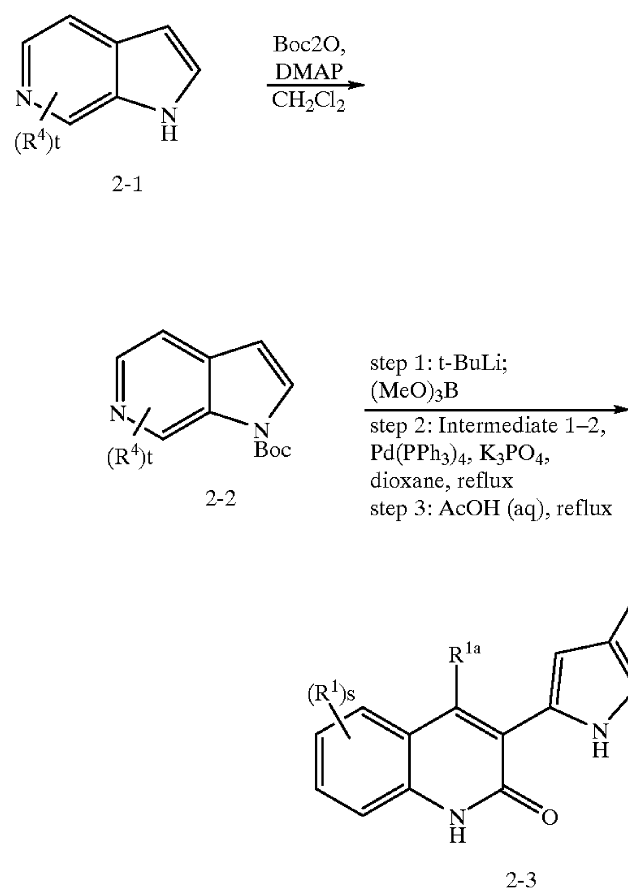
SCHEME 2
