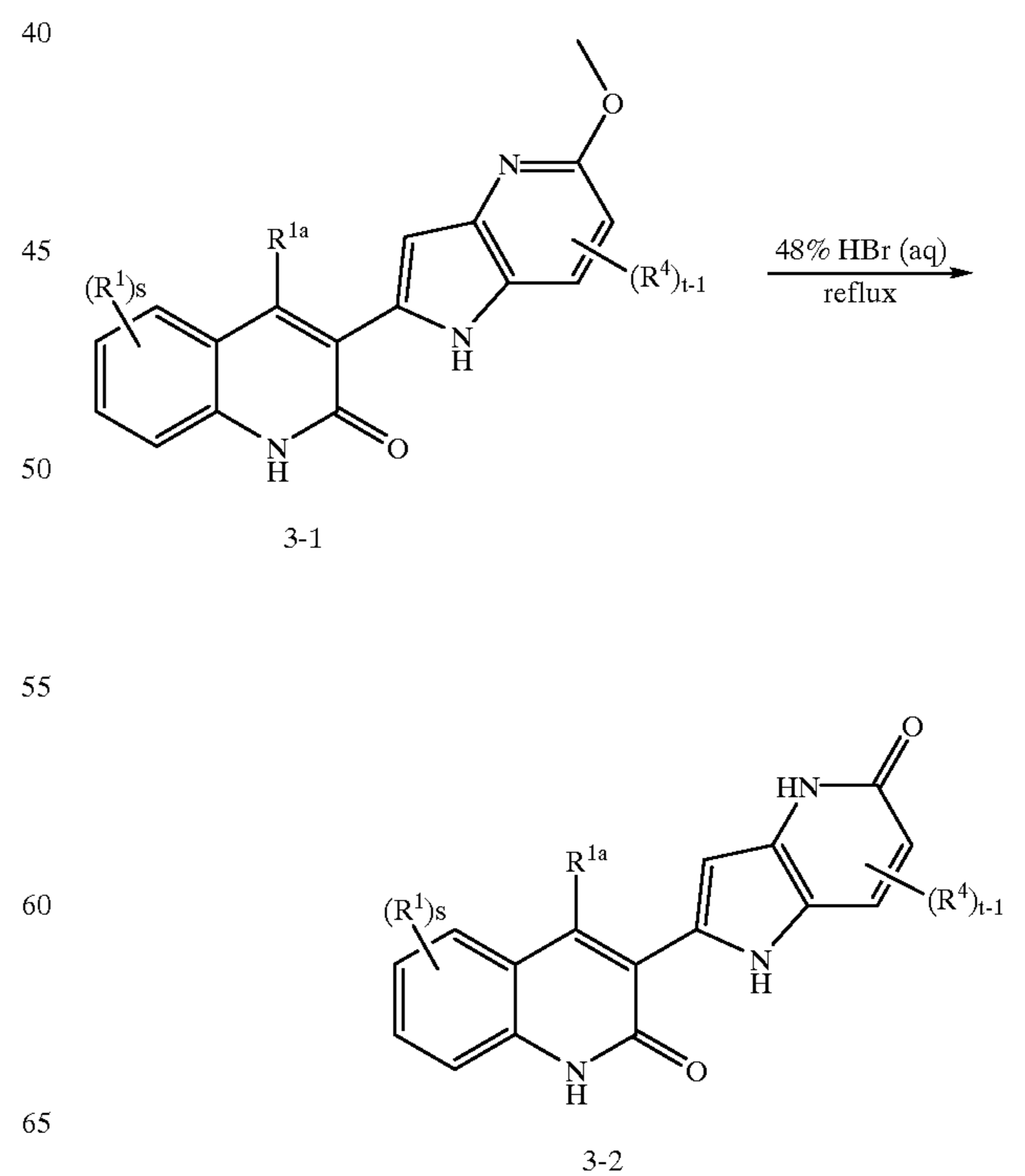
SCHEME 3
