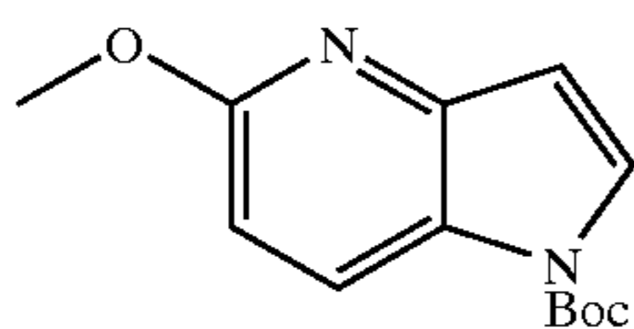
Intermediate B
