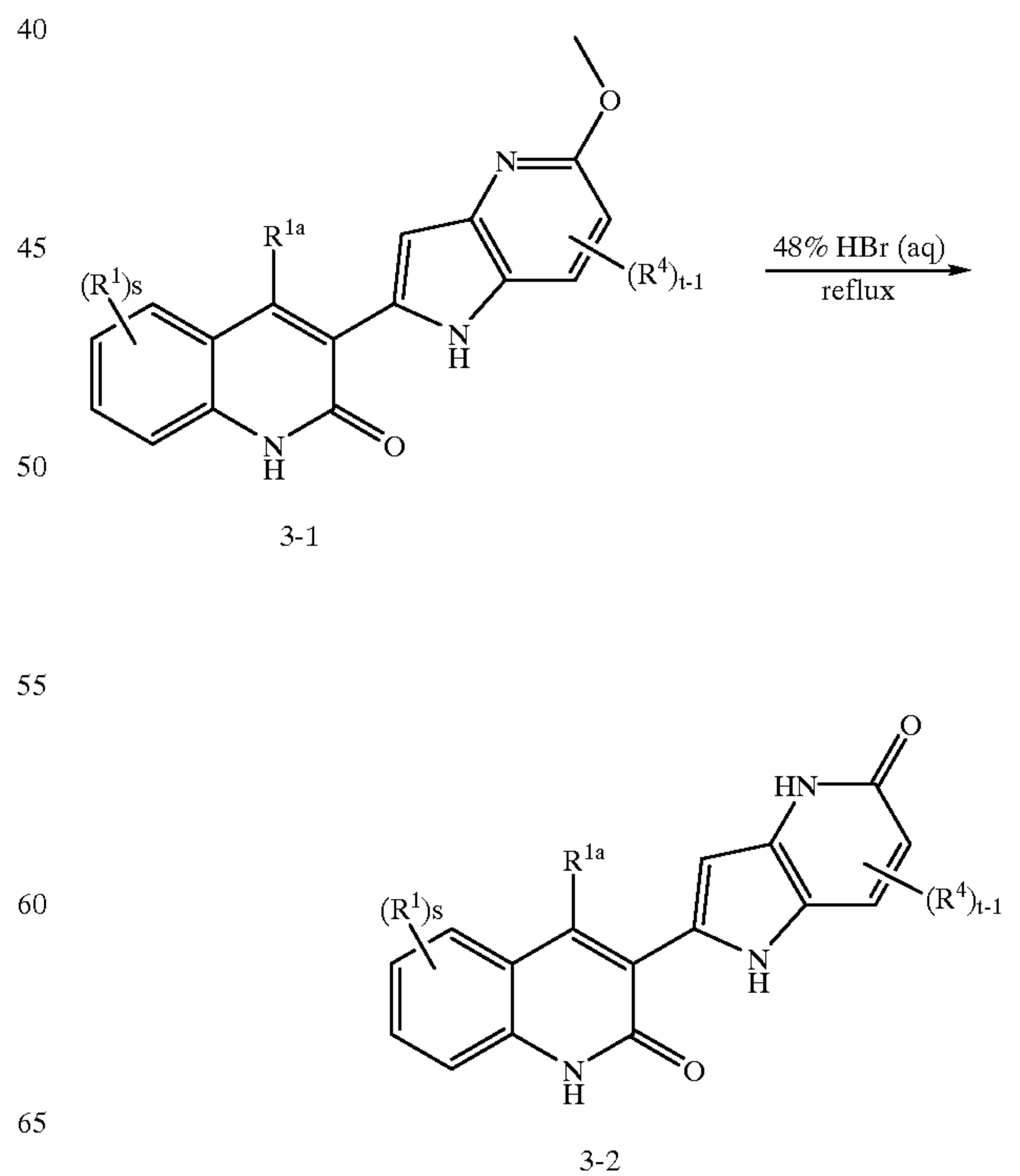
SCHEME 3
