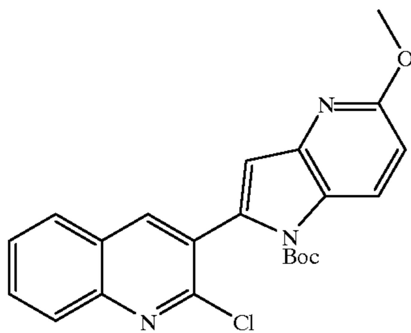
Intermediate C
