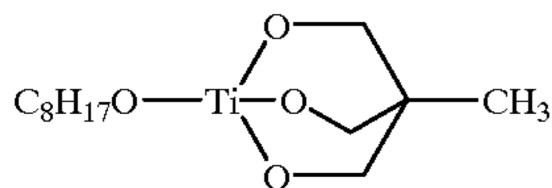
1-(2-ethyl-1-hexoxy)-4-methyl-2,6,7-trioxo-1-titanabicyclo[2,2,2]octane
