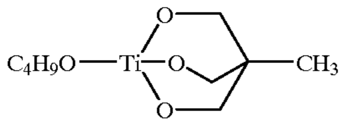
1-(1-Butoxy)-4-methyl-2,6,7-trioxo-1-titanabicyclo[2,2,2]octane
