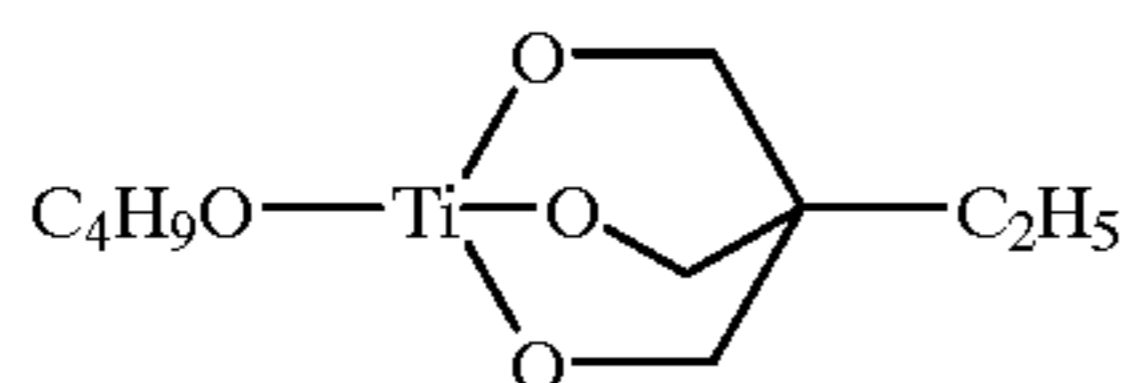
1-(1-Butoxy)-4-ethyl-2,6,7-trioxo-1-titanabicyclo[2,2,2]octane
