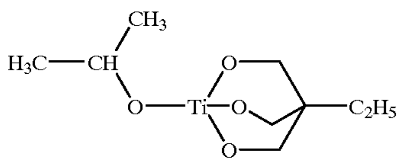
1-(2-Propoxy)-4-ethyl-2,6,7-trioxo-1-titanabicyclo[2,2,2]octane
