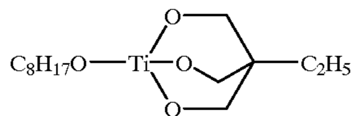
1-(2-ethyl-1-hexoxy)-4-ethyl-2,6,7-trioxo-1-titanabicyclo[2,2,2]octane
