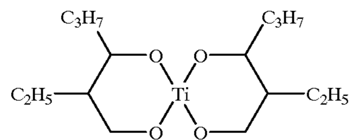
Bis(2-ethyl-1,3-hexylene) titanate
