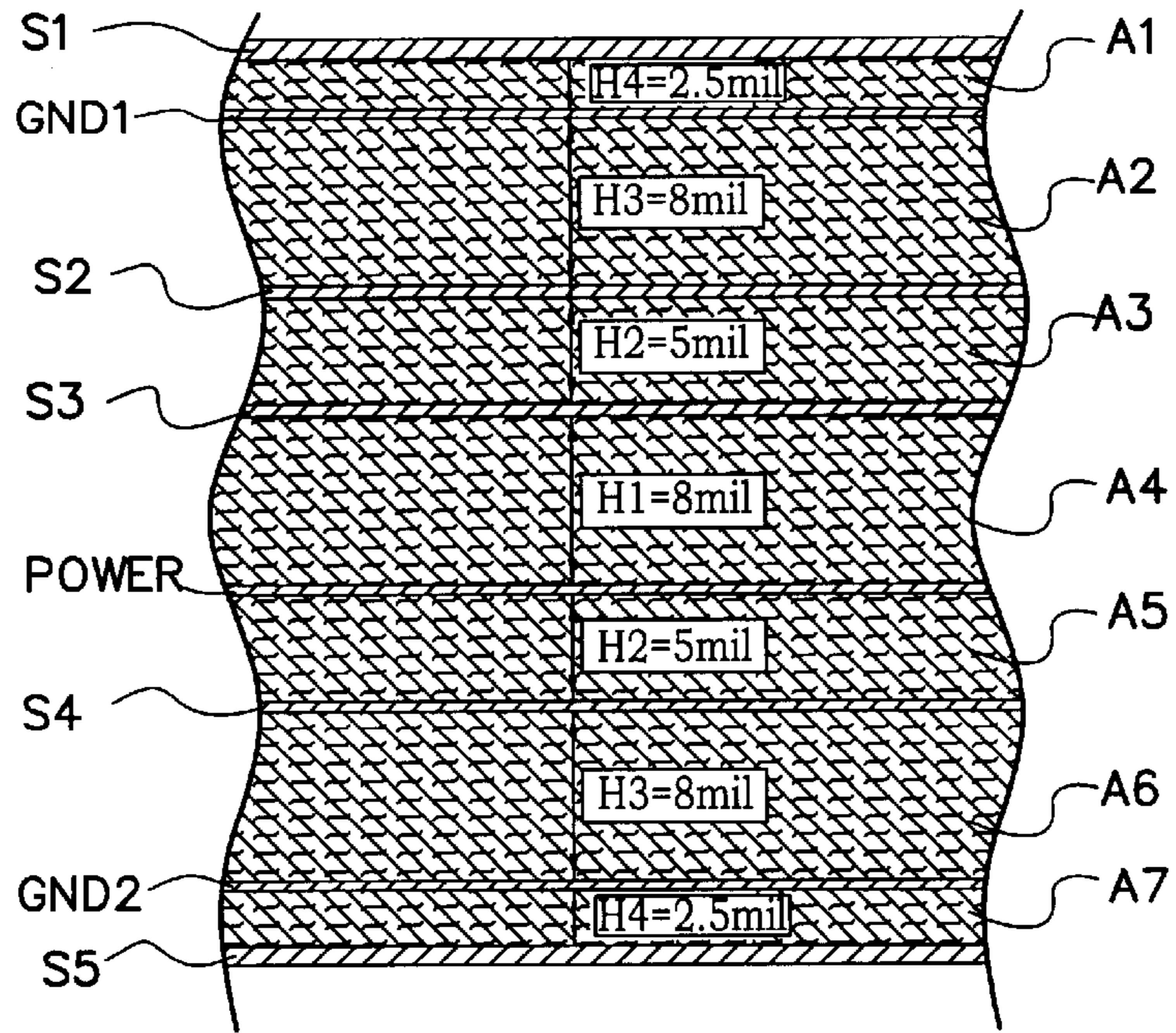
FIG. 1 (PRIOR ART)
