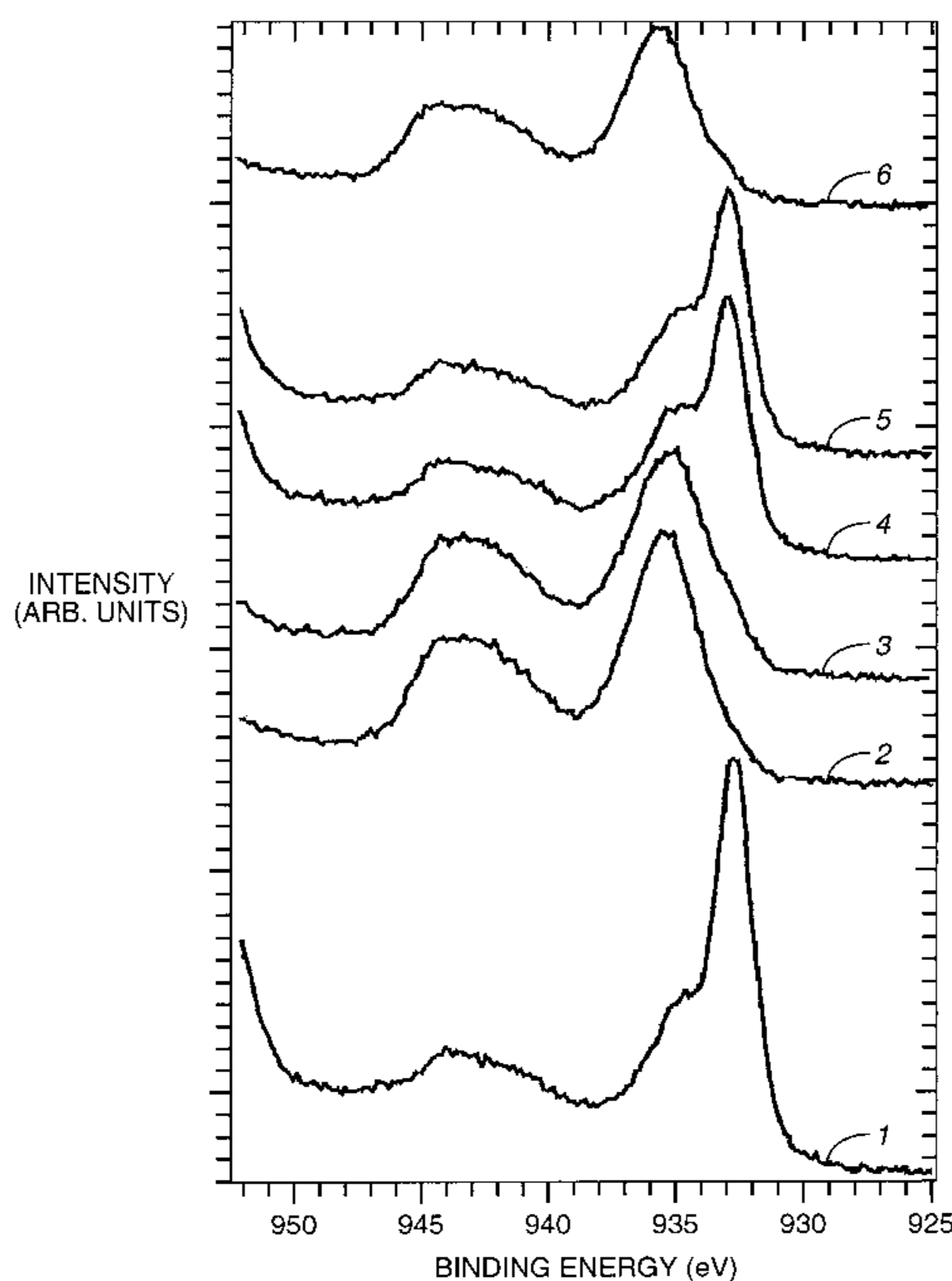
XPS ANALYSIS OF THE SURFACE COMPOSITION OF A COPPER BLANKET BEFORE (1), AFTER ETCHING (2 AND 3) AND AFTER CLEANING IN THE SOLUTION (4 AND 5) AND IN SOLUTION B8 (6).
