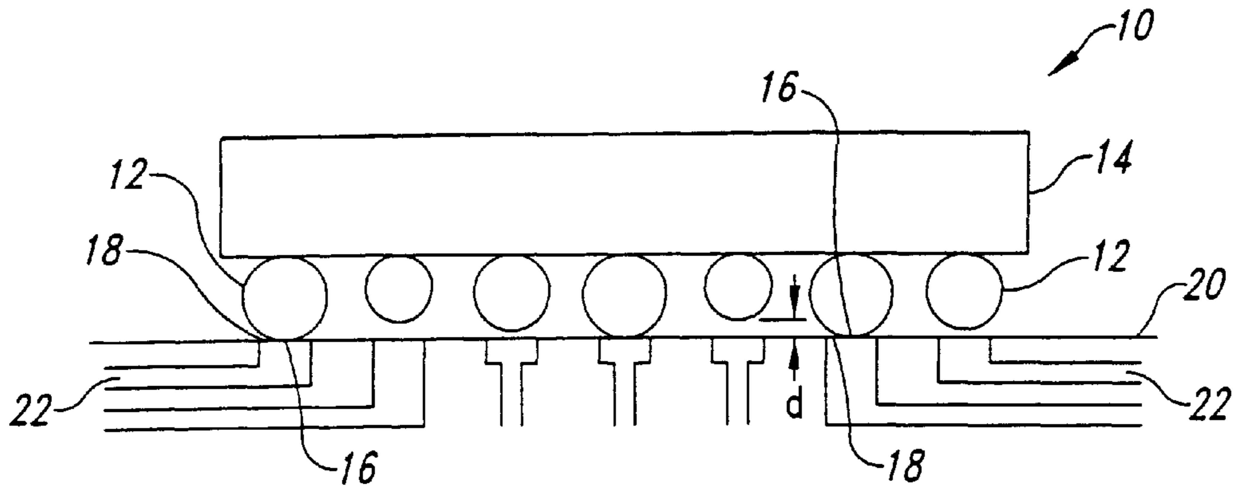
Fig. 1 (Prior Art)
