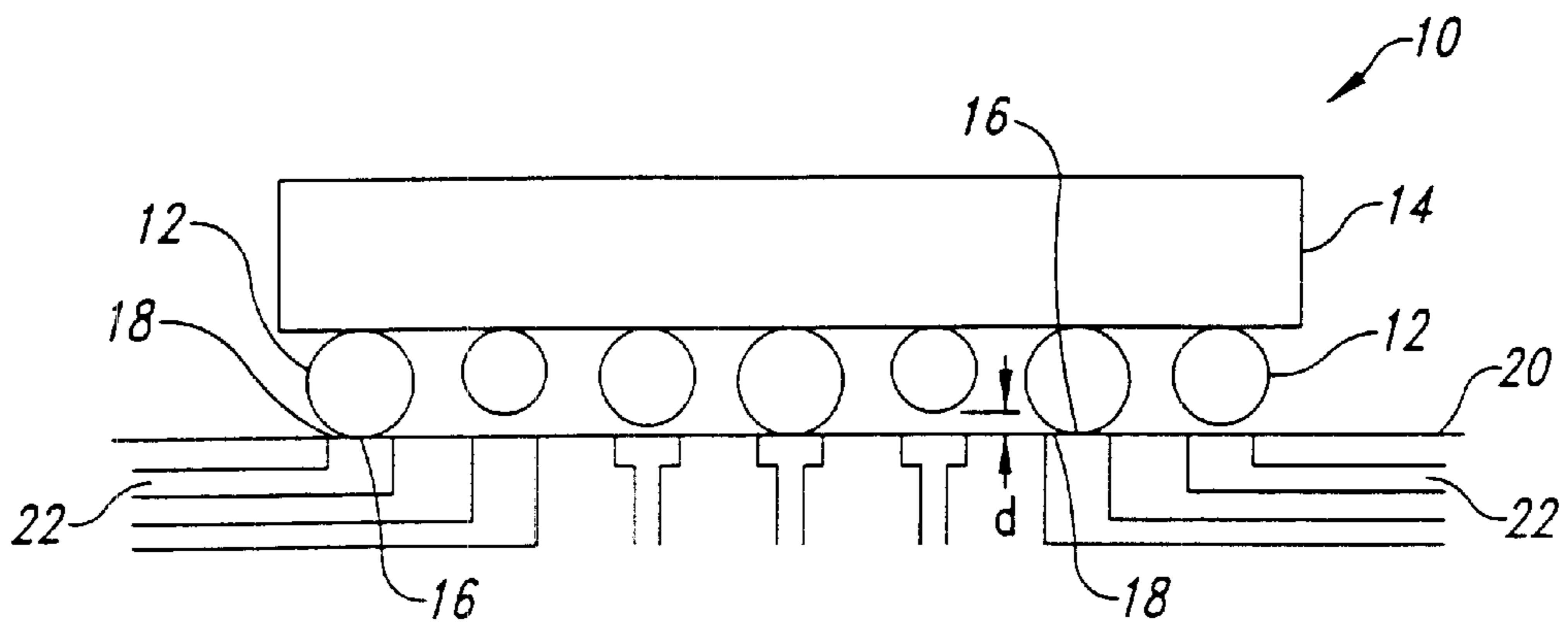
Fig. 1 (Prior Art)
