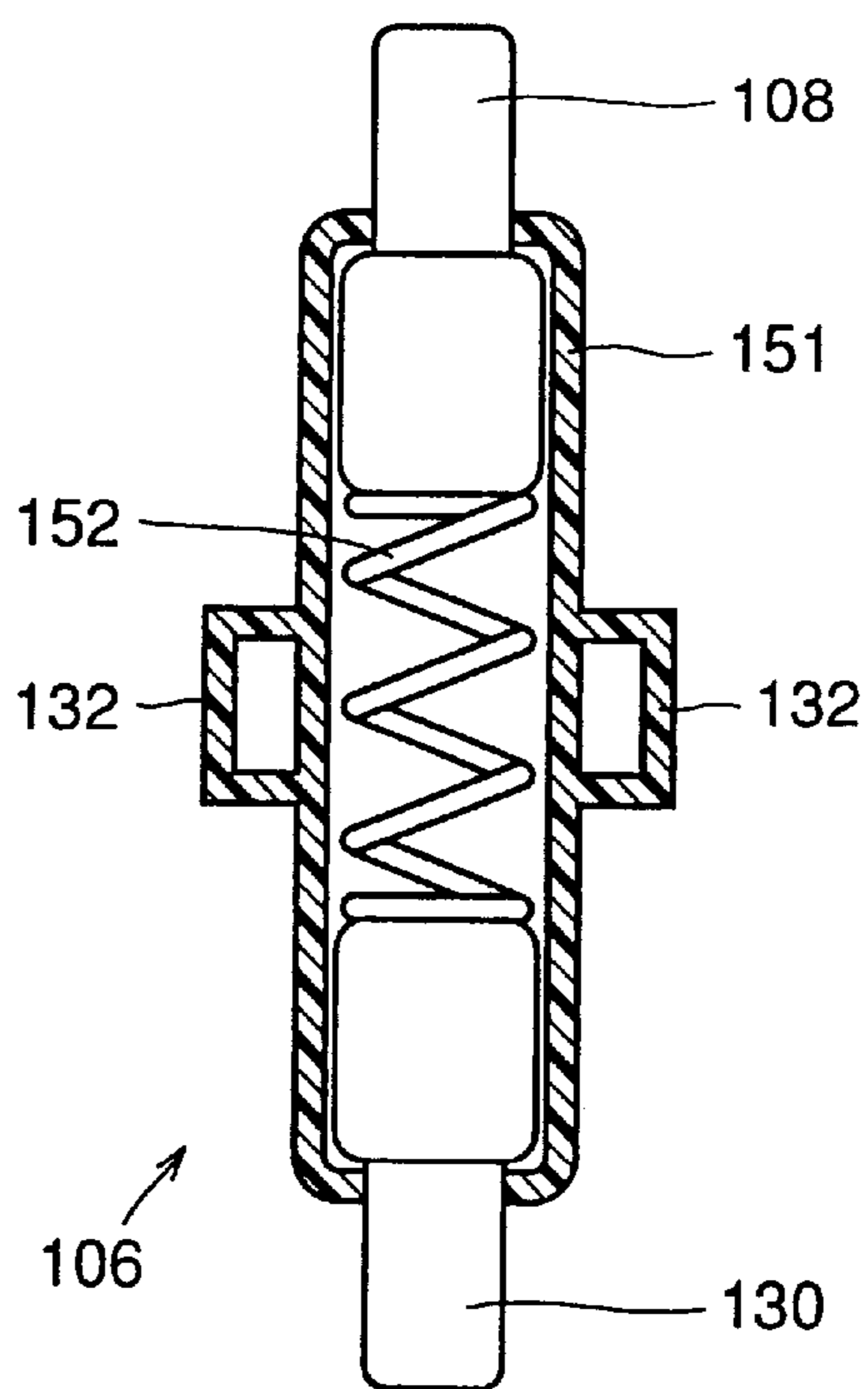
FIG. 13 PRIOR ART
