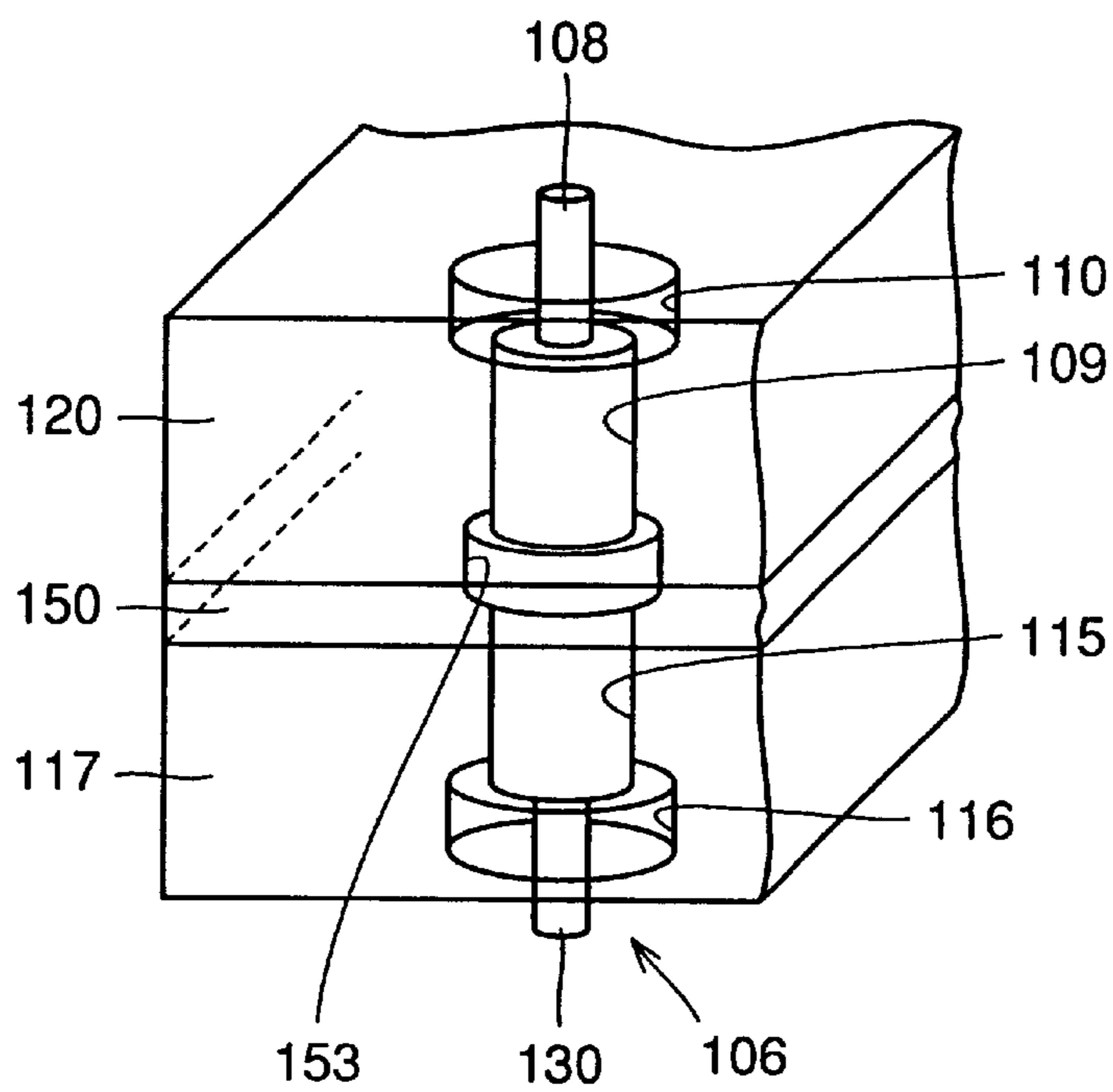
FIG. 14 PRIOR ART
