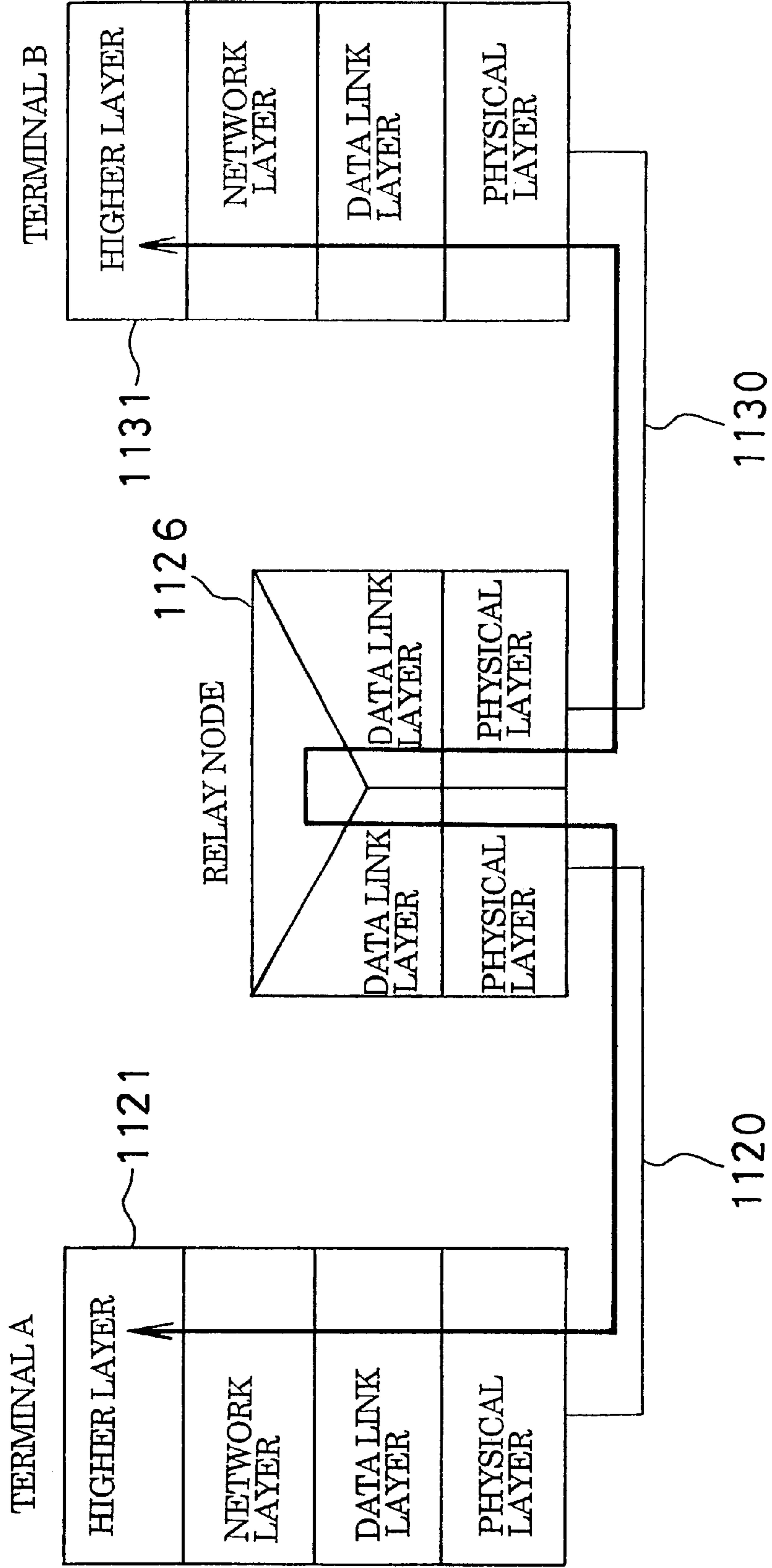
FIG. 11 PRIOR ART
