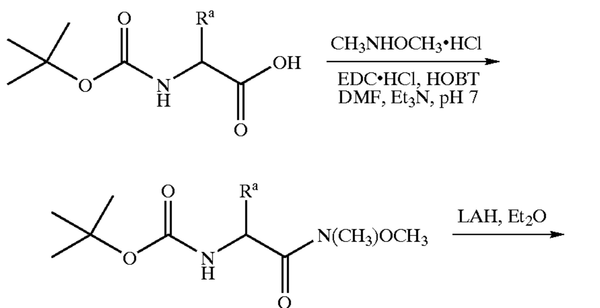
SCHEME 11
