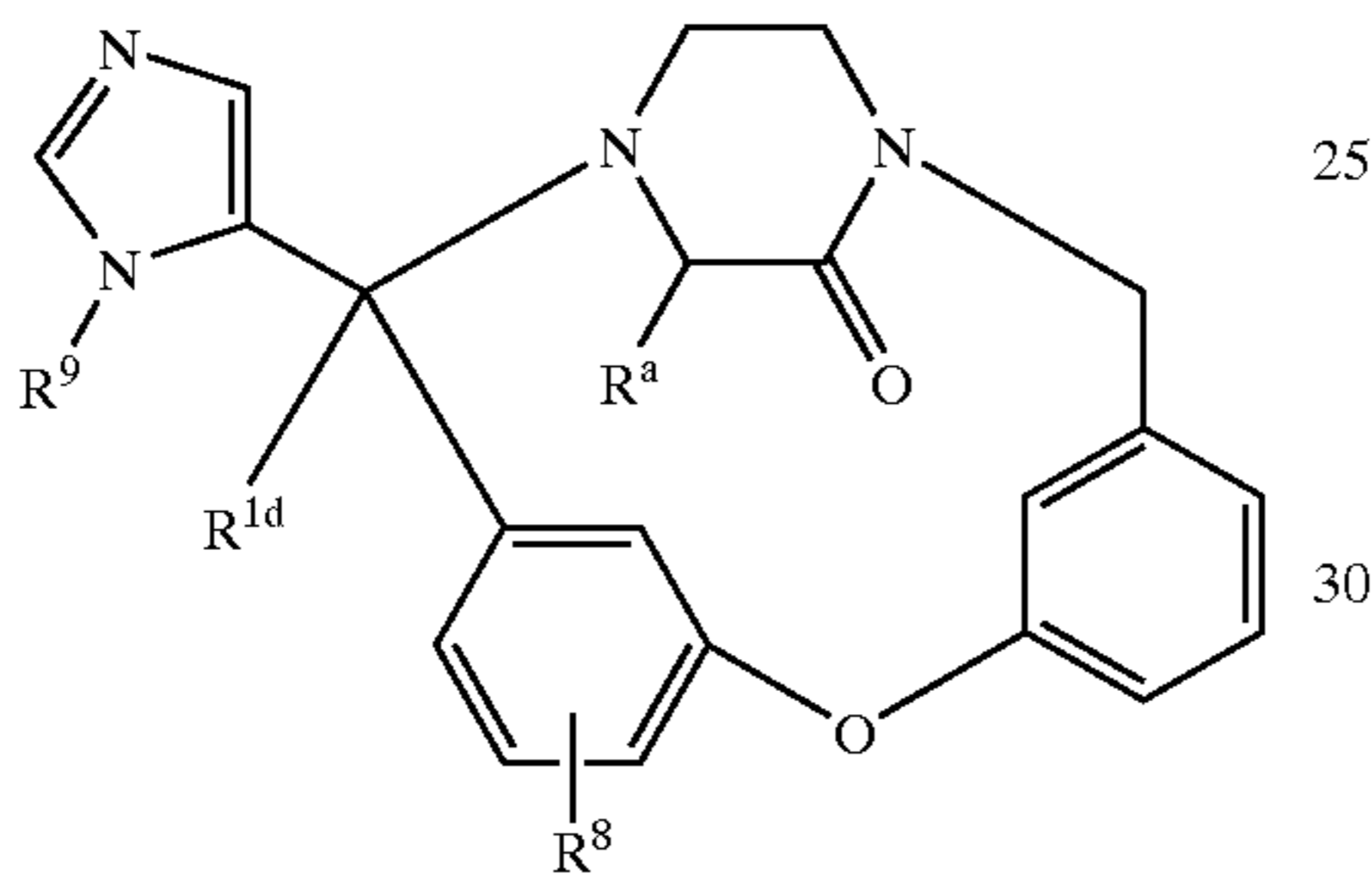
SCHEME 9
