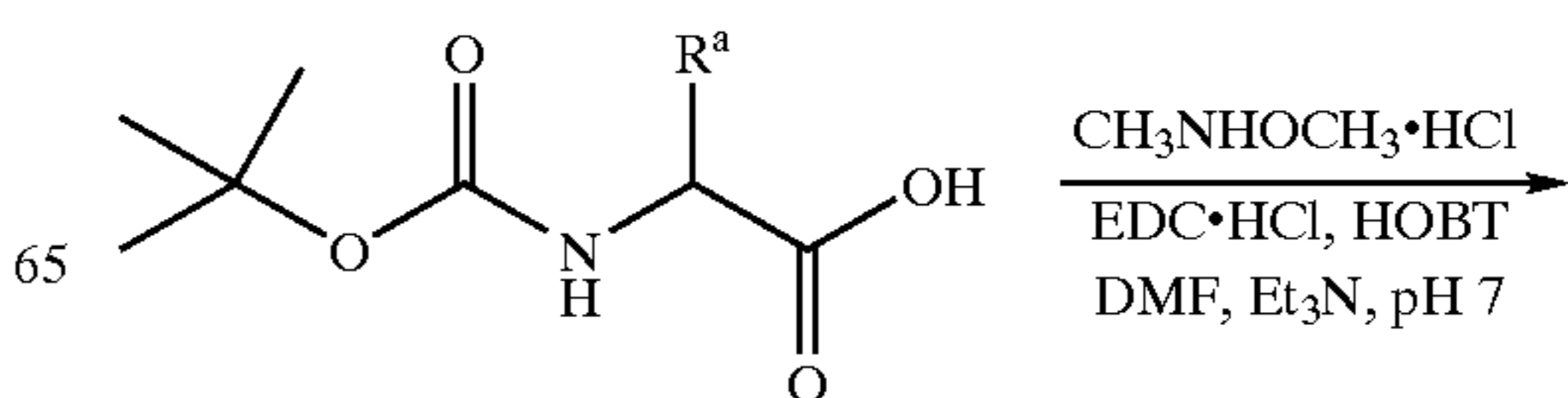
SCHEME 12
