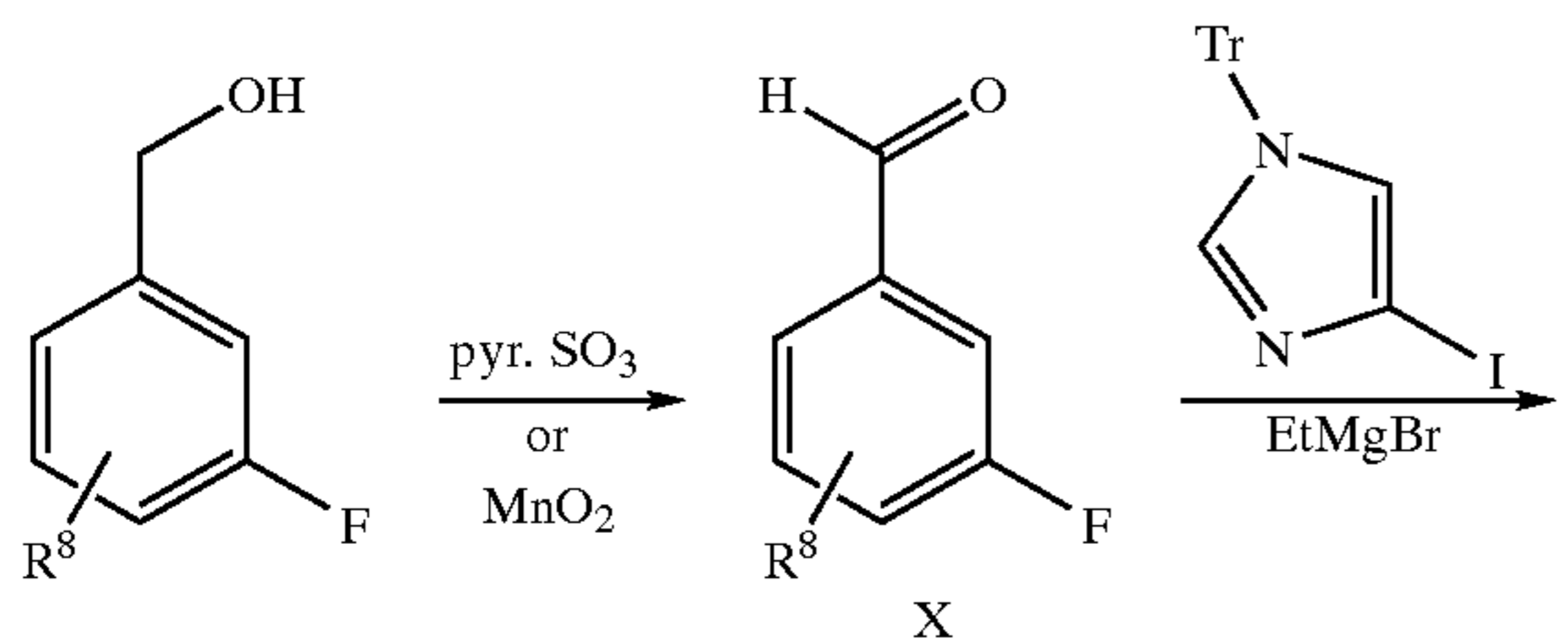
SCHEME 2
