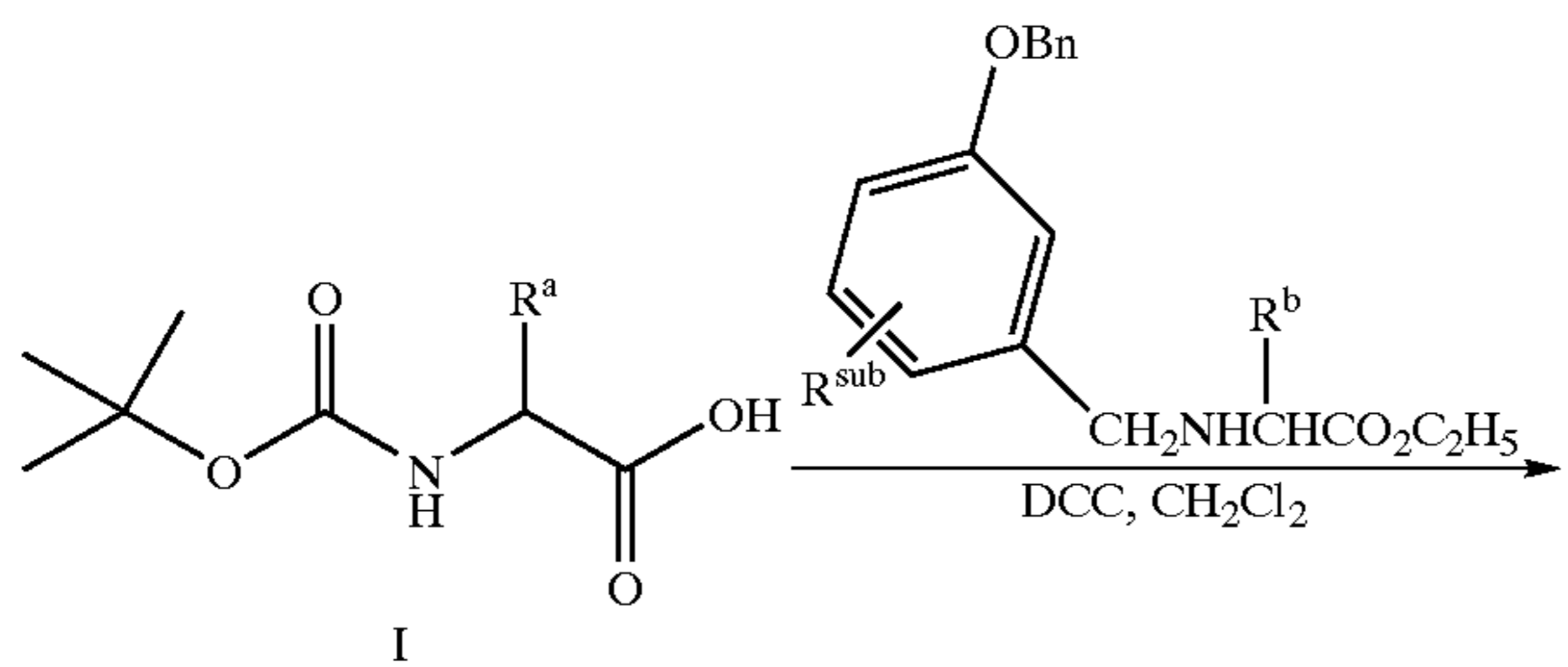
SCHEME 1
