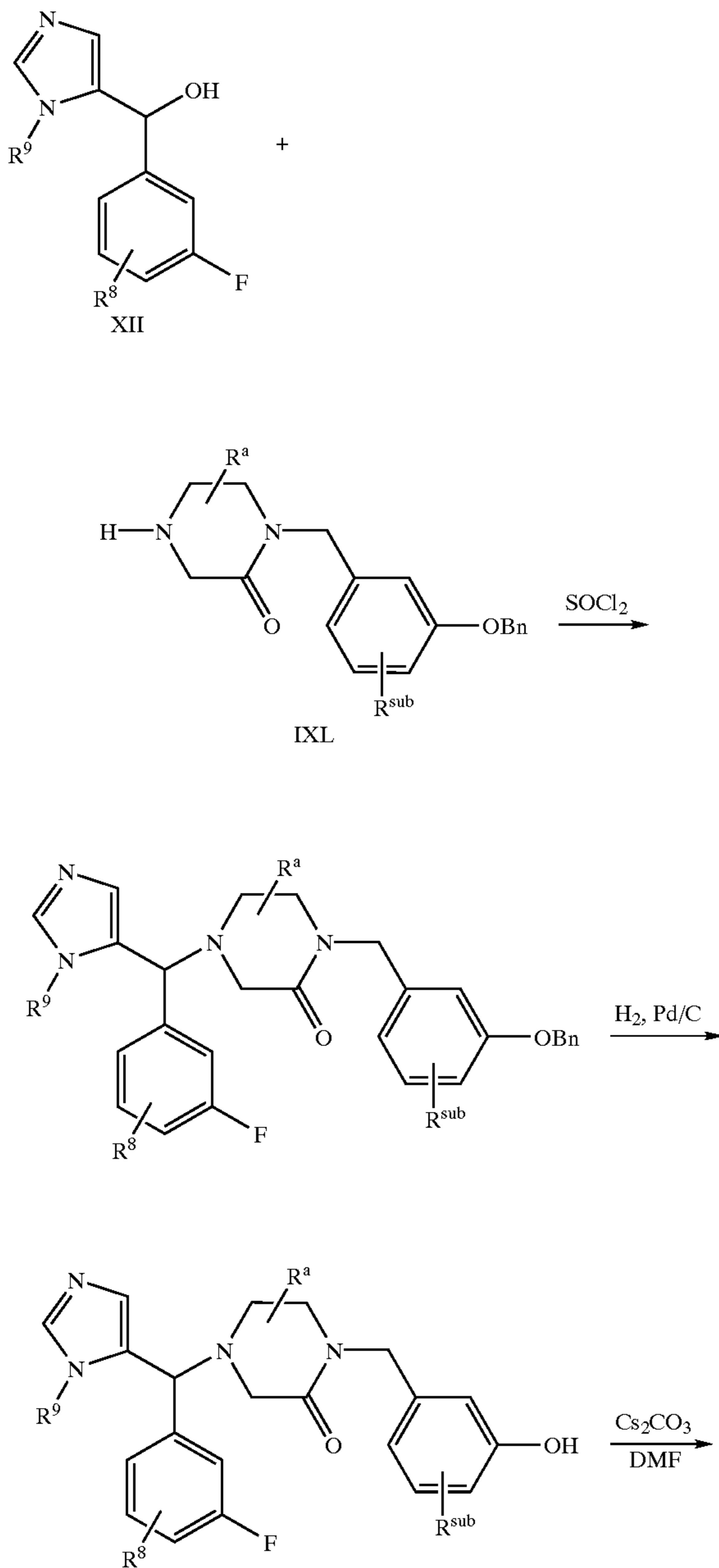
SCHEME 7
