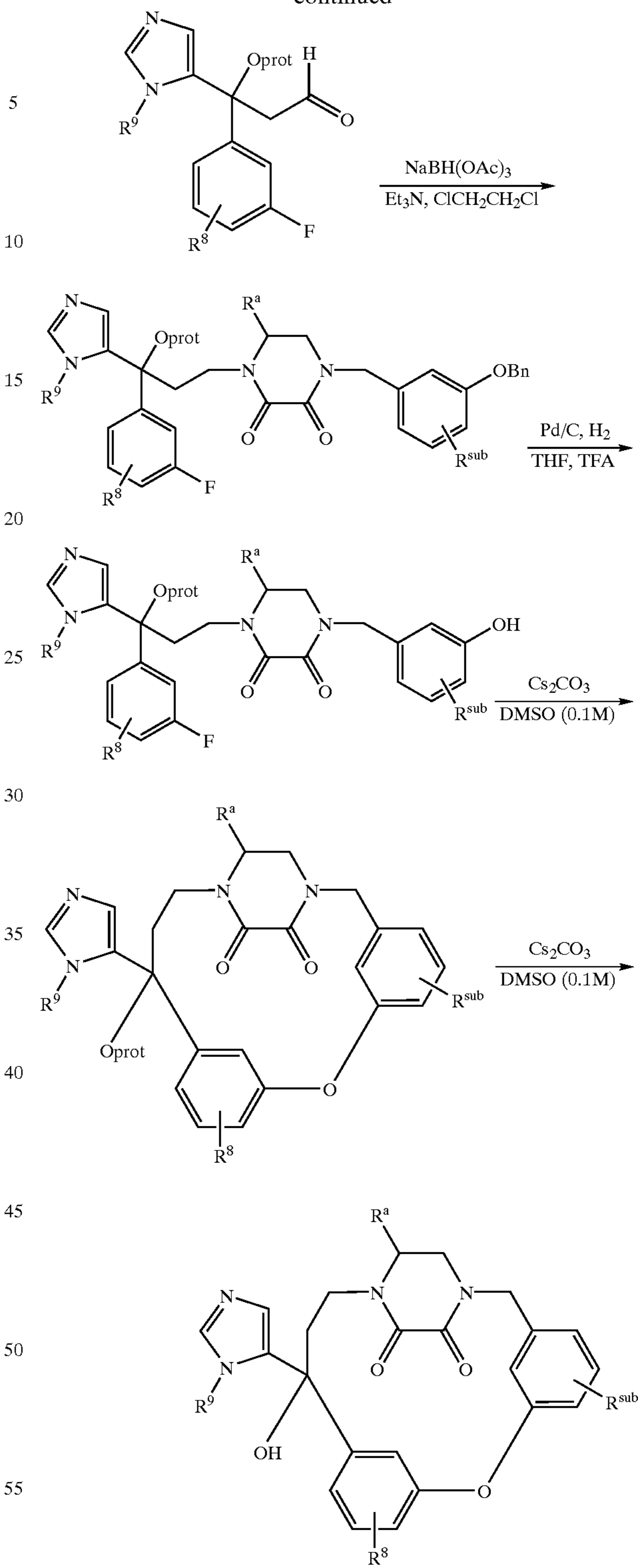
SCHEME 12
