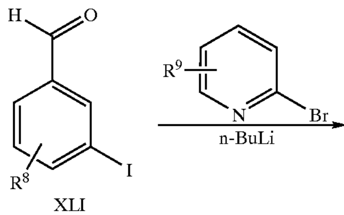
SCHEME 9
