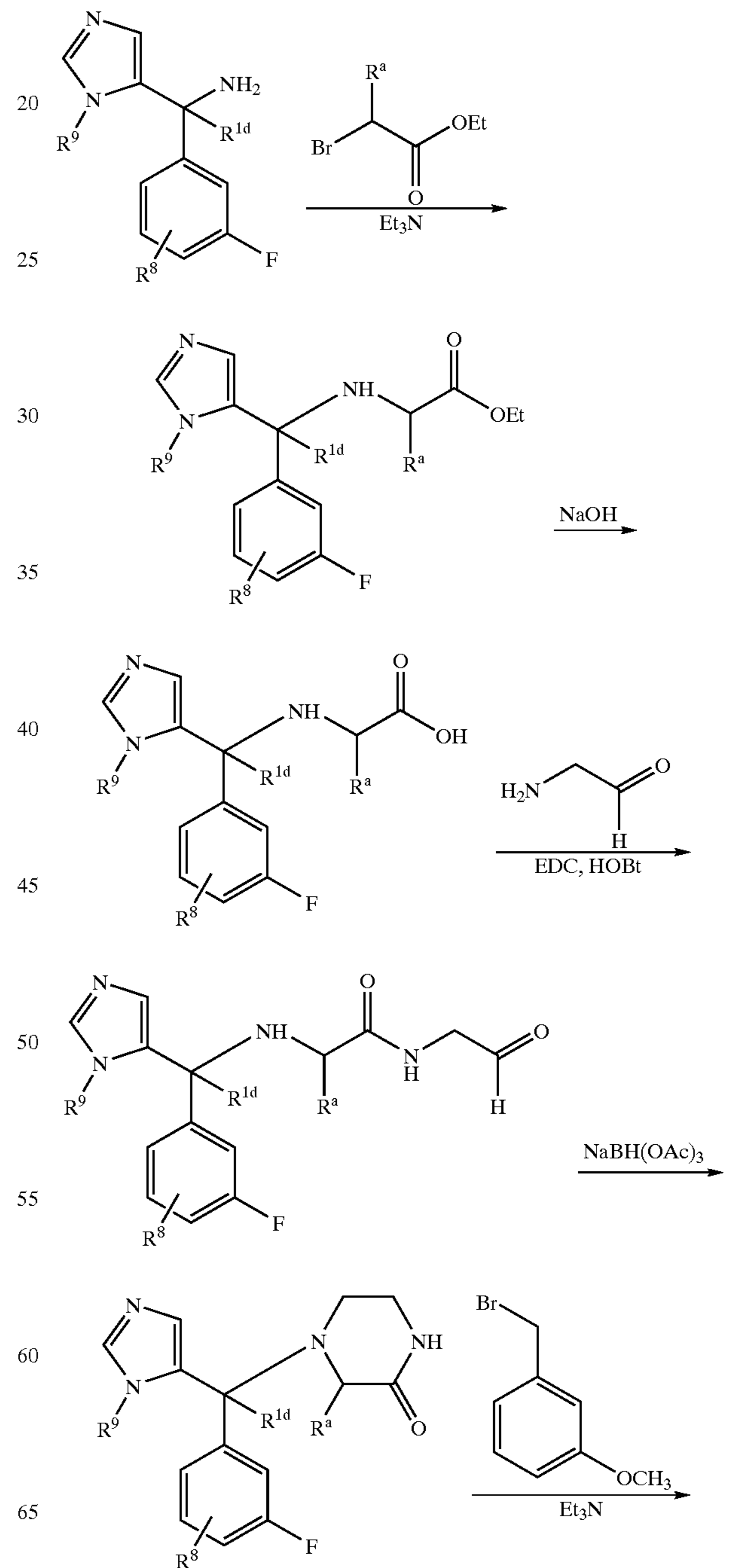
SCHEME 8
