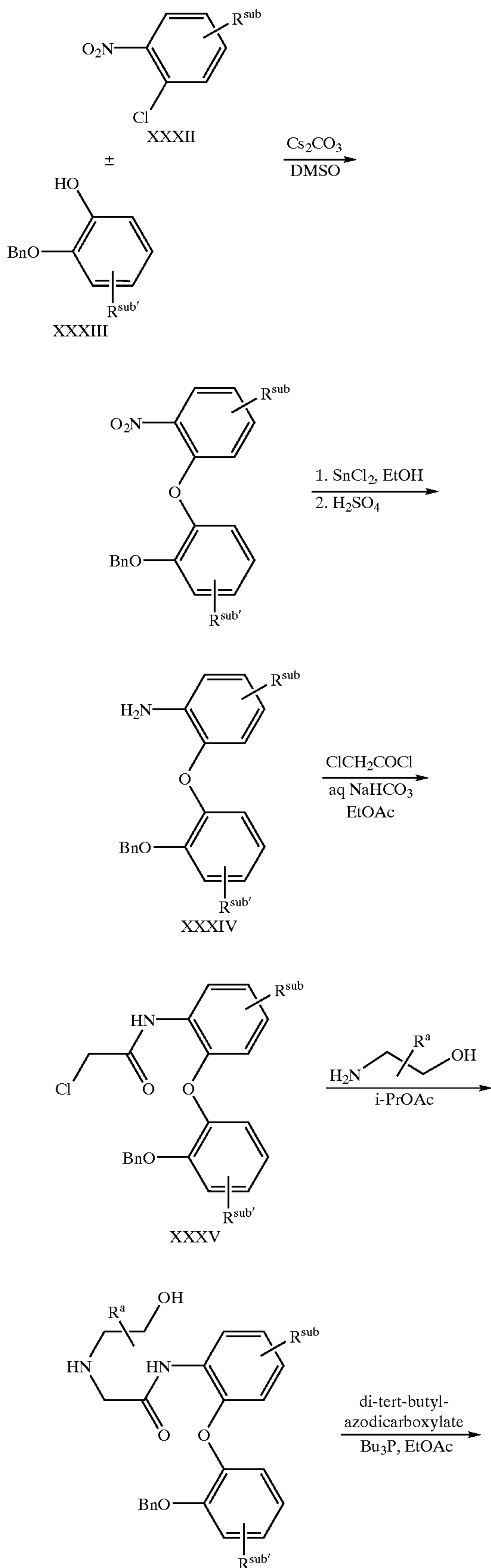
SCHEME 6
